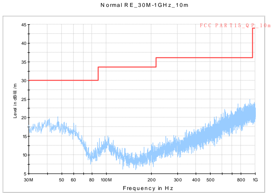
Fig. 48 Radiated Spurious Emission (802.11a, Ch157, 30 MHz-1 GHz)
