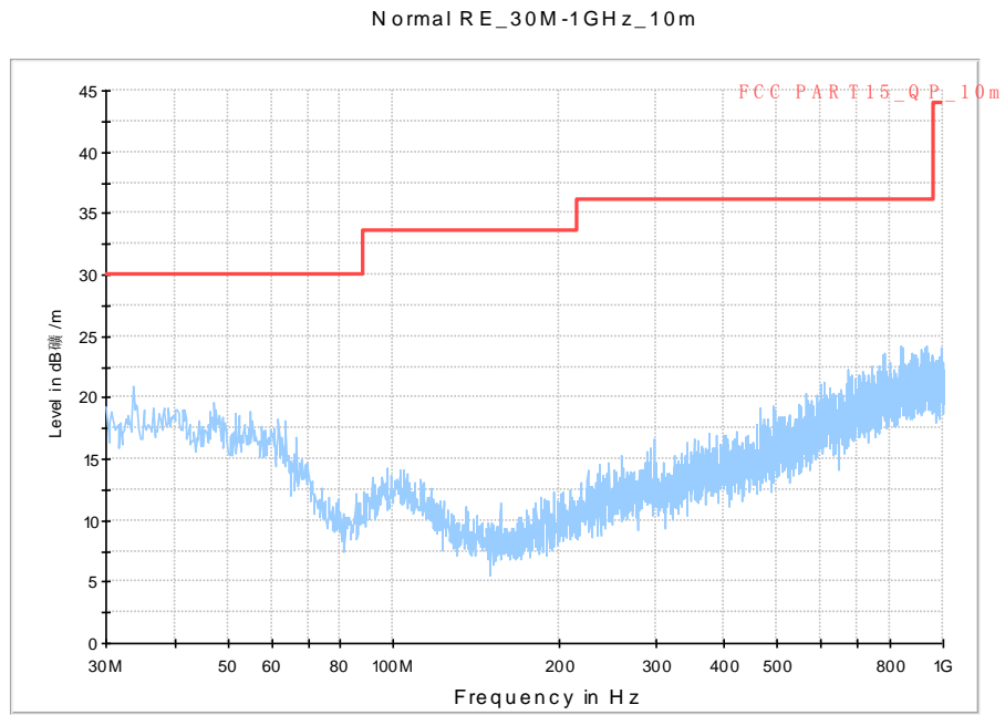
Fig. 64 Radiated Spurious Emission (802.11n-HT40, Ch151, 30 MHz-1 GHz)
