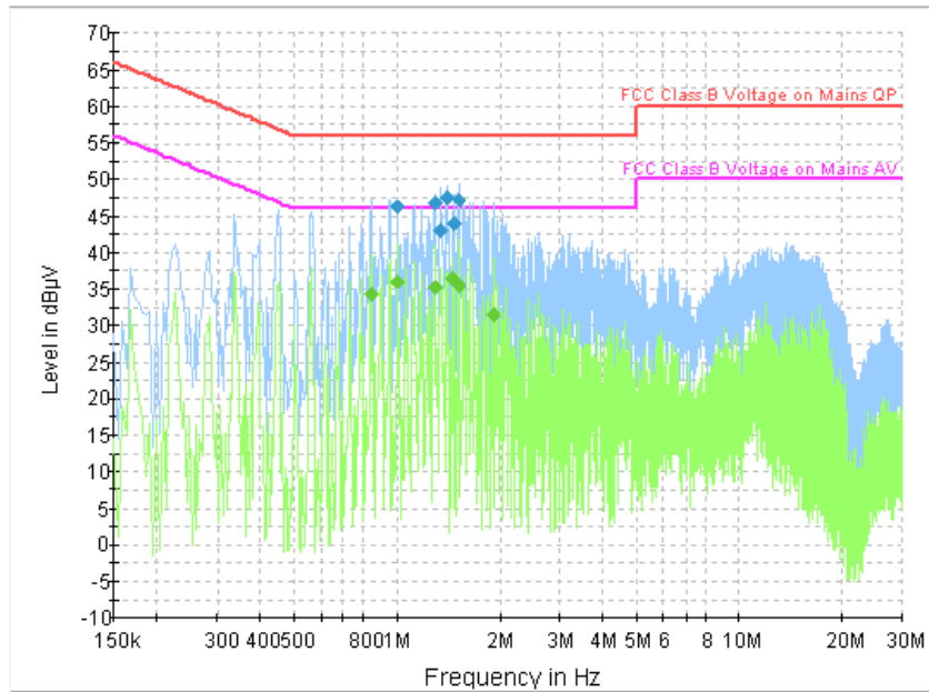
Fig. 77 AC Powerline Conducted Emission-Idle
