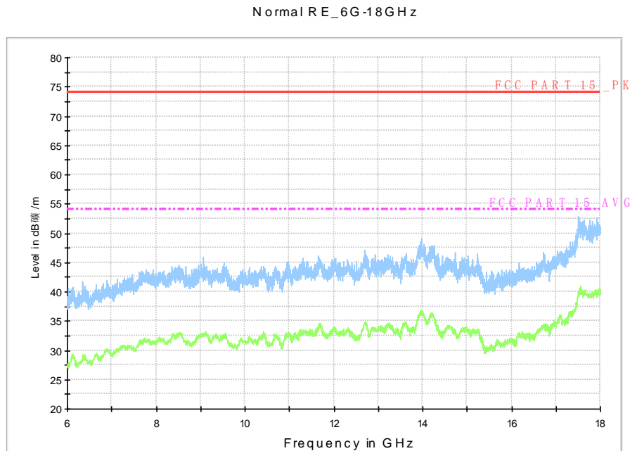
Fig. 47 Radiated Spurious Emission (802.11a, Ch149, 6 GHz-18 GHz)
