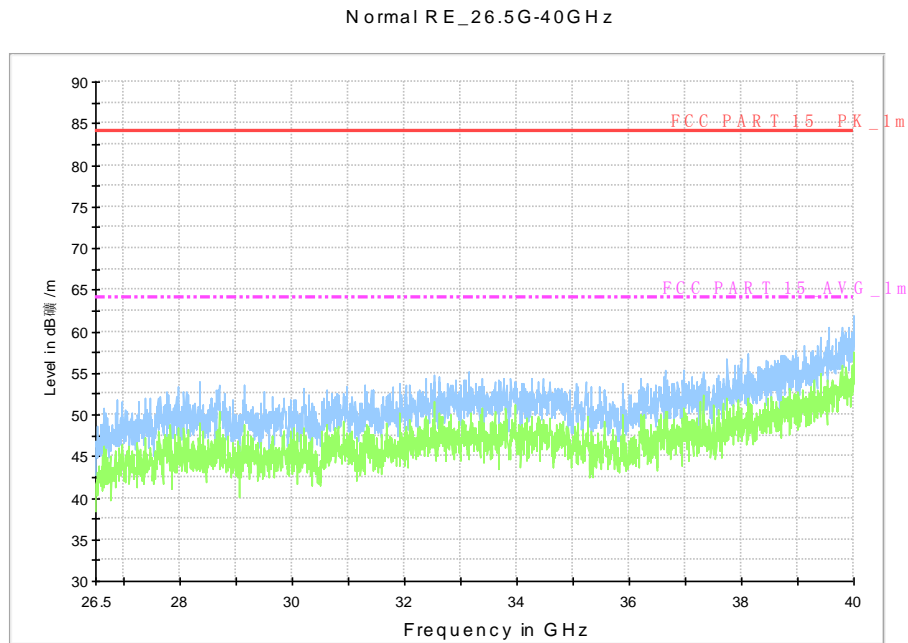
Fig. 68 Radiated emission: 802.11n, (802.11n-HT40, Ch151, 26.5 GHz - 40 GHz)
