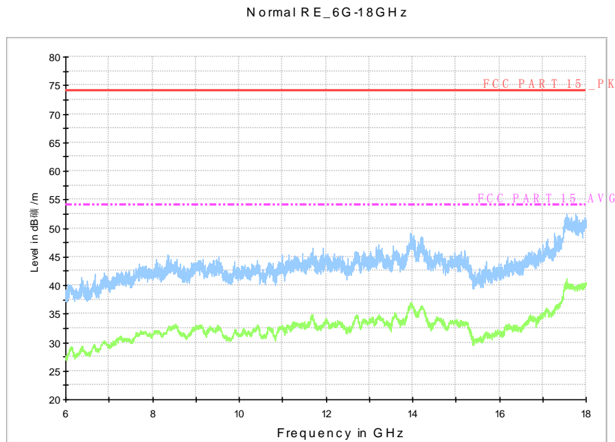
Fig. 71 Radiated Spurious Emission (802.11n-HT40, Ch159, 6 GHz-18 GHz)
