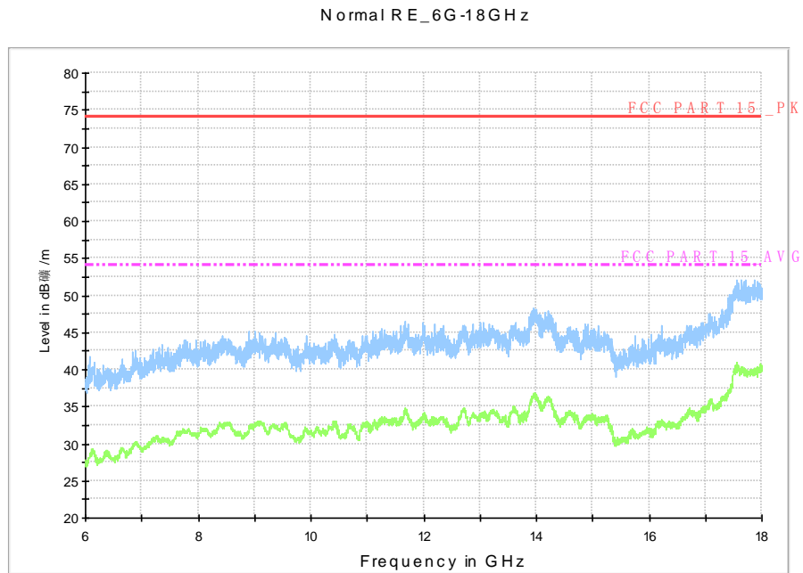
Fig. 50 Radiated Spurious Emission (802.11a, Ch157, 6 GHz-18 GHz)
