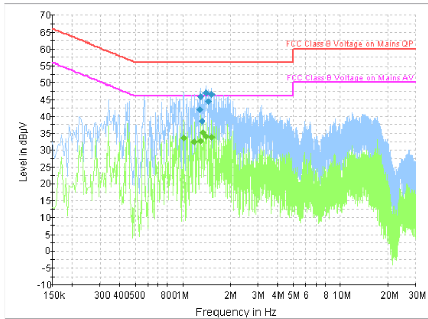
Fig. 76 AC Powerline Conducted Emission-802.11a
