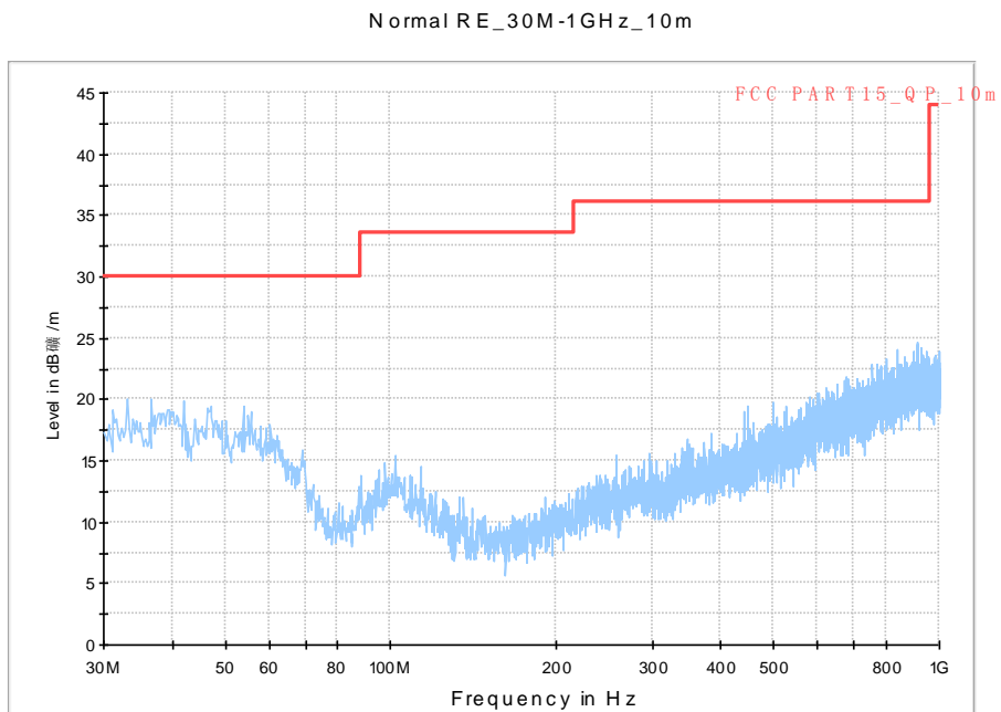
Fig. 57 Radiated Spurious Emission (802.11n-HT20, Ch157, 30 MHz-1 GHz)
