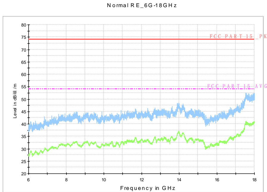
Fig. 73 Radiated Spurious Emission (802.11ac-HT80, Ch155, 6 GHz-18 GHz)
