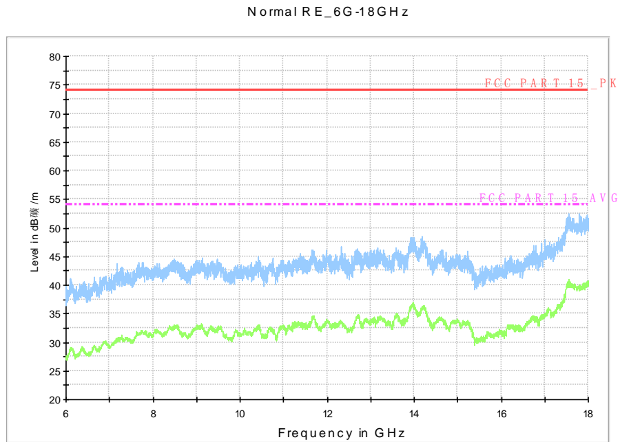
Fig. 54 Radiated Spurious Emission (802.11a, Ch165, 6 GHz-18 GHz)
