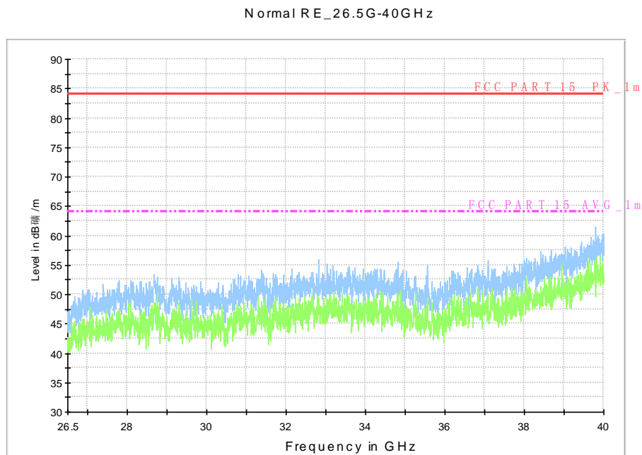
Fig. 61 Radiated emission: 802.11n, (802.11n-HT20, Ch157, 26.5 GHz - 40 GHz)
