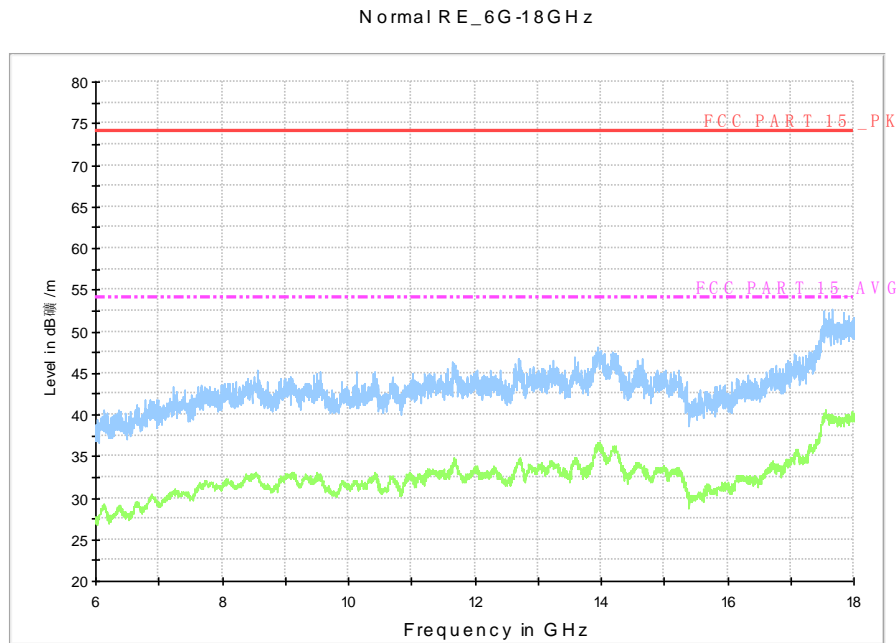
Fig. 63 Radiated Spurious Emission (802.11n-HT20, Ch165, 6 GHz-18 GHz)
