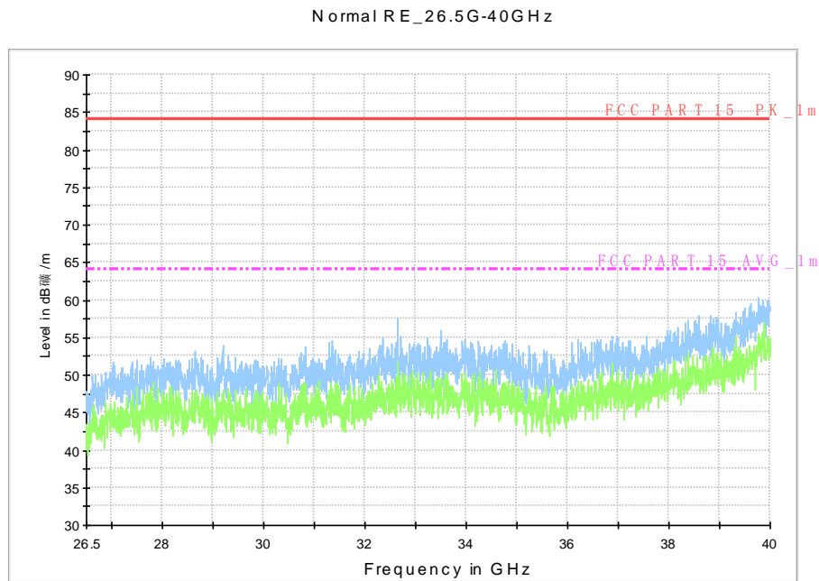
Fig. 75 Radiated emission: 802.11n, (802.11ac-HT80, Ch155, 26.5 GHz - 40 GHz)
