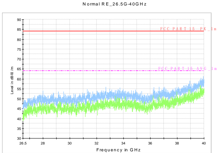
Fig. 52 Radiated emission: 802.11n, (802.11a, Ch157, 26.5 GHz - 40 GHz)
