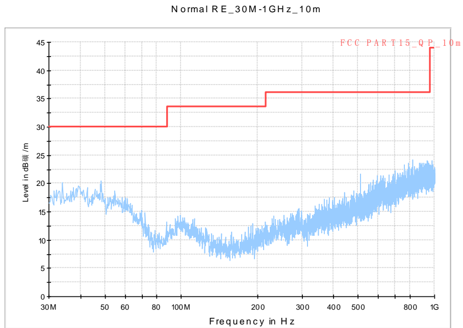
Fig. 69 Radiated Spurious Emission (802.11n-HT40, Ch159, 30 MHz-1 GHz)
