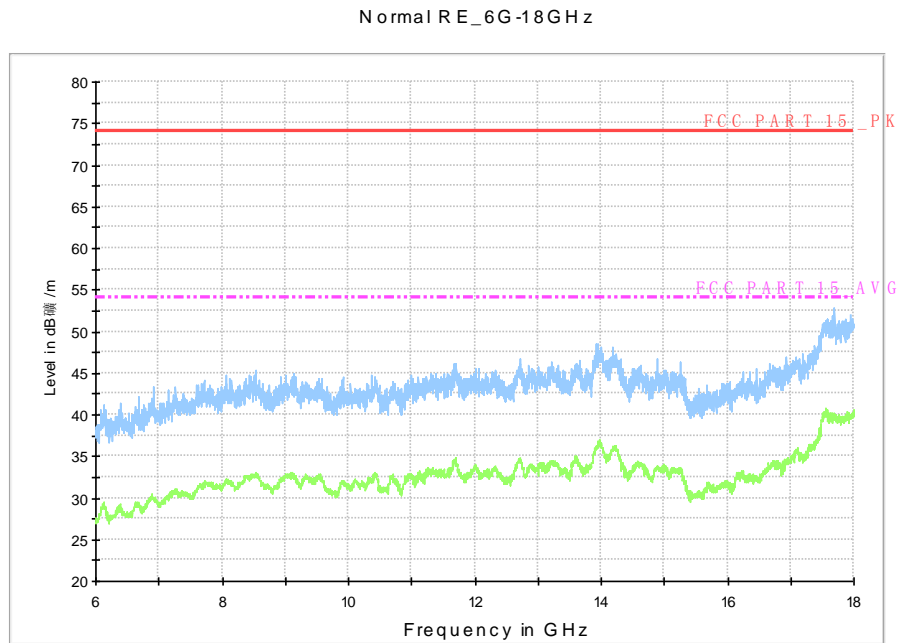
Fig. 66 Radiated Spurious Emission (802.11n-HT40, Ch151, 6 GHz-18 GHz)
