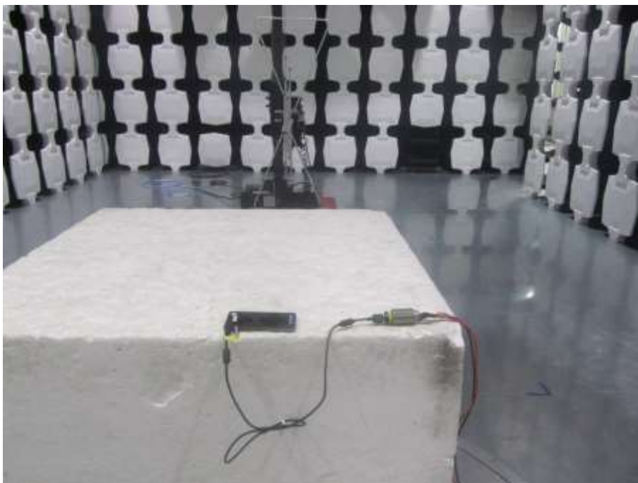
GPS Radiated emission
