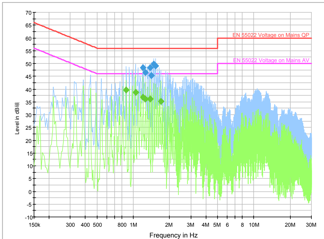
Fig.18 AC Powerline Conducted Emission with charger-TX Mode
