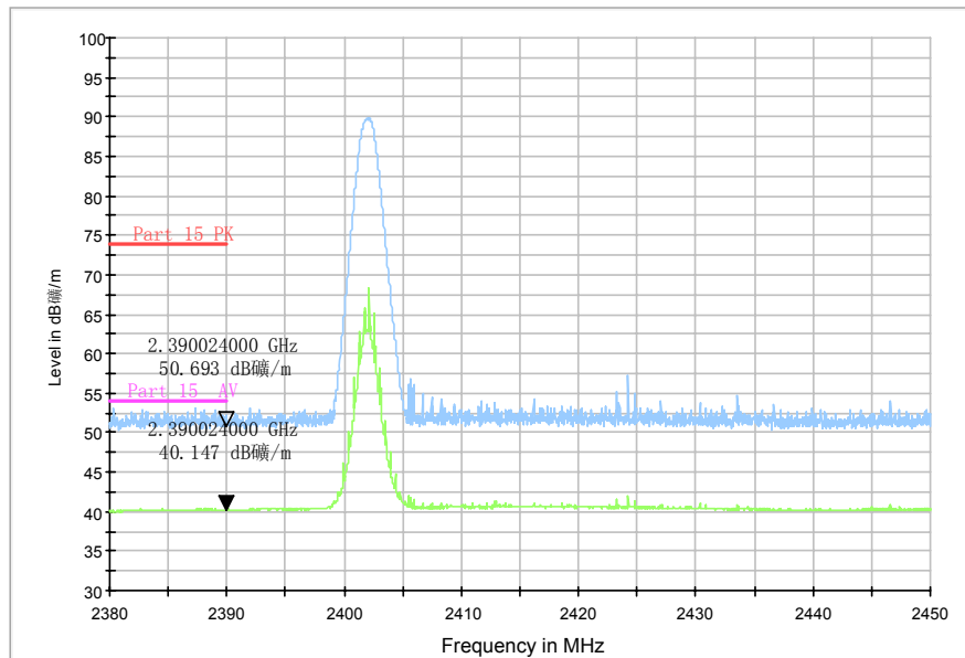
RE - Power-2.38GHz-2.45GHz
