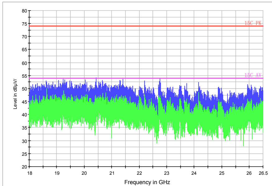
18G-26.5G RE
