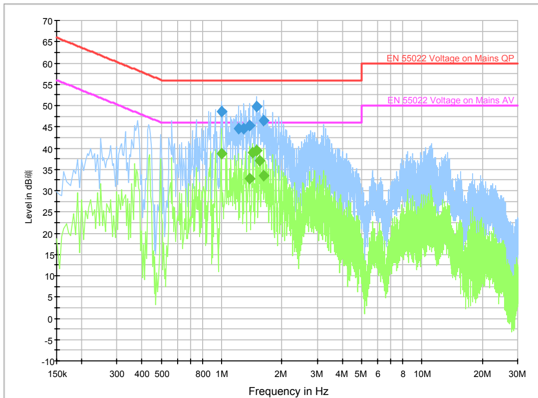
Fig.19 AC Powerline Conducted Emission with charger-Idle Mode
