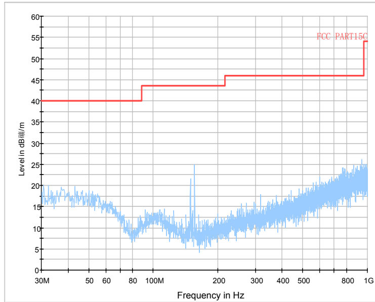
RE_30M-1GHz_3m
