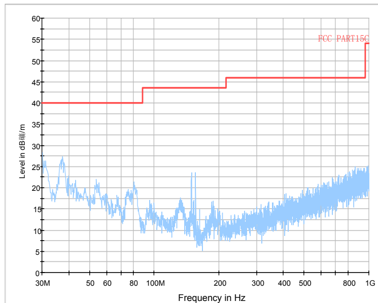
RE_30M-1GHz_3m
