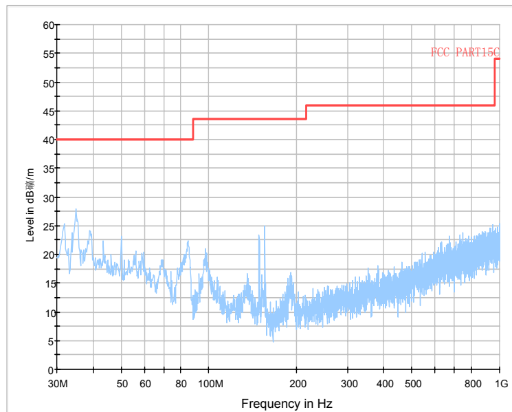
RE_30M-1GHz_3m
