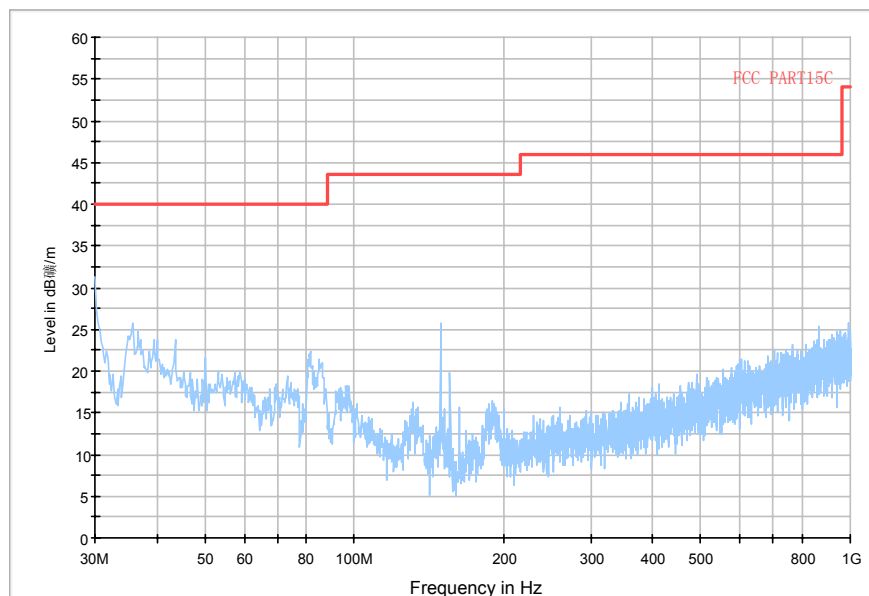
RE_30M-1GHz_3m
