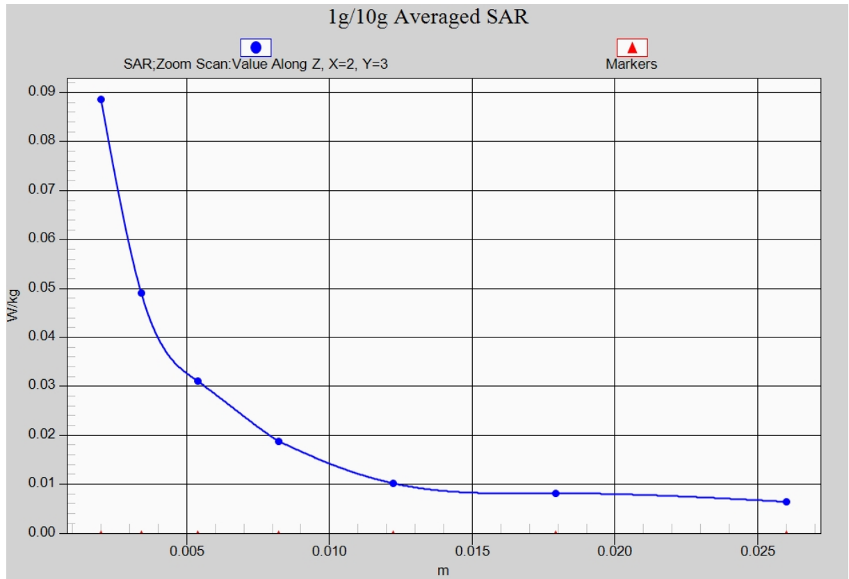
Fig. 14-1 Z-Scan at power reference point (5GHz CH36)
