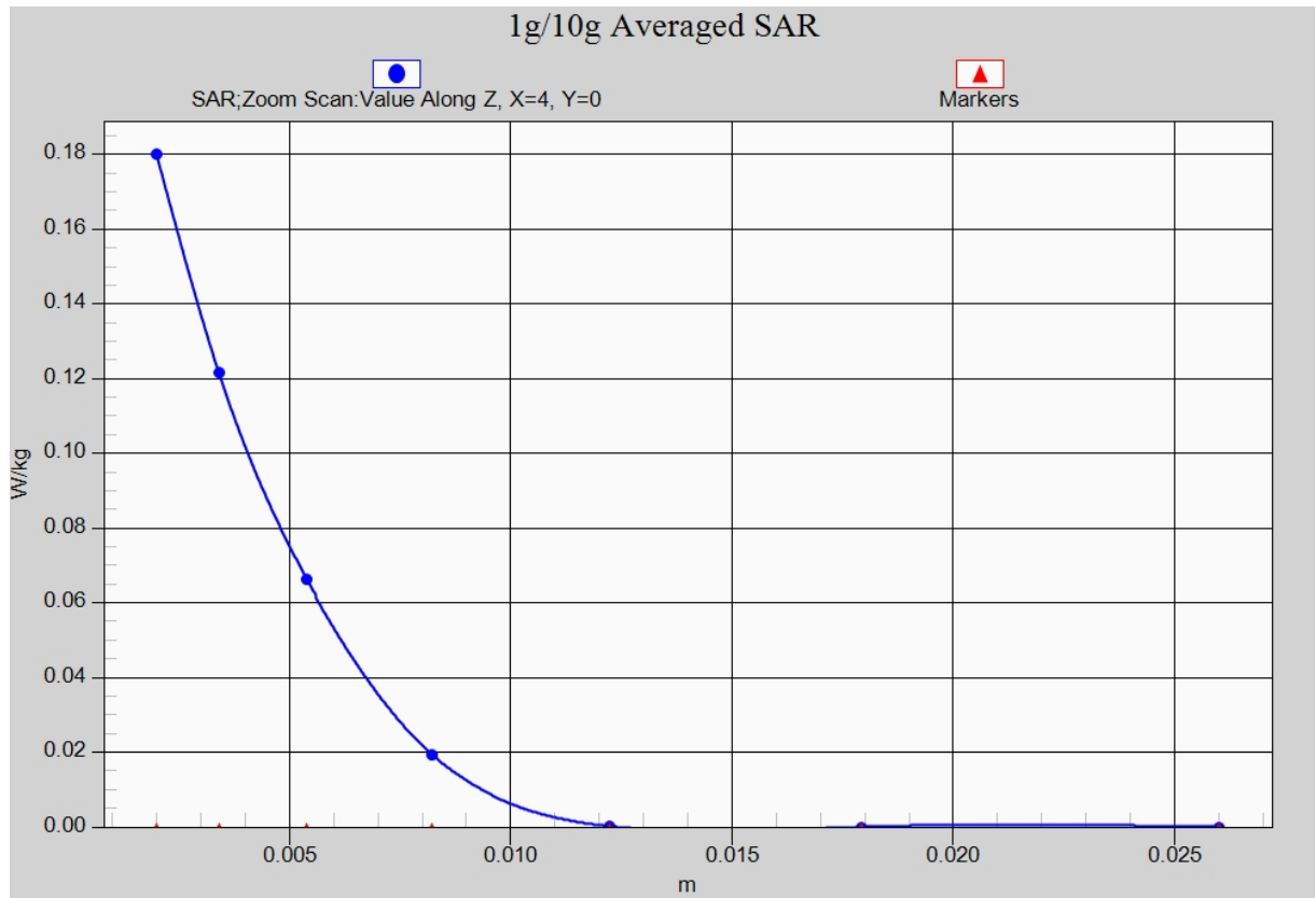
Fig. 9-1 Z-Scan at power reference point (5GHz CH36)
