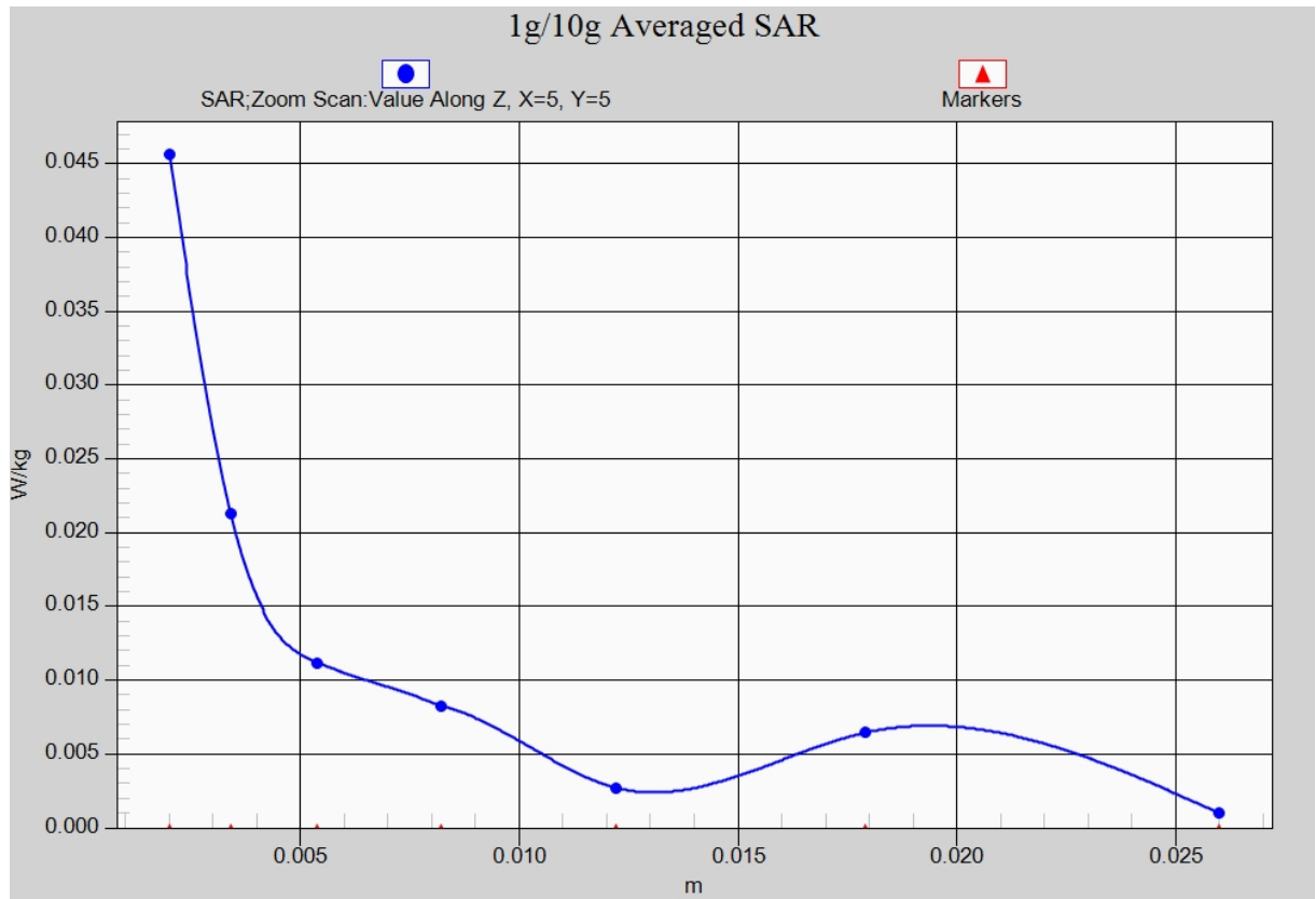
Fig. 10-1 Z-Scan at power reference point (5GHz CH36)
