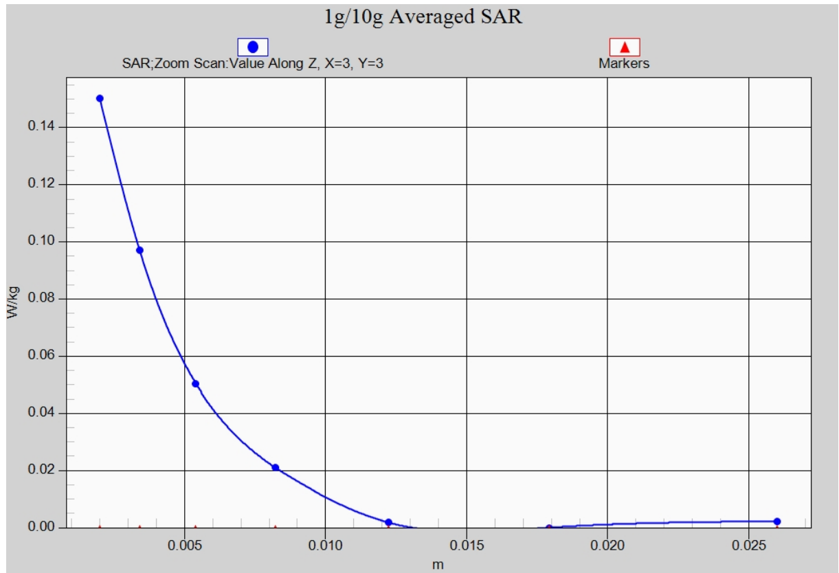
Fig. 13-1 Z-Scan at power reference point (5GHz CH36)
