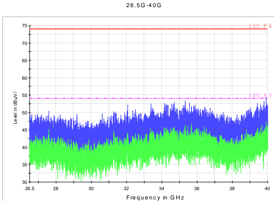
Fig. 82 Radiated Spurious Emission (802.11a, ch56, 26.5 GHz-40 GHz)
