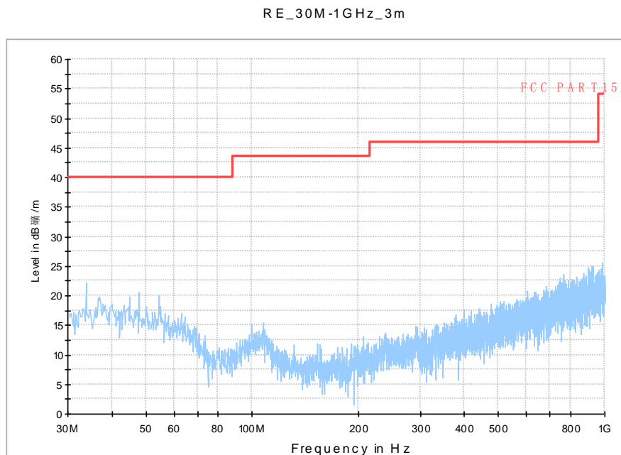
Fig. 59 Radiated Spurious Emission (802.11a, ch40, 30 MHz-1 GHz)
