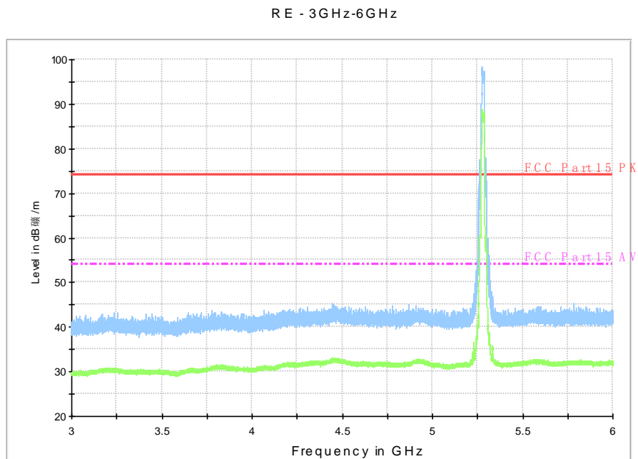
Fig. 79 Radiated Spurious Emission (802.11a, ch56, 3 GHz-6 GHz)
