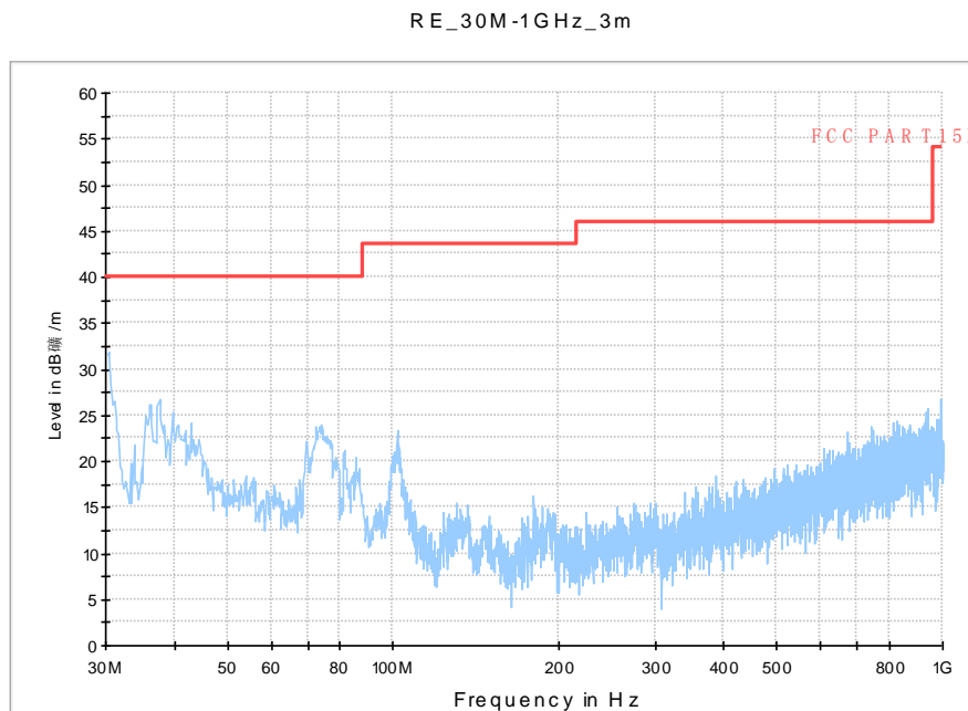
Fig. 101 Radiated Spurious Emission (802.11a, ch140, 30 MHz-1 GHz)
