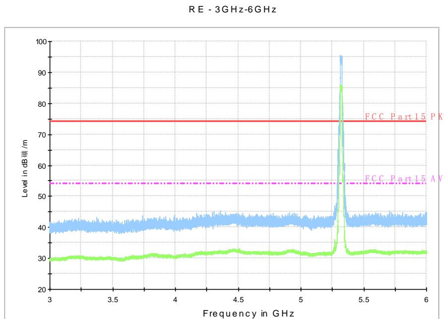
Fig. 85 Radiated Spurious Emission (802.11a, ch64, 3 GHz-6 GHz)
