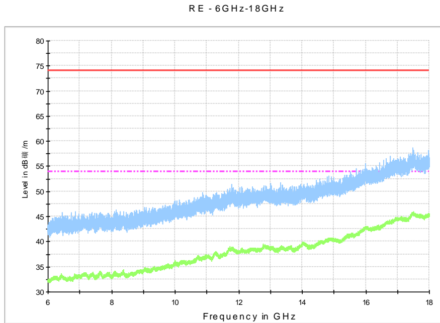
Fig. 86 Radiated Spurious Emission (802.11a, ch64, 6 GHz-18 GHz)
