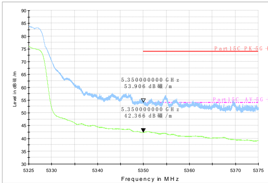
RE - Power-5.325GHz-5.375GHz
