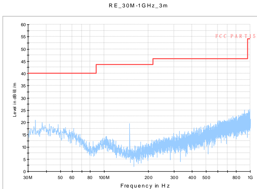
Fig. 113 Radiated Spurious Emission (802.11a, ch40, 30 MHz-1 GHz)
