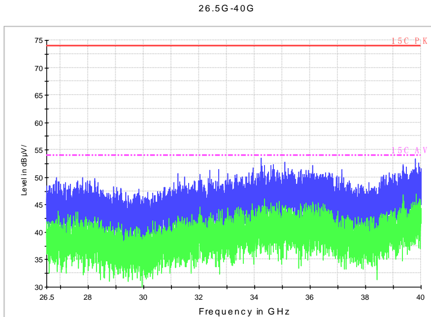
Fig. 76 Radiated Spurious Emission (802.11a, ch52, 26.5 GHz-40 GHz)
