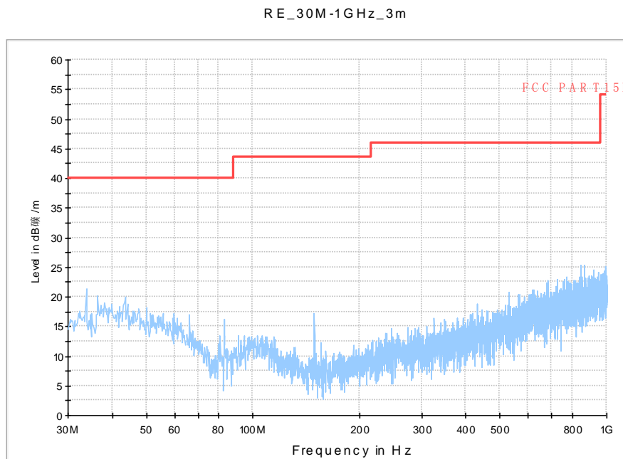
Fig. 107 Radiated Spurious Emission (802.11n-HT20, ch36, 30 MHz-1 GHz)
