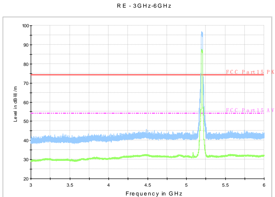
Fig. 61 Radiated Spurious Emission (802.11a, ch40, 3 GHz-6 GHz)
