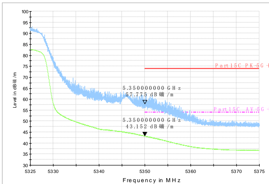
RE - Power-5.325GHz-5.375GHz
