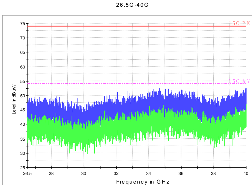
Fig. 88 Radiated Spurious Emission (802.11a, ch64, 26.5 GHz-40 GHz)
