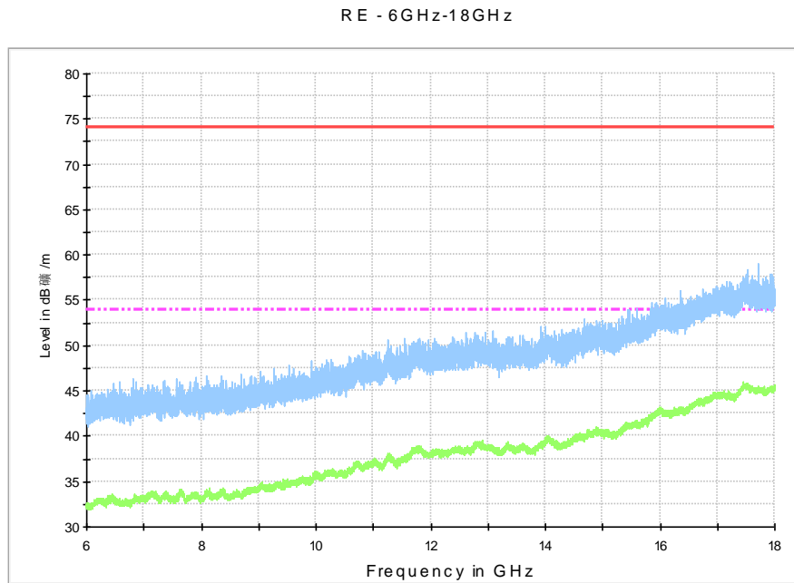
Fig. 104 Radiated Spurious Emission (802.11a, ch140, 6 GHz-18 GHz)
