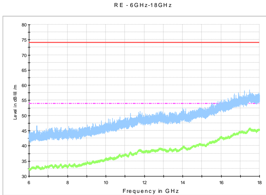
Fig. 92 Radiated Spurious Emission (802.11a, ch100, 6 GHz-18 GHz)
