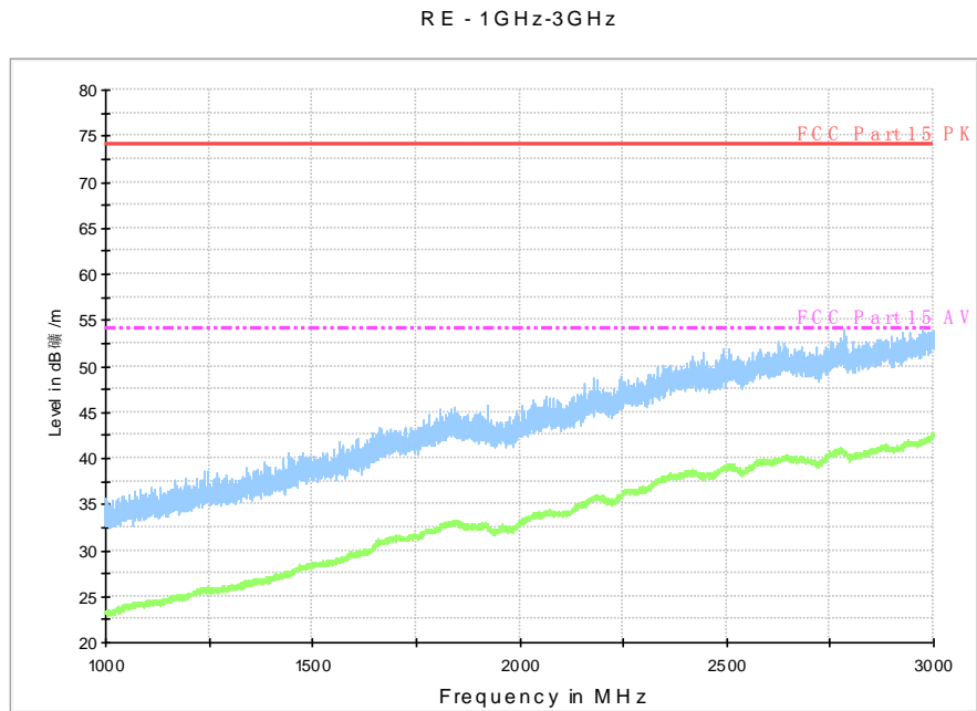
Fig. 66 Radiated Spurious Emission (802.11a, ch48, 1 GHz-3 GHz)
