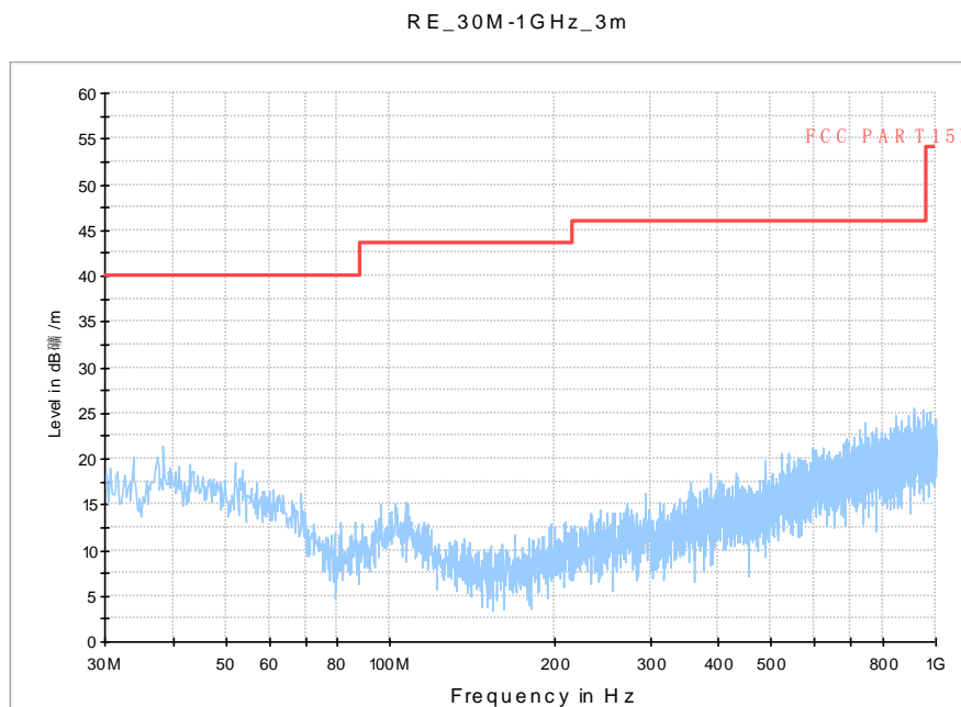
Fig. 89 Radiated Spurious Emission (802.11a, ch100, 30 MHz-1 GHz)
