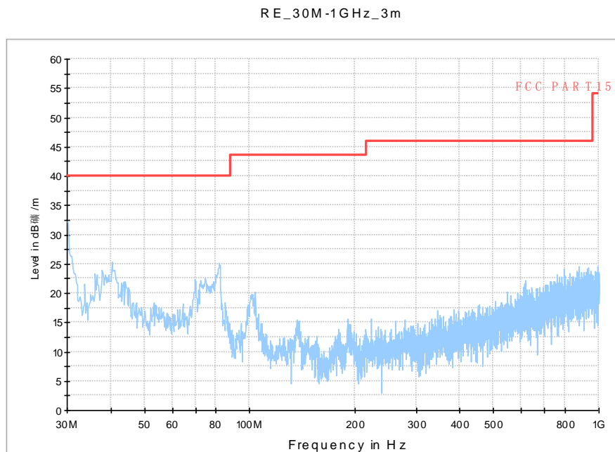
Fig. 71 Radiated Spurious Emission (802.11a, ch52, 30 MHz-1 GHz)
