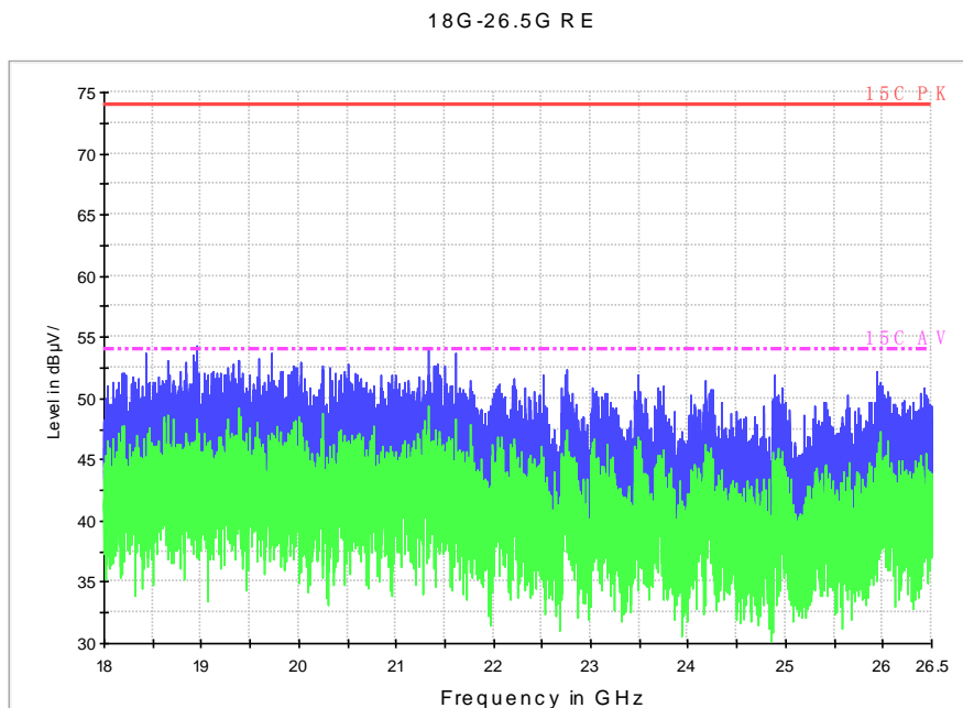
Fig. 63 Radiated Spurious Emission (802.11a, ch40, 18 GHz-26.5 GHz)
