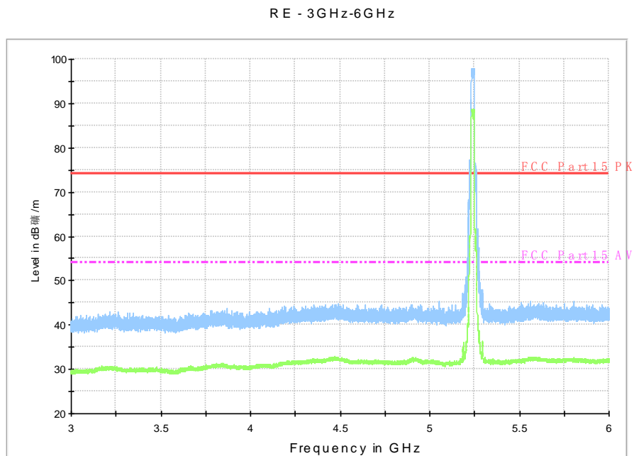
Fig. 67 Radiated Spurious Emission (802.11a, ch48, 3 GHz-6 GHz)
