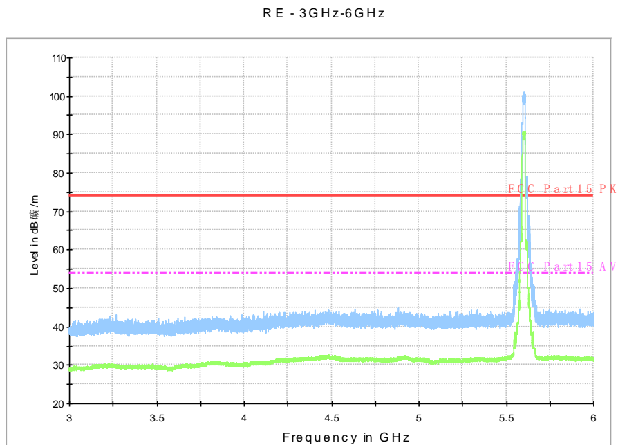
Fig. 97 Radiated Spurious Emission (802.11a, ch120, 3 GHz-6 GHz)
