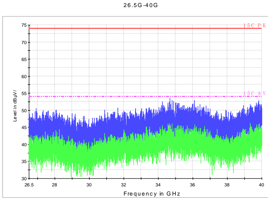
Fig. 106 Radiated Spurious Emission (802.11a, ch140, 26.5 GHz-40 GHz)
