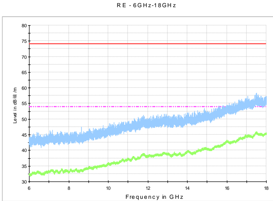
Fig. 56 Radiated Spurious Emission (802.11a, ch36, 6 GHz-18 GHz)
