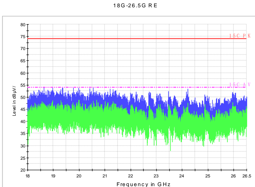
Fig. 117 Radiated Spurious Emission (802.11a, ch40, 18 GHz-26.5 GHz)
