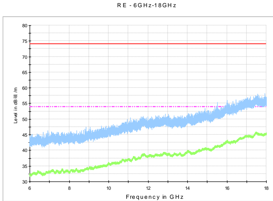
Fig. 62 Radiated Spurious Emission (802.11a, ch40, 6 GHz-18 GHz)
