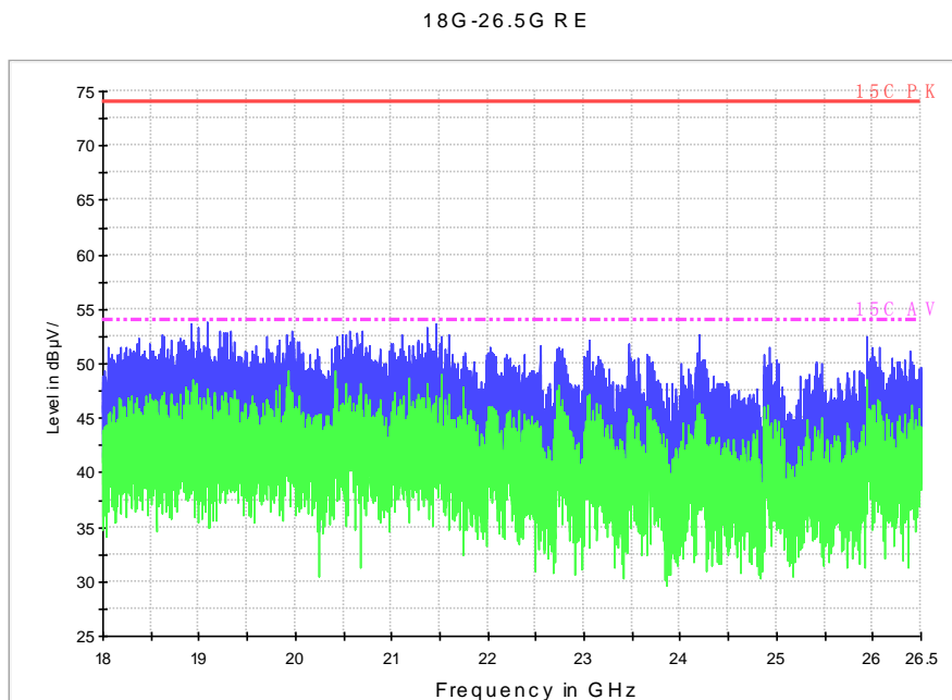
Fig. 87 Radiated Spurious Emission (802.11a, ch64, 18 GHz-26.5 GHz)
