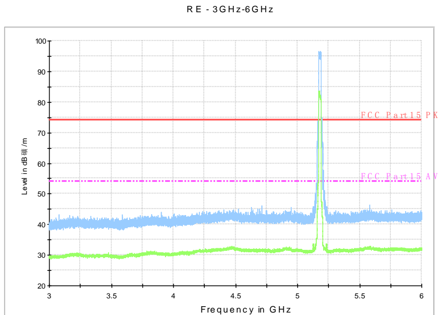
Fig. 55 Radiated Spurious Emission (802.11a, ch36, 3 GHz-6 GHz)
