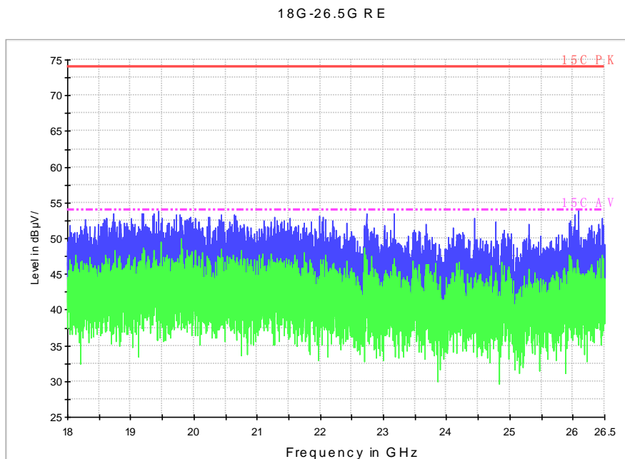
Fig. 81 Radiated Spurious Emission (802.11a, ch56, 18 GHz-26.5 GHz)
