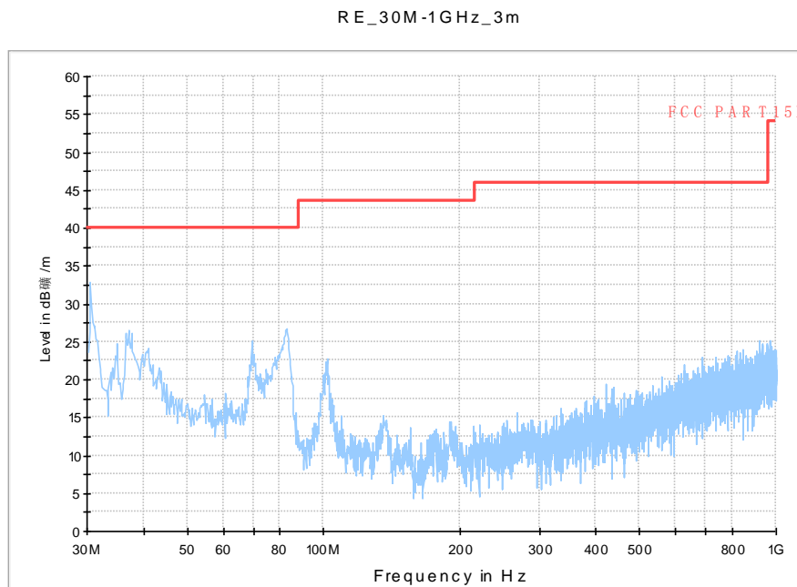
Fig. 83 Radiated Spurious Emission (802.11a, ch64, 30 MHz-1 GHz)
