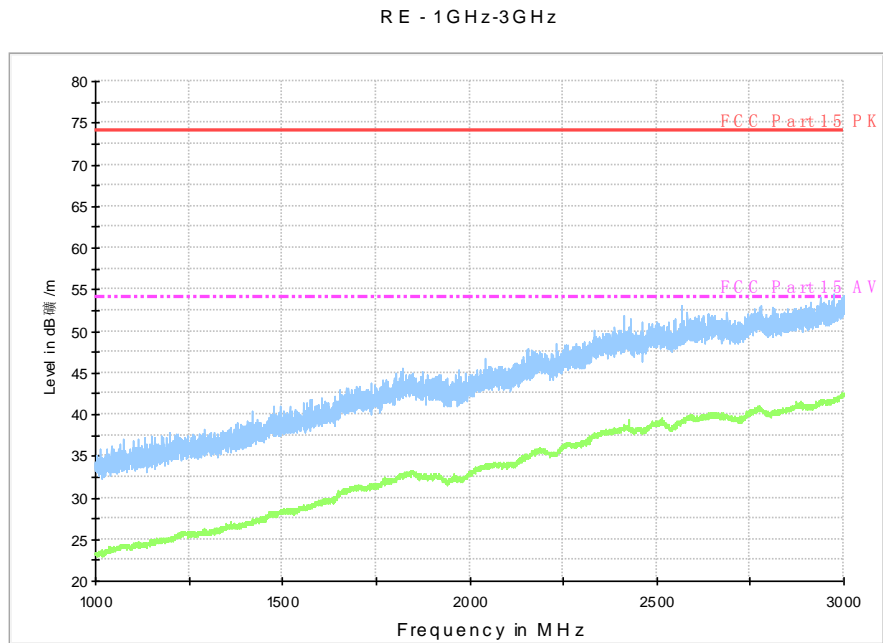
Fig. 84 Radiated Spurious Emission (802.11a, ch64, 1 GHz-3 GHz)
