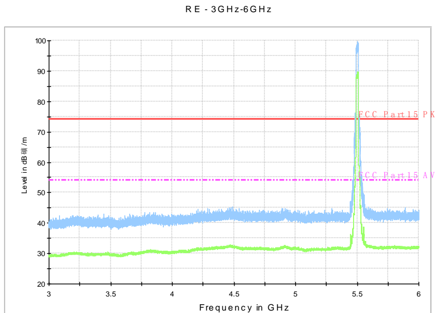
Fig. 91 Radiated Spurious Emission (802.11a, ch100, 3 GHz-6 GHz)
