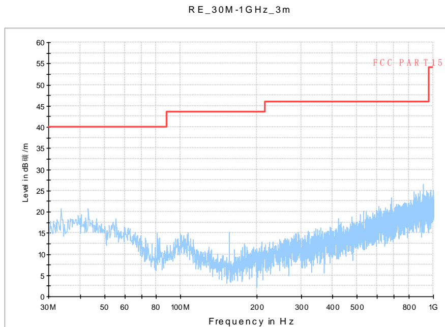
Fig. 65 Radiated Spurious Emission (802.11a, ch48, 30 MHz-1 GHz)
