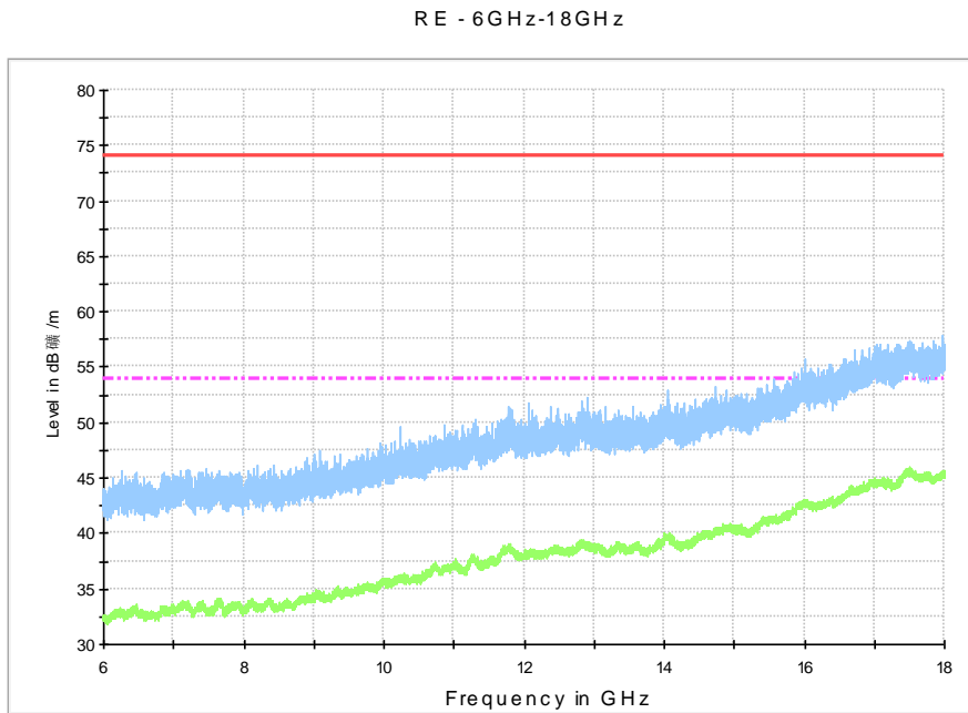
Fig. 98 Radiated Spurious Emission (802.11a, ch120, 6 GHz-18 GHz)
