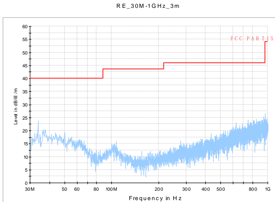
Fig. 95 Radiated Spurious Emission (802.11a, ch120, 30 MHz-1 GHz)
