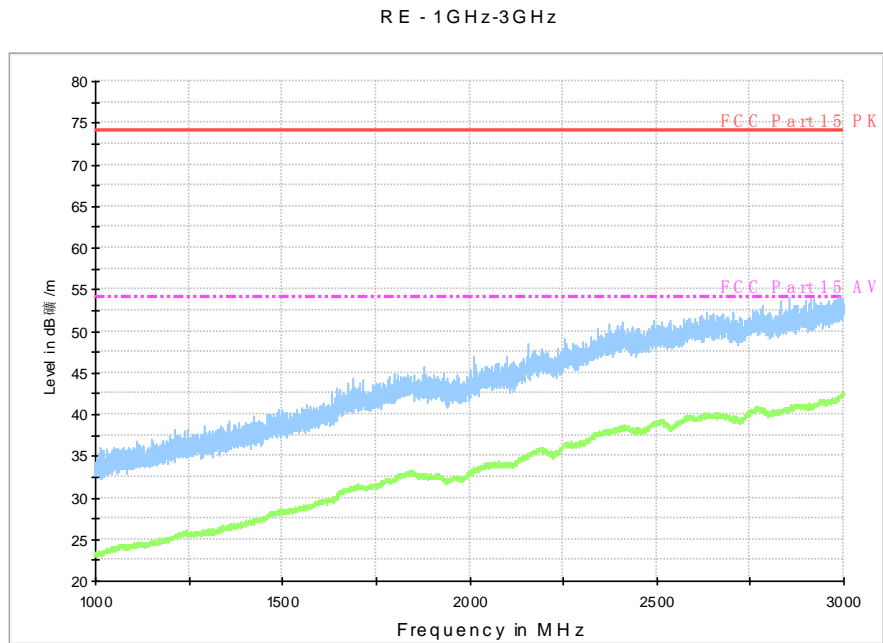
Fig. 78 Radiated Spurious Emission (802.11a, ch56, 1 GHz-3 GHz)
