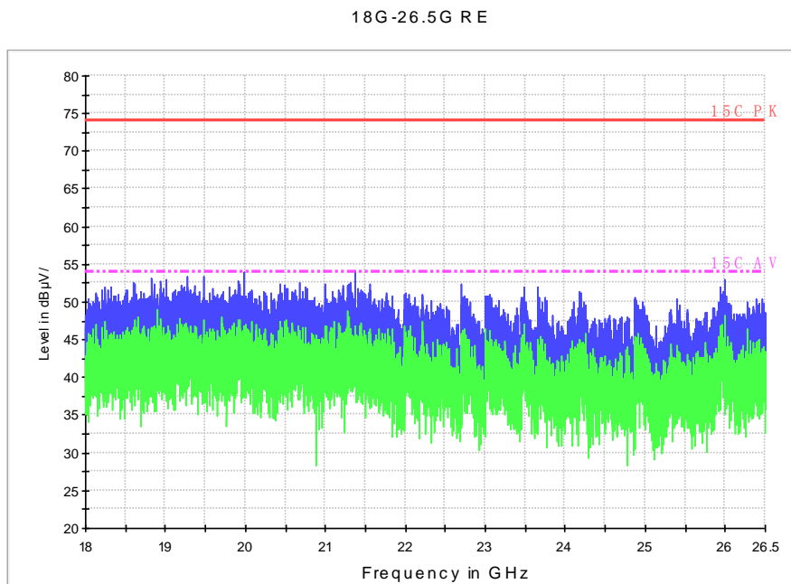
Fig. 93 Radiated Spurious Emission (802.11a, ch100, 18 GHz-26.5 GHz)
