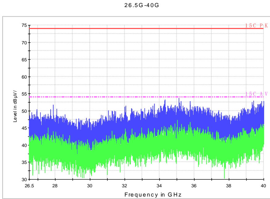
Fig. 94 Radiated Spurious Emission (802.11a, ch100, 26.5 GHz-40 GHz)
