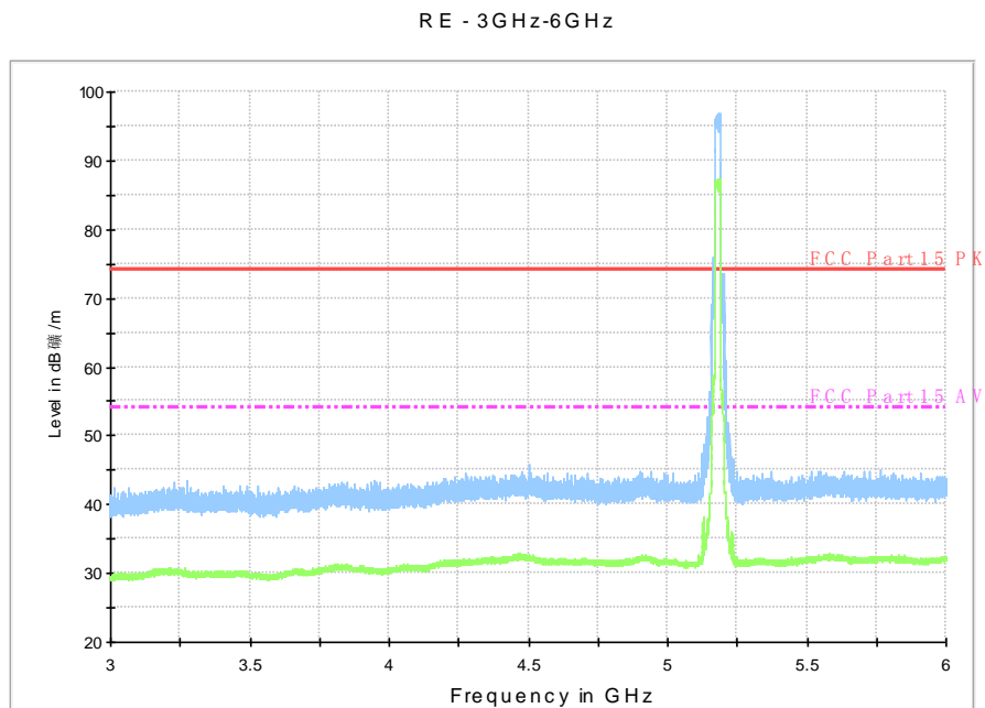
Fig. 109 Radiated Spurious Emission (802.11n-HT20, ch36, 3 GHz-6 GHz)
