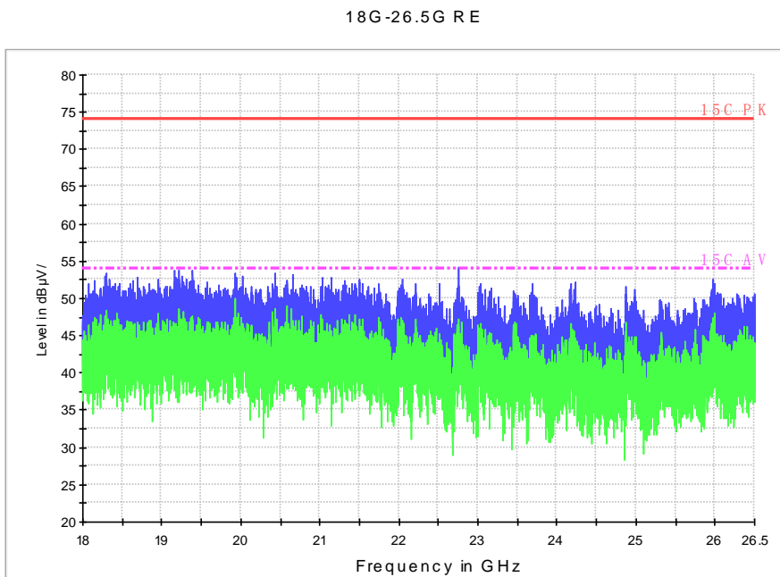
Fig. 111 Radiated Spurious Emission (802.11n-HT20, ch36, 18 GHz-26.5 GHz)
