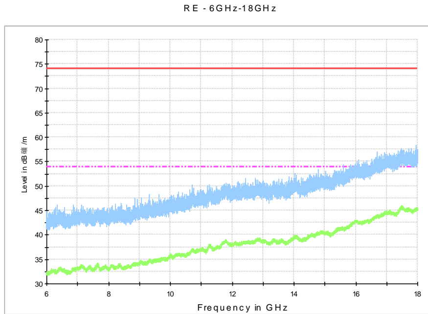
Fig. 116 Radiated Spurious Emission (802.11a, ch40, 6 GHz-18 GHz)
