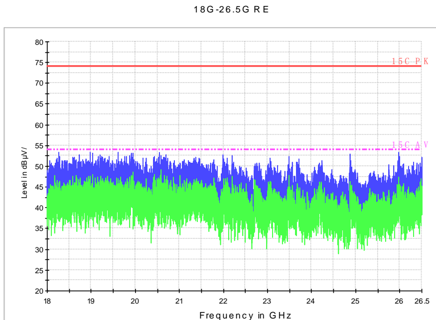
Fig. 105 Radiated Spurious Emission (802.11a, ch140, 18 GHz-26.5 GHz)
