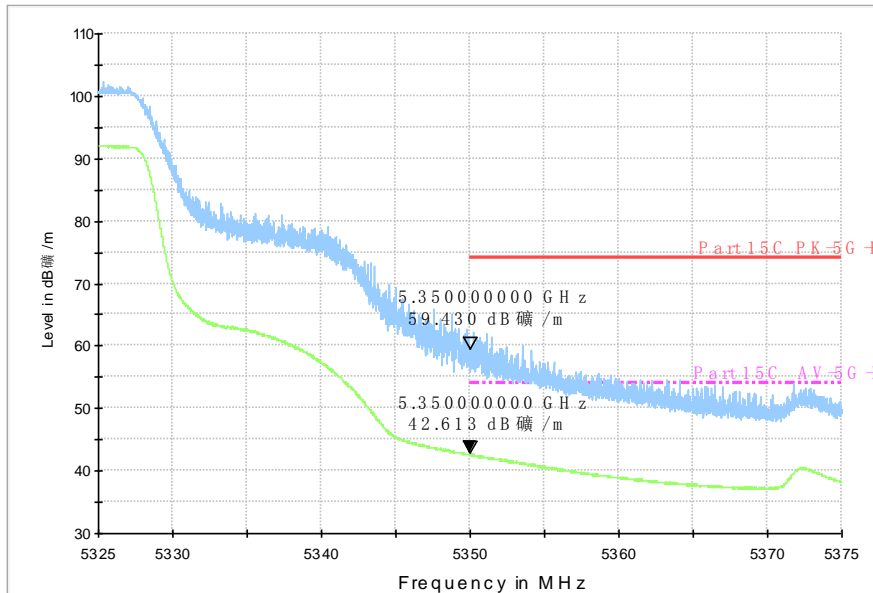
RE - Power-5.325GHz-5.375GHz
