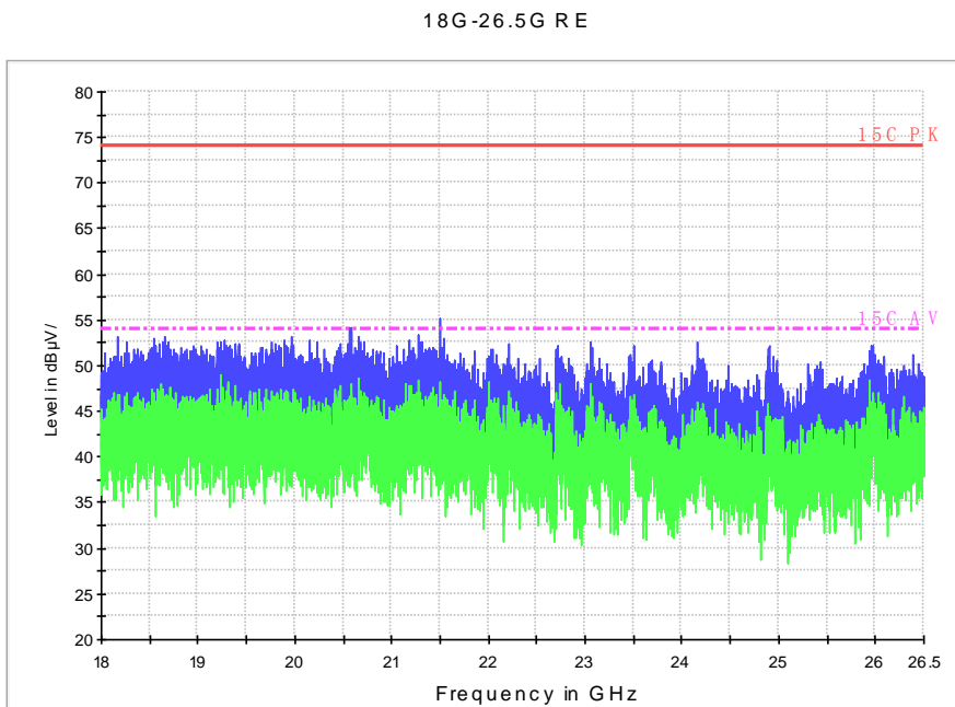
Fig. 57 Radiated Spurious Emission (802.11a, ch36, 18 GHz-26.5 GHz)
