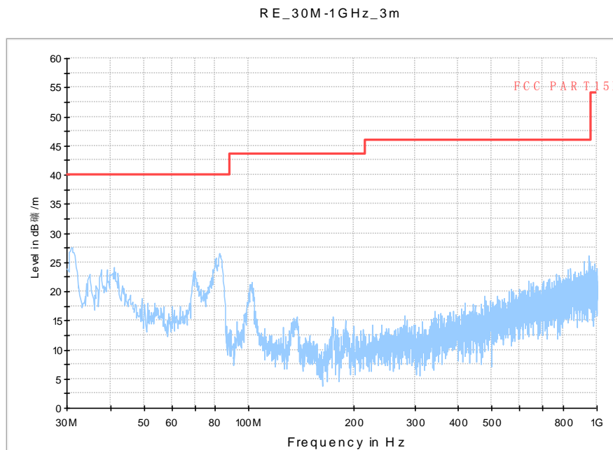
Fig. 77 Radiated Spurious Emission (802.11a, ch56, 30 MHz-1 GHz)
