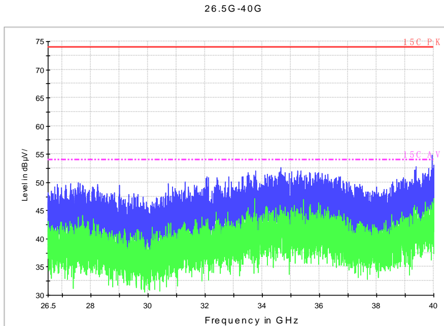
Fig. 100 Radiated Spurious Emission (802.11a, ch120, 26.5 GHz-40 GHz)
