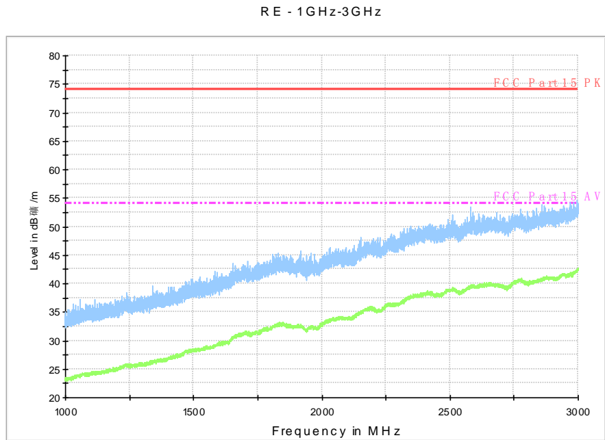
Fig. 96 Radiated Spurious Emission (802.11a, ch120, 1 GHz-3 GHz)
