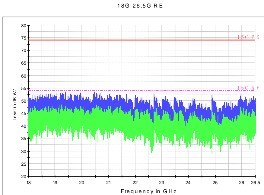
Fig. 69 Radiated Spurious Emission (802.11a, ch48, 18 GHz-26.5 GHz)
