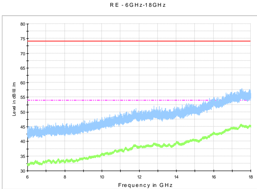
Fig. 110 Radiated Spurious Emission (802.11n-HT20, ch36, 6 GHz-18 GHz)
