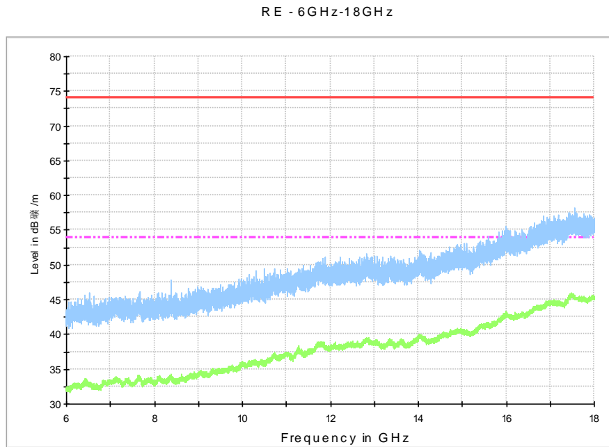
Fig. 68 Radiated Spurious Emission (802.11a, ch48, 6 GHz-18 GHz)
