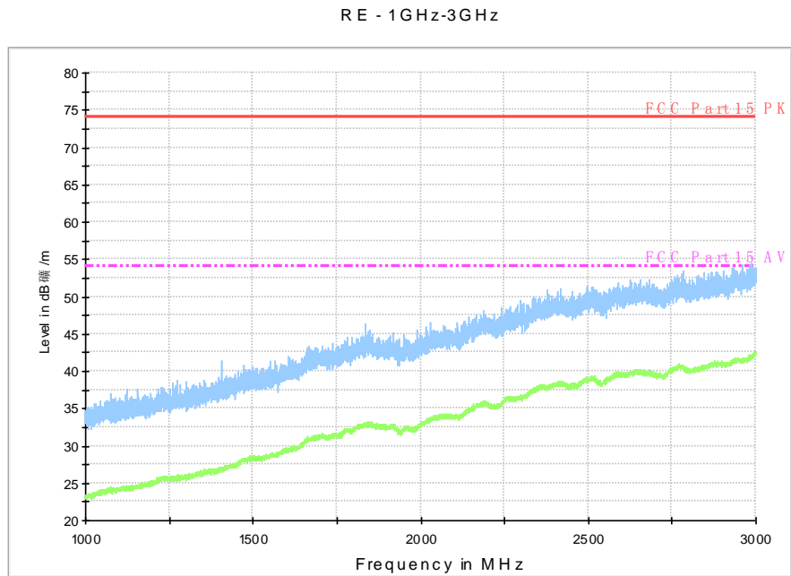
Fig. 102 Radiated Spurious Emission (802.11a, ch140, 1 GHz-3 GHz)
