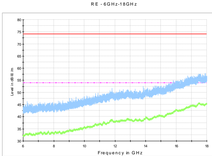
Fig. 80 Radiated Spurious Emission (802.11a, ch56, 6 GHz-18 GHz)
