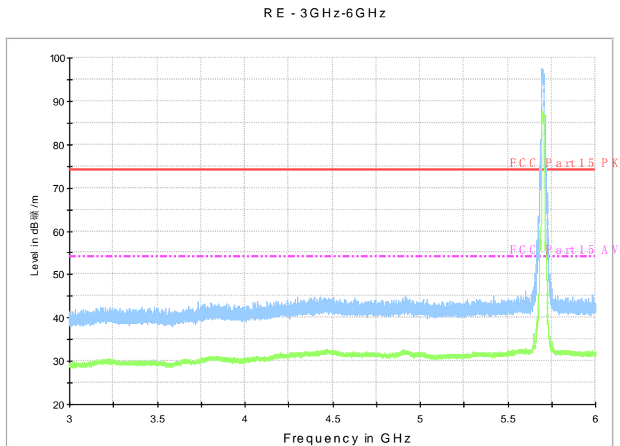
Fig. 103 Radiated Spurious Emission (802.11a, ch140, 3 GHz-6 GHz)
