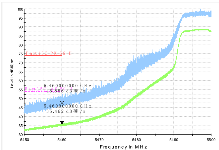
RE - Power-5.45GHz-5.50GHz
