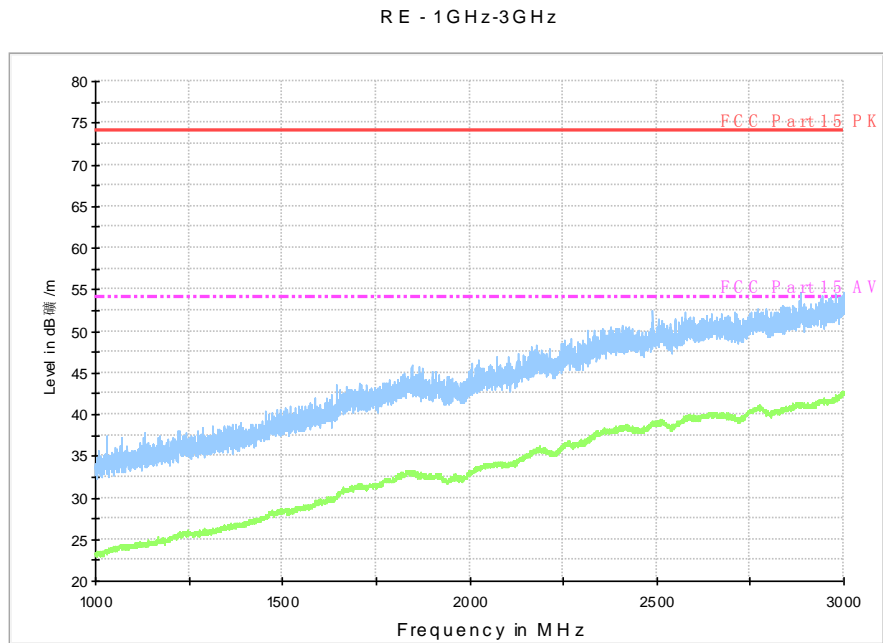
Fig. 108 Radiated Spurious Emission (802.11n-HT20, ch36, 1 GHz-3 GHz)
