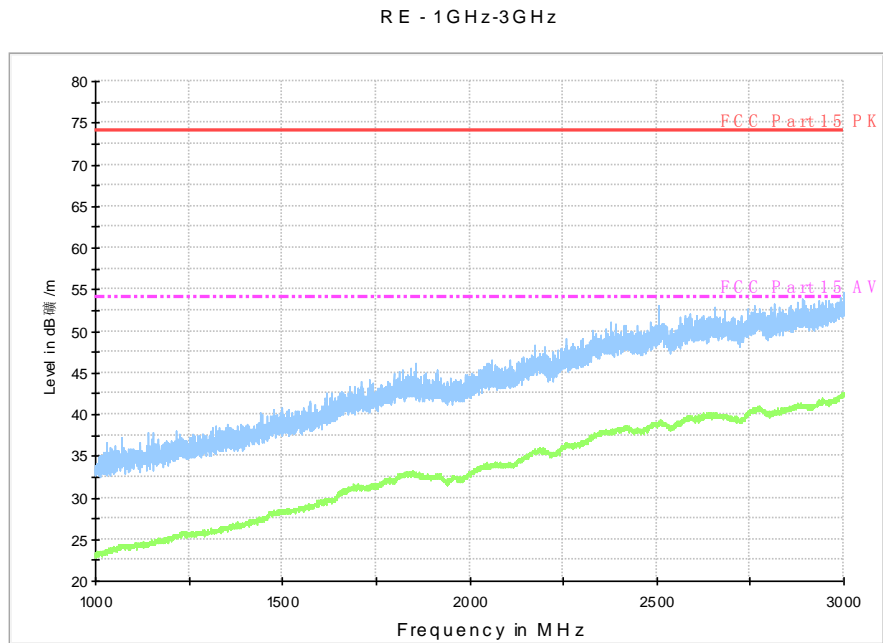
Fig. 90 Radiated Spurious Emission (802.11a, ch100, 1 GHz-3 GHz)
