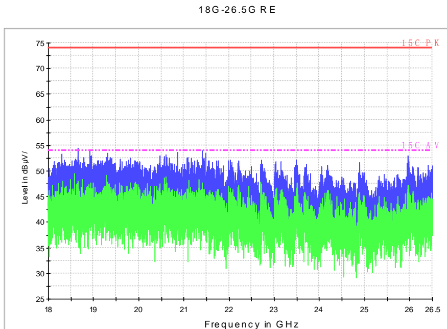
Fig. 75 Radiated Spurious Emission (802.11a, ch52, 18 GHz-26.5 GHz)
