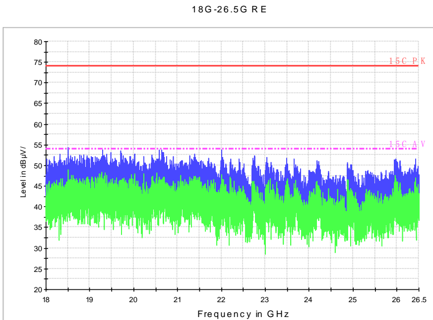
Fig. 99 Radiated Spurious Emission (802.11a, ch120, 18 GHz-26.5 GHz)
