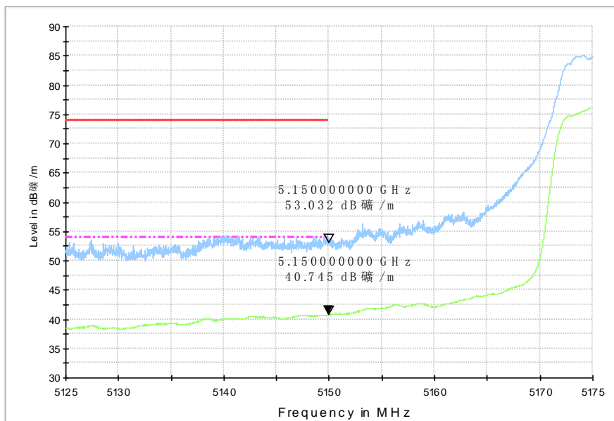
RE - Power-5.125GHz-5.175GHz
