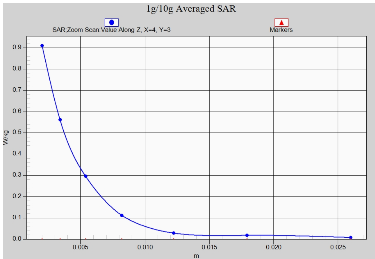
Fig. 32-1 Z-Scan at power reference point (5GHz CH42)
