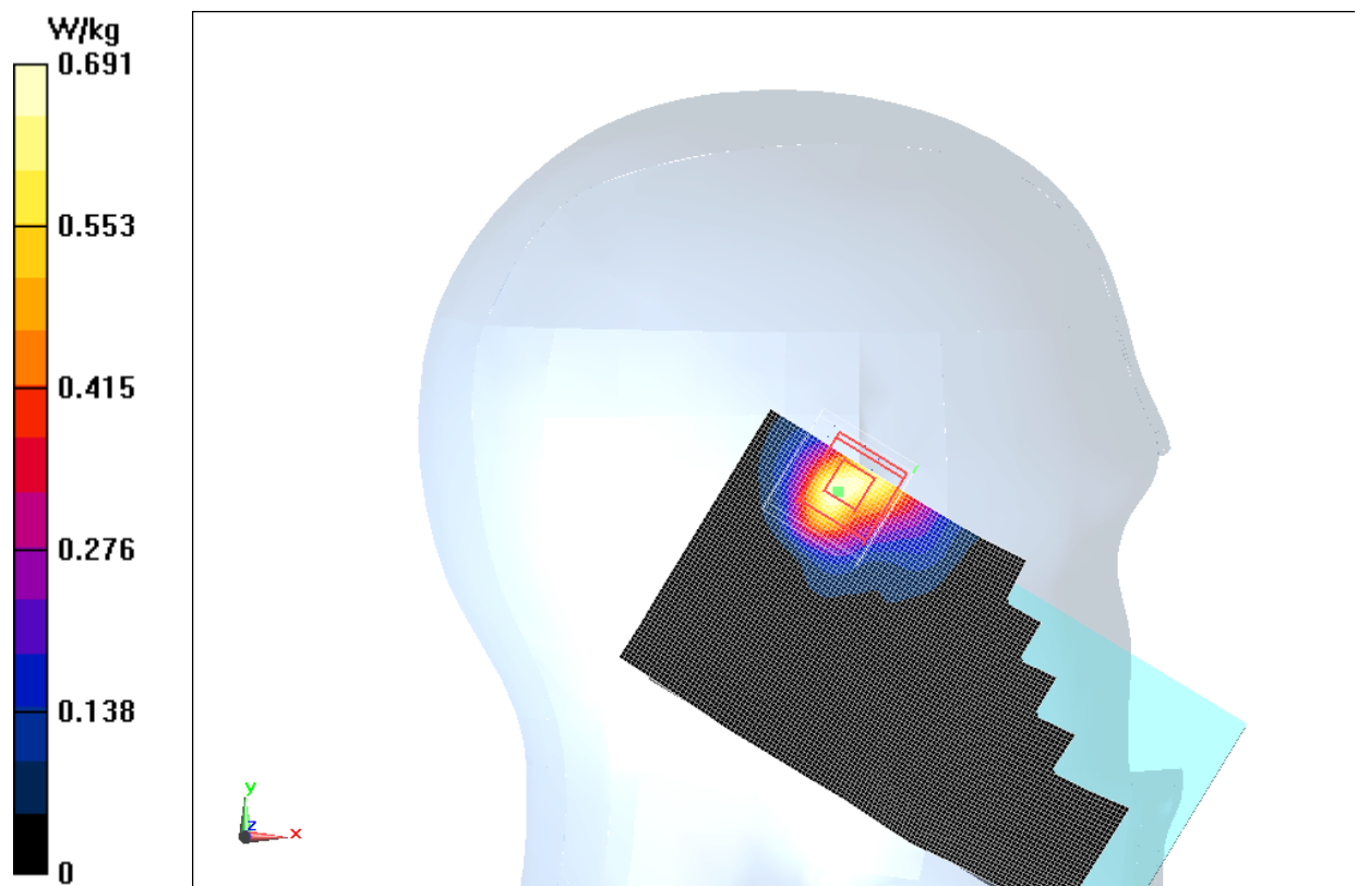
Fig.22 2450 MHz CH6
