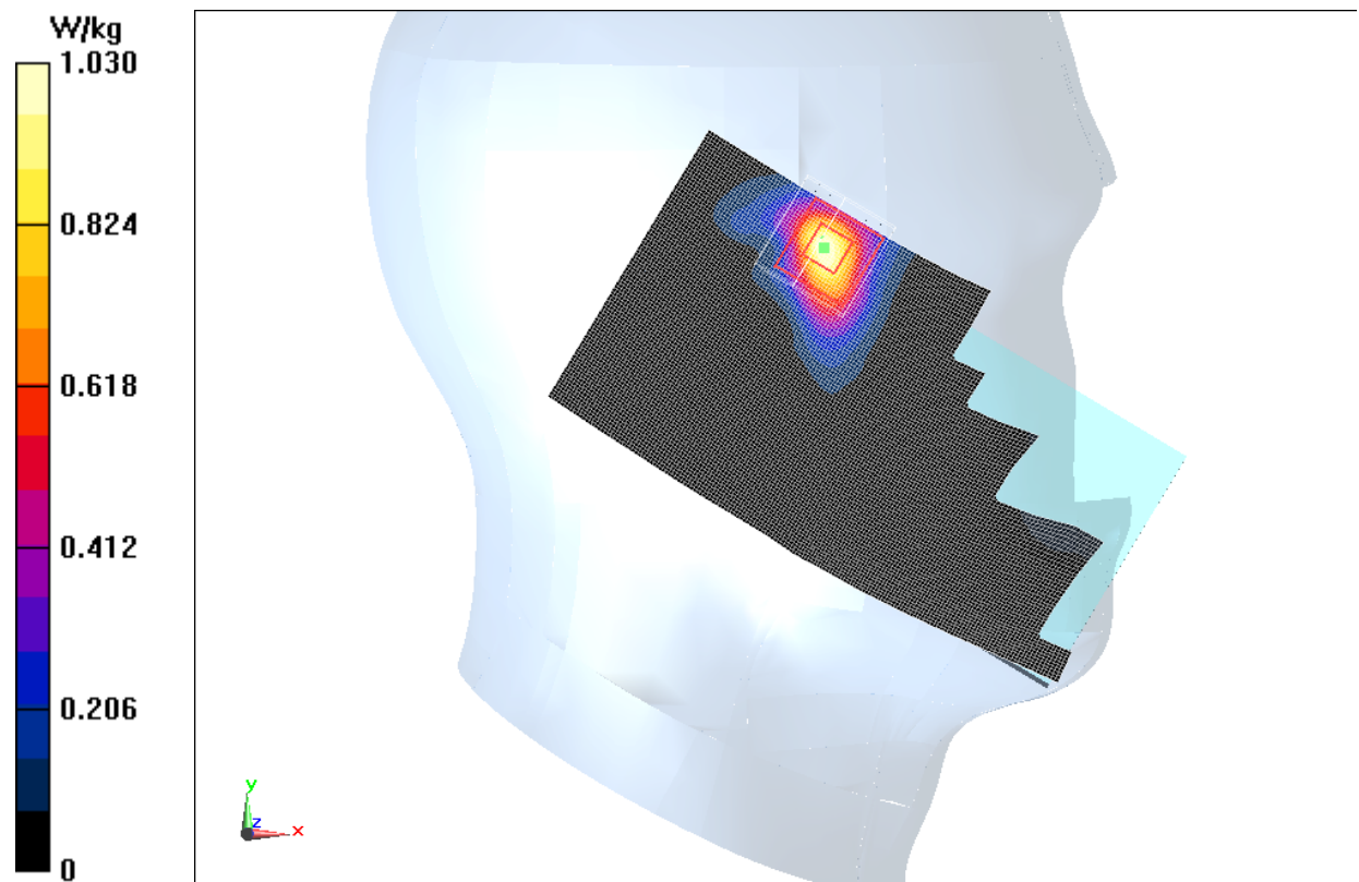
Fig.29 5GHz CH62
