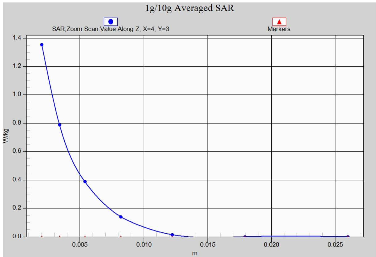
Fig. 26-3 Z-Scan at power reference point (5GHz CH149)
