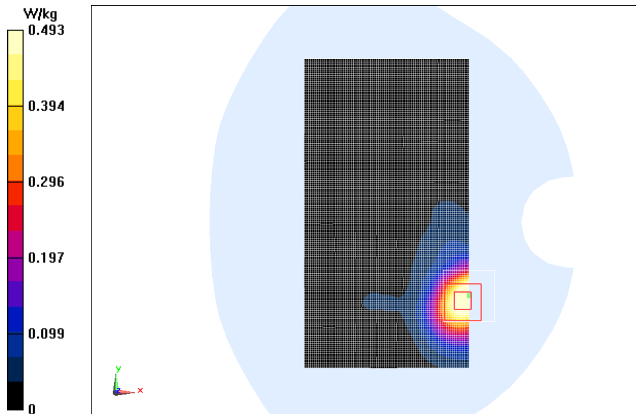
Fig.23 2450 MHz CH1
