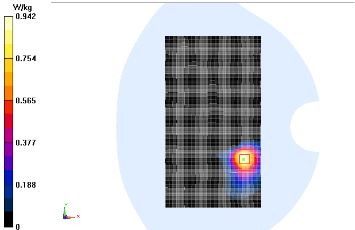
Fig.30 5GHz CH62
