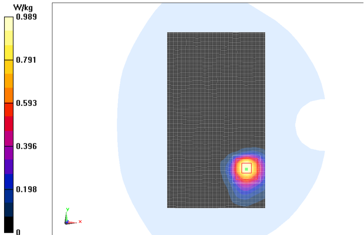
Fig.26 5GHz CH44
