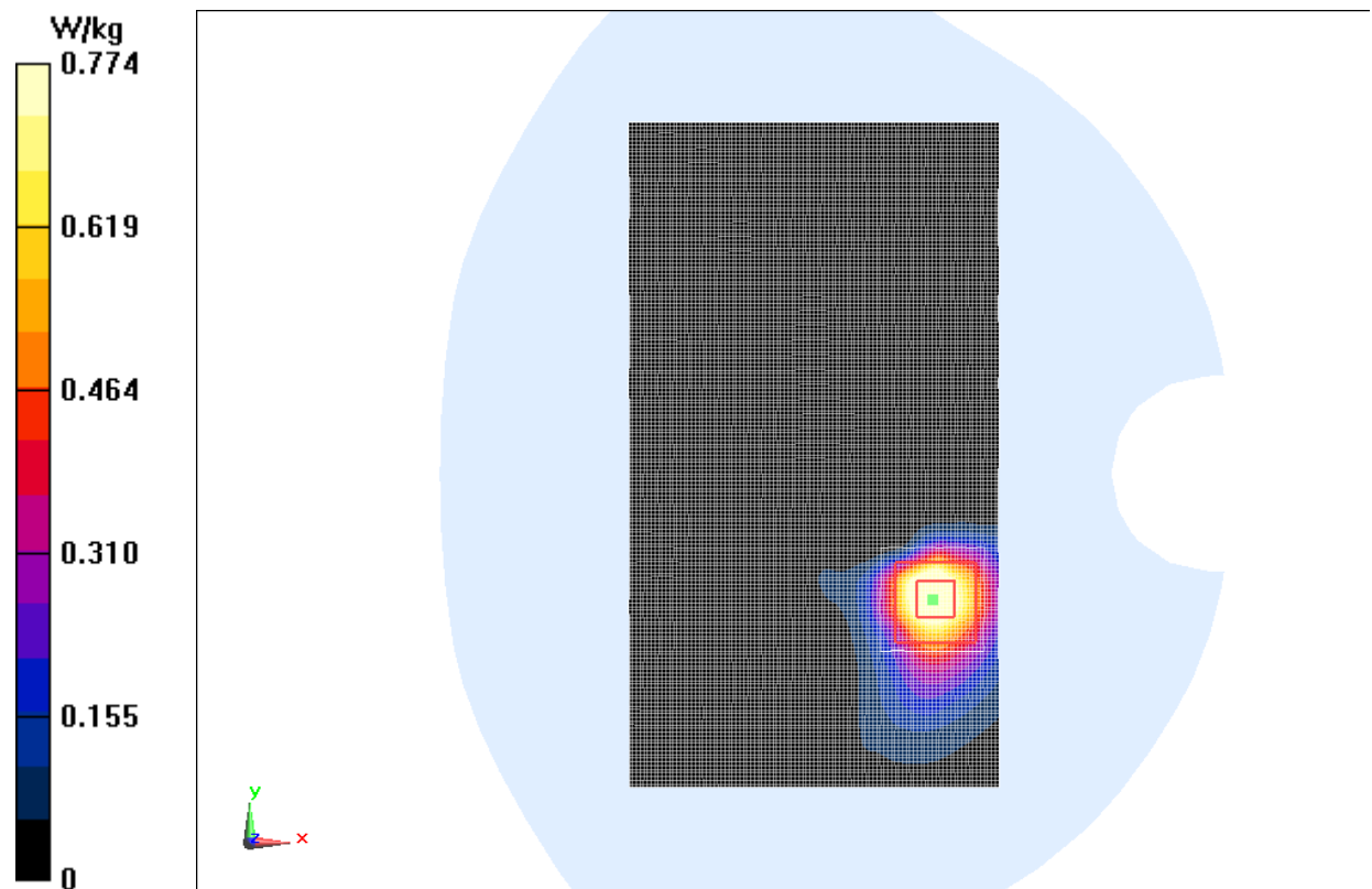
Fig.28 5GHz CH60
