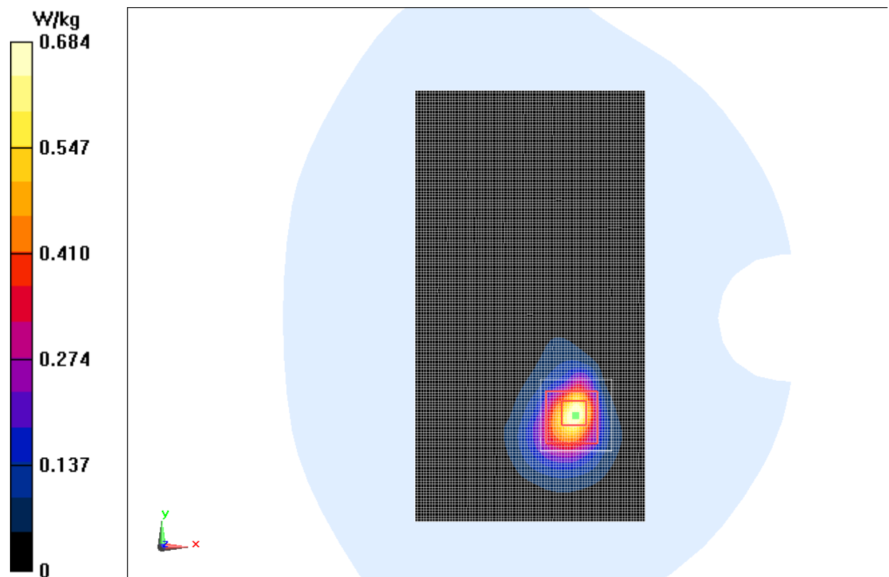
Fig.24 2450 MHz CH6
