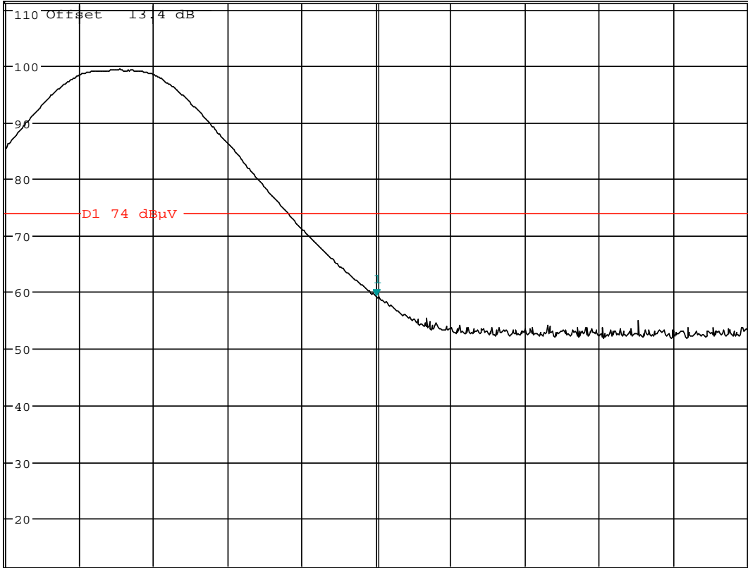
Plot 6-19. Radiated Restricted Band Edge Plot (Peak)
