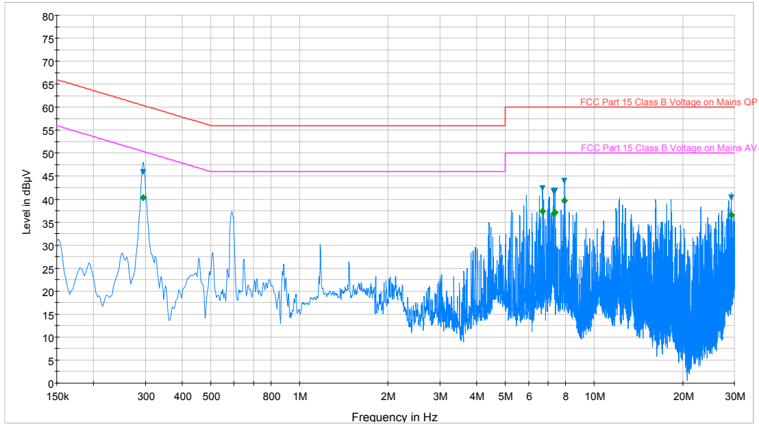
Plot 6-20. Line Conducted Plot with Bluetooth LE (L1)
