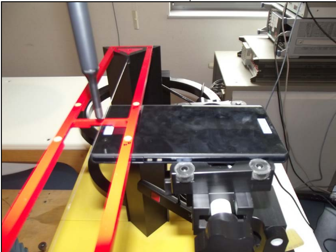
Photo 6: HAC test position
