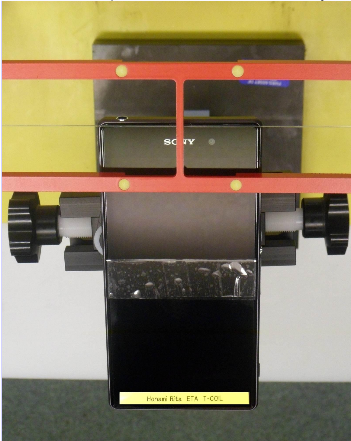
PHT/10027127JD01B/004: Top View of EUT Under Test Arch Phantom - T-Coil testing
