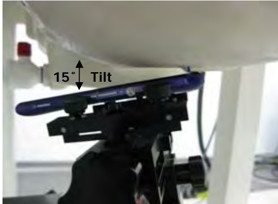
Fig.19 Left Head Section / Ear-Tilt Position(15°)
