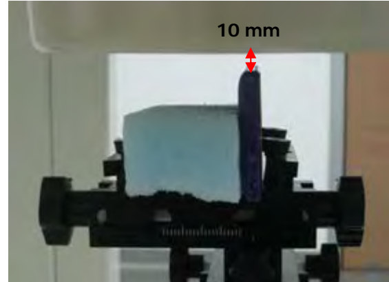
Fig.23 EUT left to flat phantom
