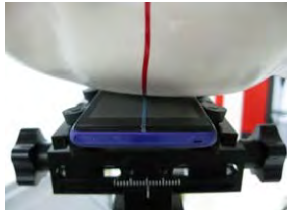
Fig.16 Right Head Section / Cheek-Touch Position
