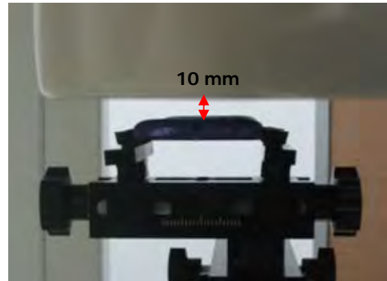
Fig.21 EUT back to flat phantom
