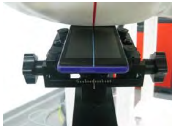
Fig.17 Right Head Section / Ear-Tilt Position(15°)
