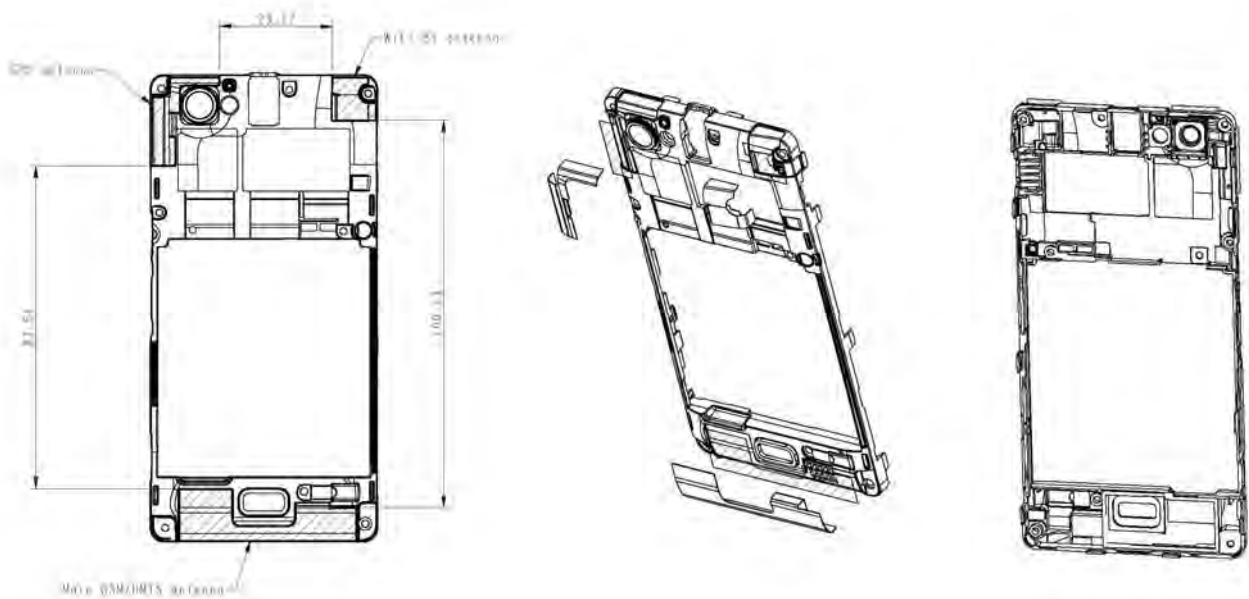
Fig.36 Antenna position of EUT
