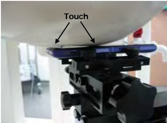
Fig.16 Right Head Section / Cheek-Touch Position
