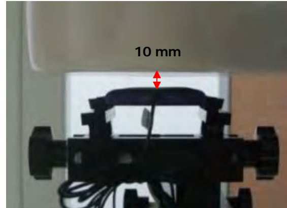
Fig.24 EUT back side with headset (MH410C) to flat phantom
