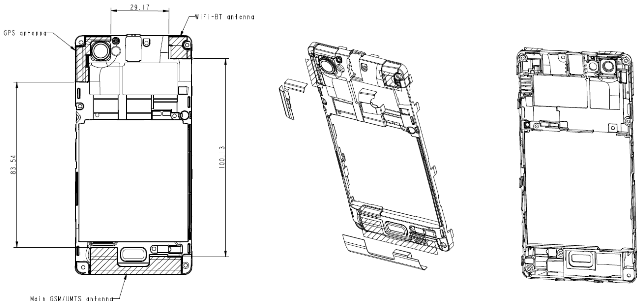
Fig.21 Antenna position of EUT
