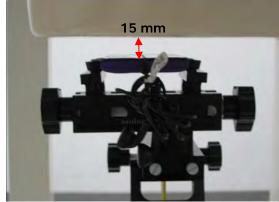
Fig.7 EUT front side with headset (MH410C) to flat phantom
