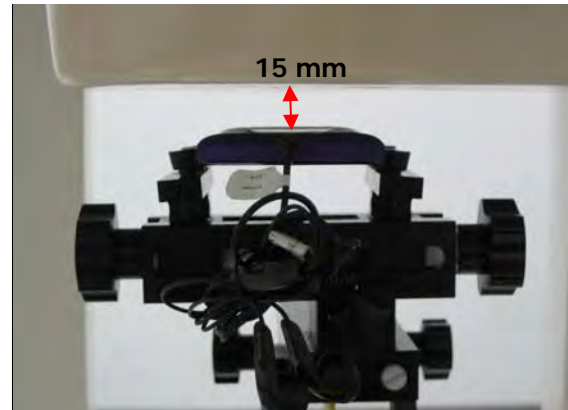
Fig.8 EUT back side with headset (MH410C) to flat phantom
