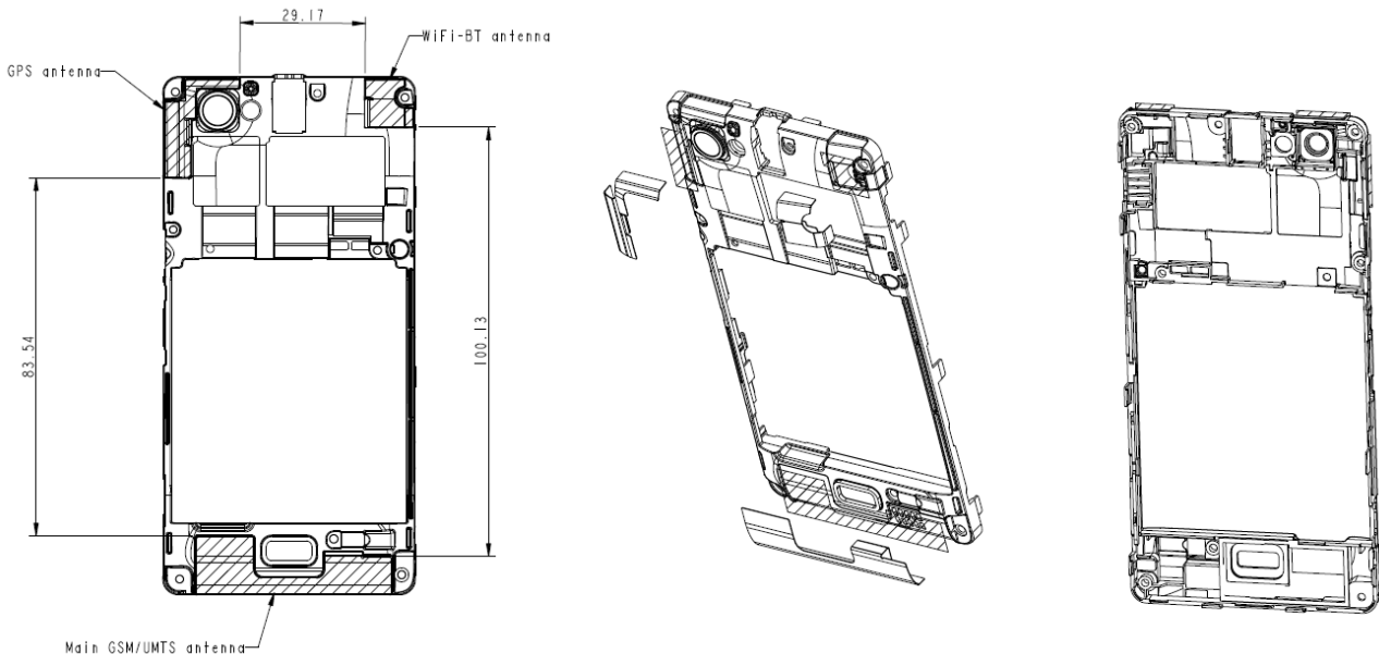
Fig.32 Antenna position of EUT
