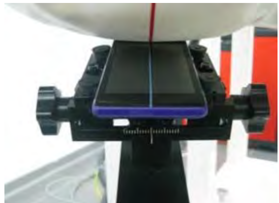
Fig.18 Right Head Section / Ear-Tilt Position(15°)
