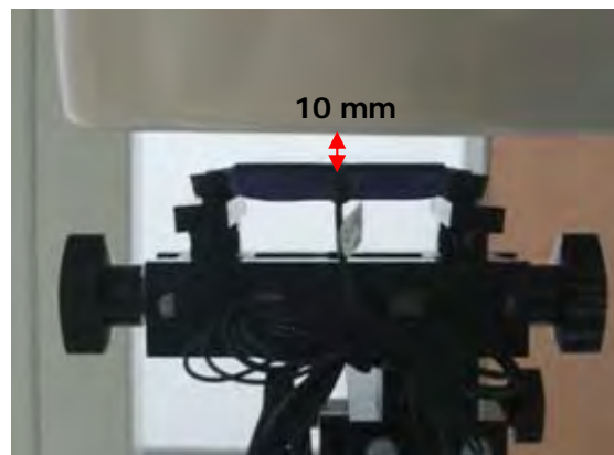
Fig.26 EUT front with headset (MH410C) to flat phantom
