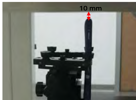
Fig.24 EUT bottom to flat phantom
