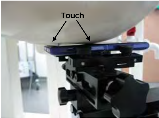
Fig.17 Right Head Section / Cheek-Touch Position
