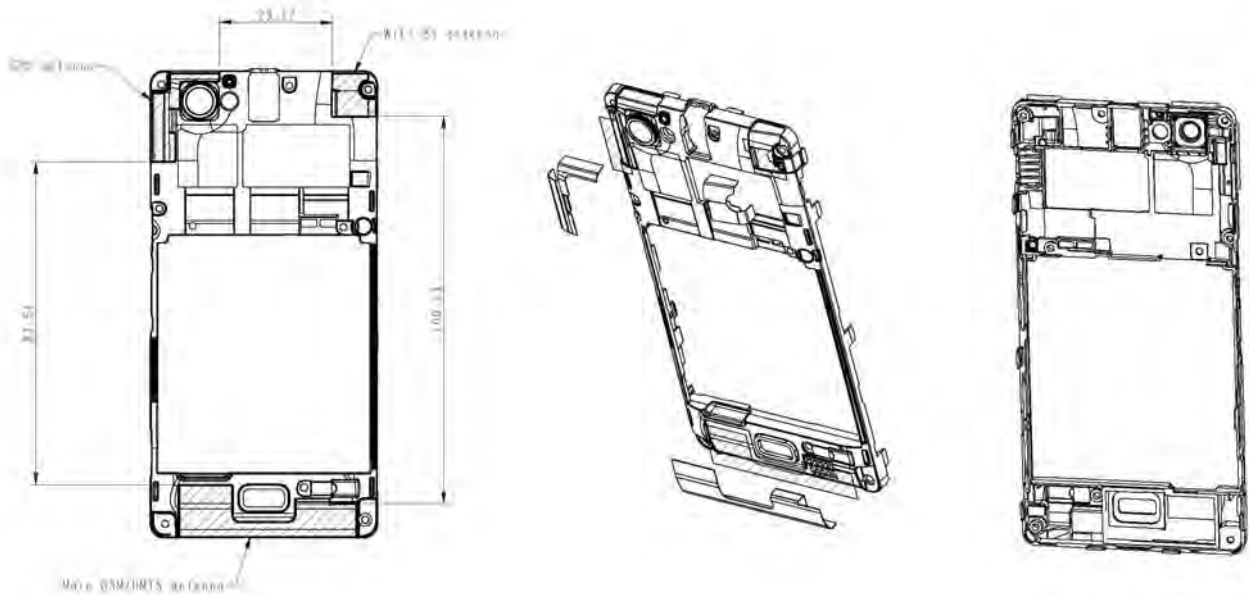
Fig.38 Antenna position of EUT
