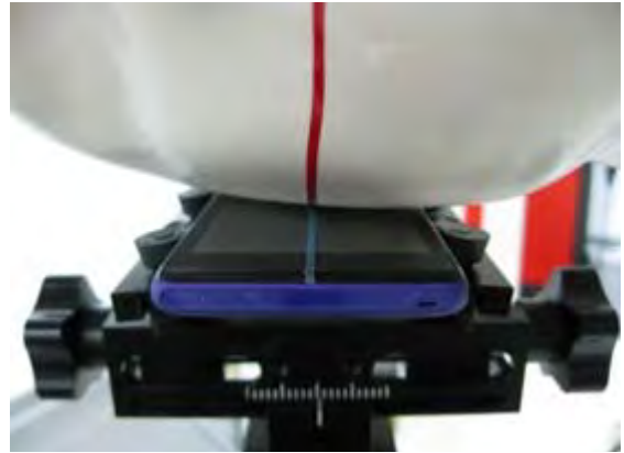
Fig.17 Right Head Section / Cheek-Touch Position
