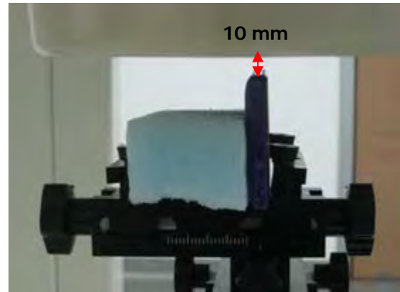
Fig.25 EUT left to flat phantom
