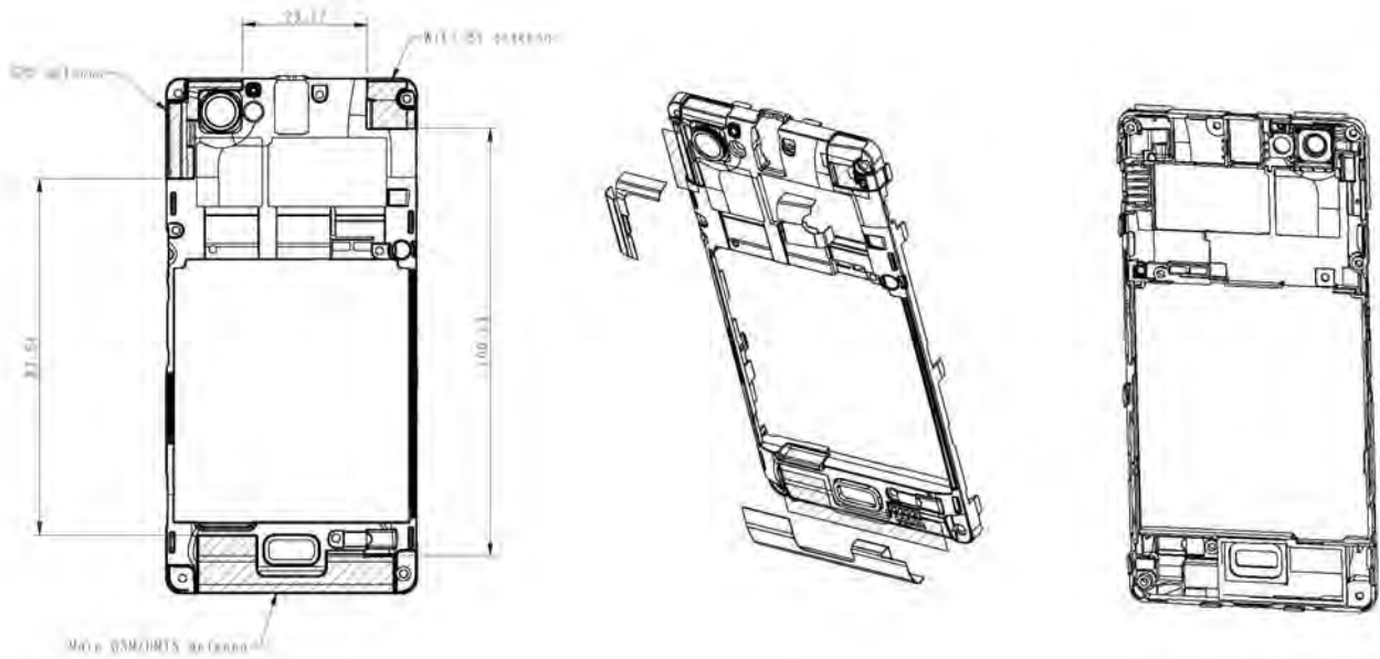
Fig.38 Antenna position of EUT
