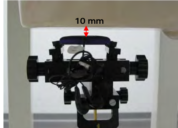
Fig.12 EUT back with headset (MH410C) to flat phantom
