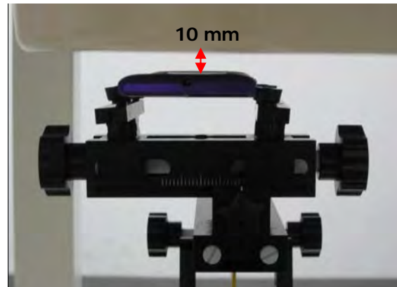
Fig.11 EUT back to flat phantom
