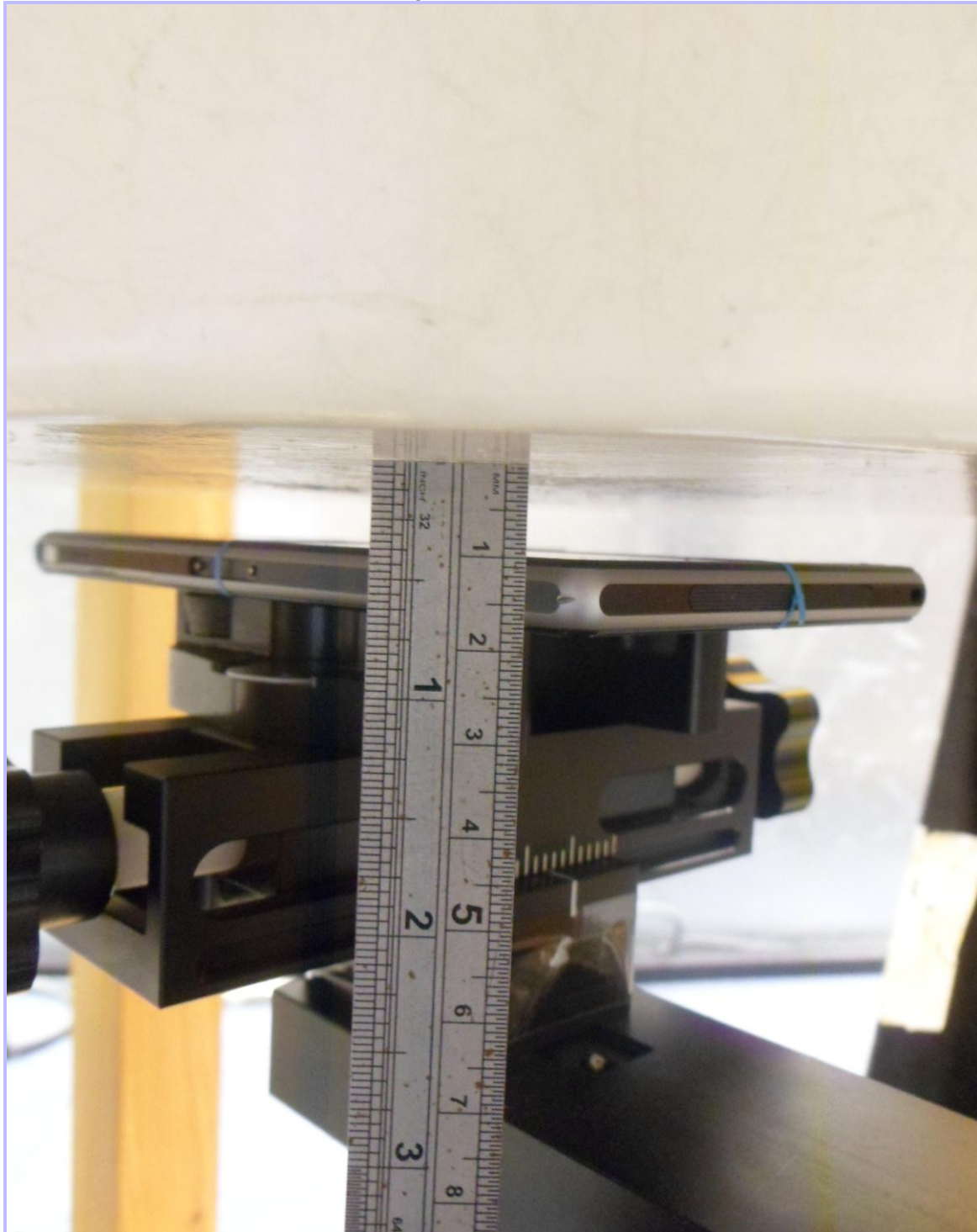
PHT/10014929/006: Front of EUT Facing Phantom at 10mm
