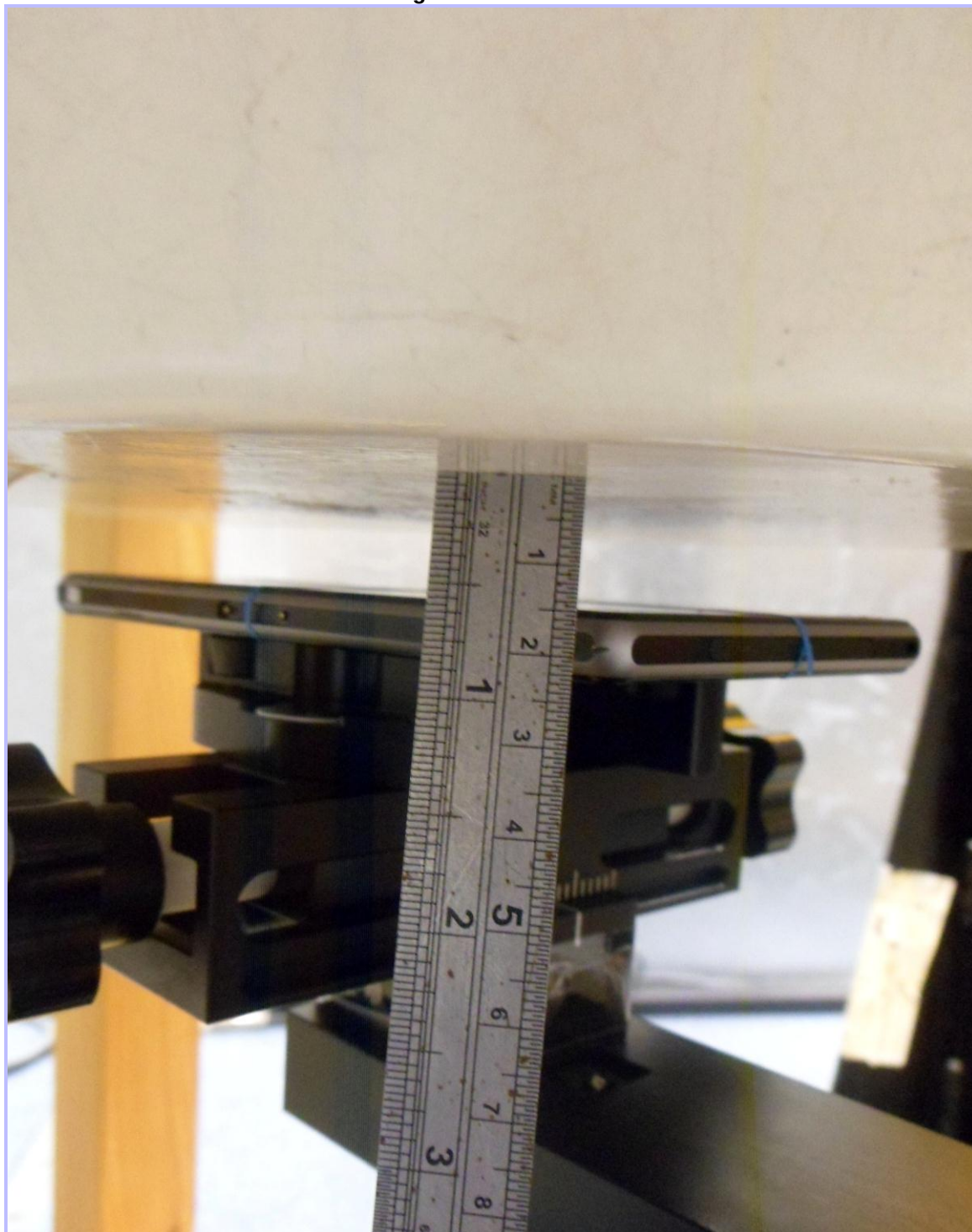
PHT/10014929/007: Front of EUT Facing Phantom at 15m
