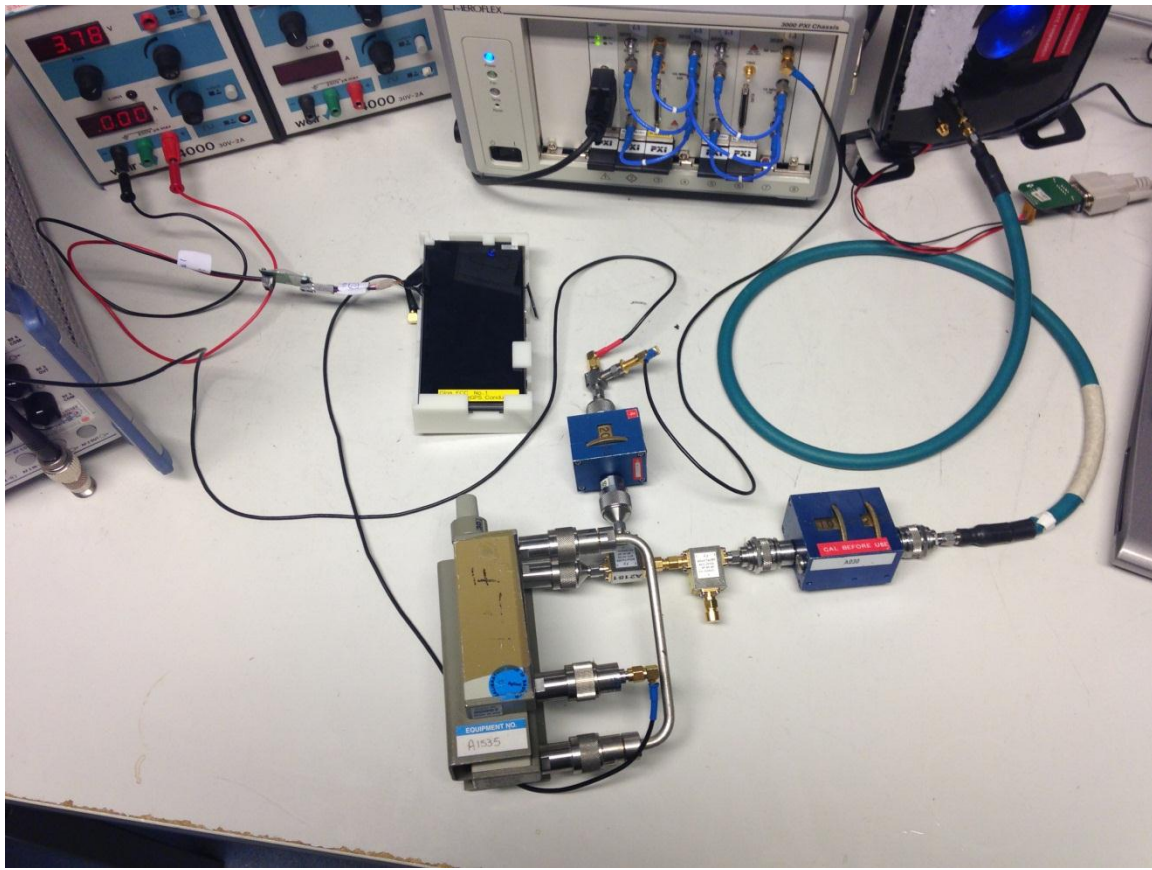
WLAN 5GHz DFS Test Set-Up Photos for PY7PM-0470
