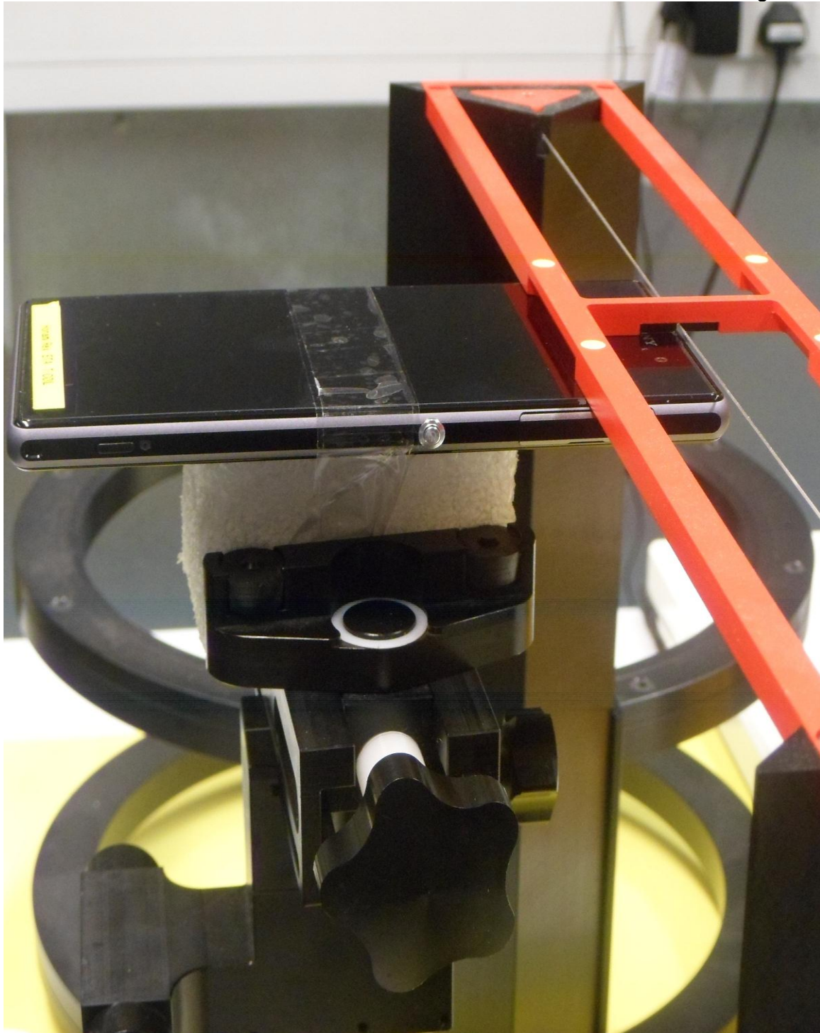
PHT/10014945JD23B/003: Side View of EUT Under Test Arch Phantom - T-Coil testing
