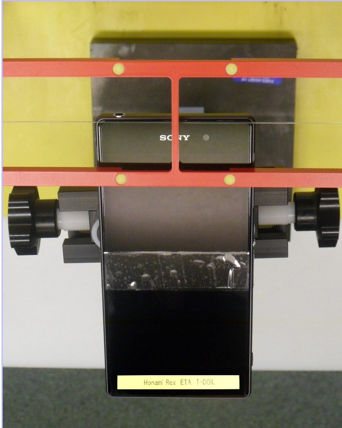
PHT/10014945JD23B/004: Top View of EUT Under Test Arch Phantom - T-Coil testing
