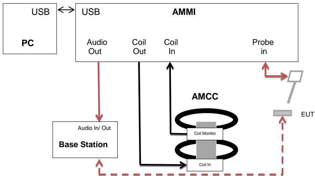
Figure 1: Test set up Diagram T-coil
