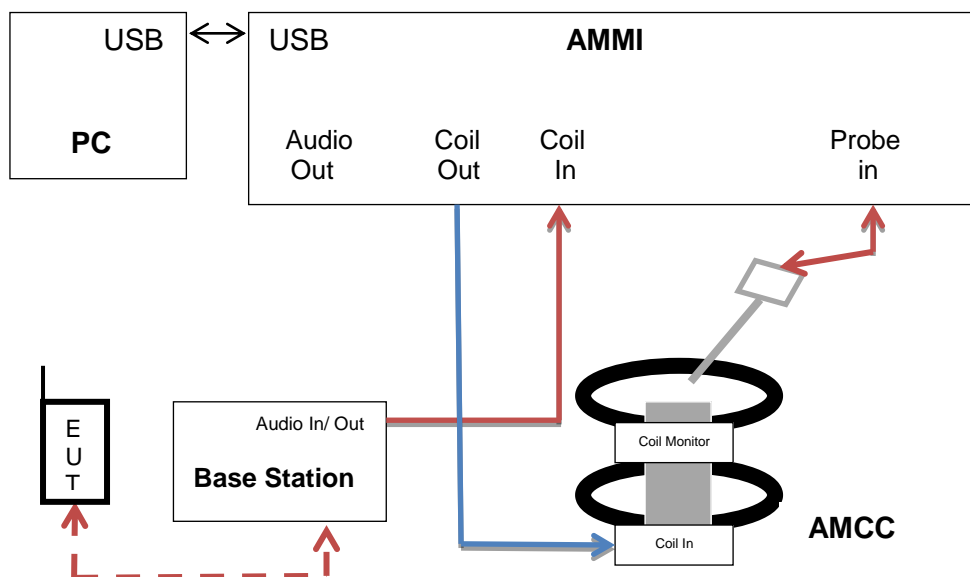
Figure 2: RF reference signal measurement Set-up
