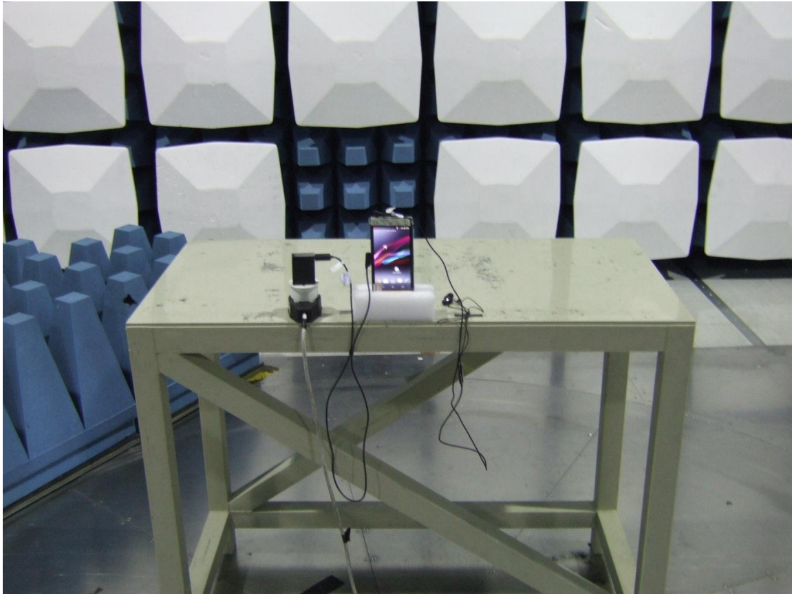
Radiated Emissions: Accessory Configuration 2
