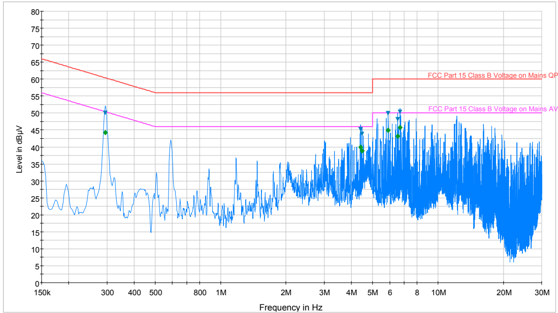
Plot 6-73. Line Conducted Plot with 802.11a (L1)
