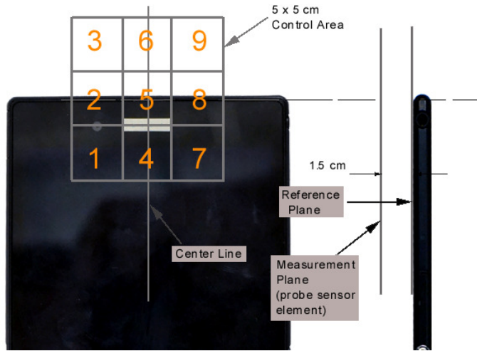
Figure 18-3 5x5 Scan grid above WD
