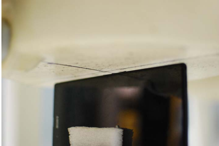
SAR Test Setup Photo 16 – Right Edge at 0.3 cm
