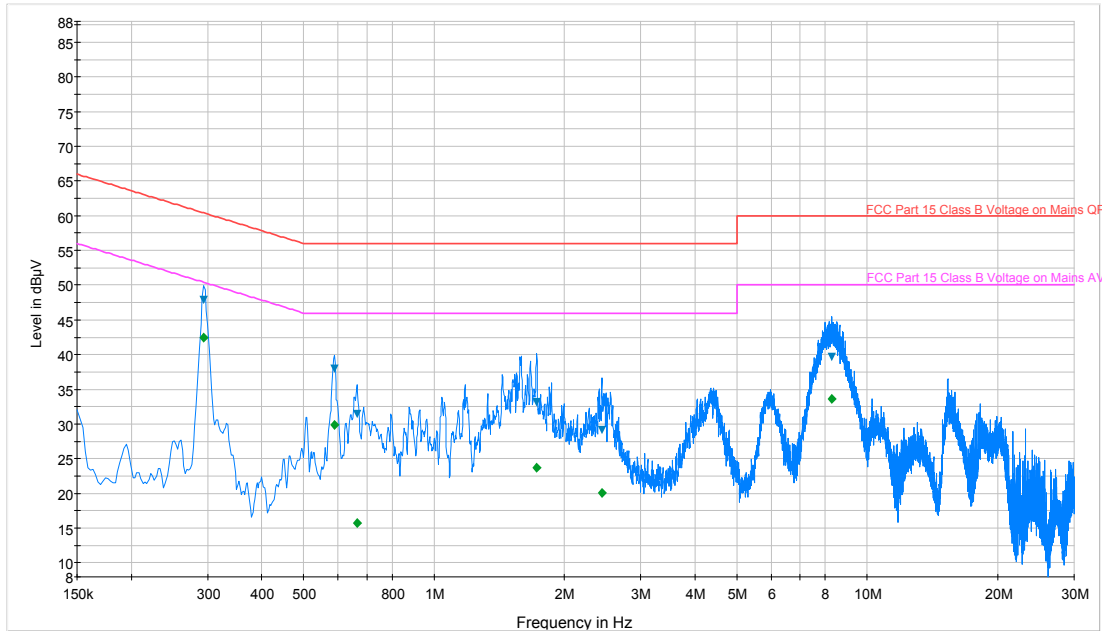
Plot 6-71. Line Conducted Plot with 802.11b (L1)
