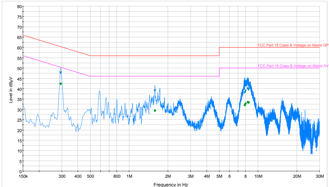
Plot 6-72. Line Conducted Plot with 802.11b (N)
