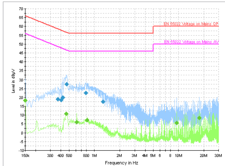
Fig. 88 AC Powerline Conducted Emission-802.11a mode
