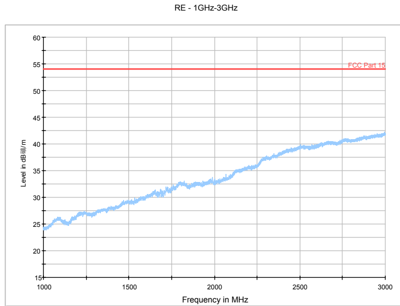
Fig. 48 Radiated Spurious Emission (802.11a, Ch157, 1 GHz-3 GHz)
