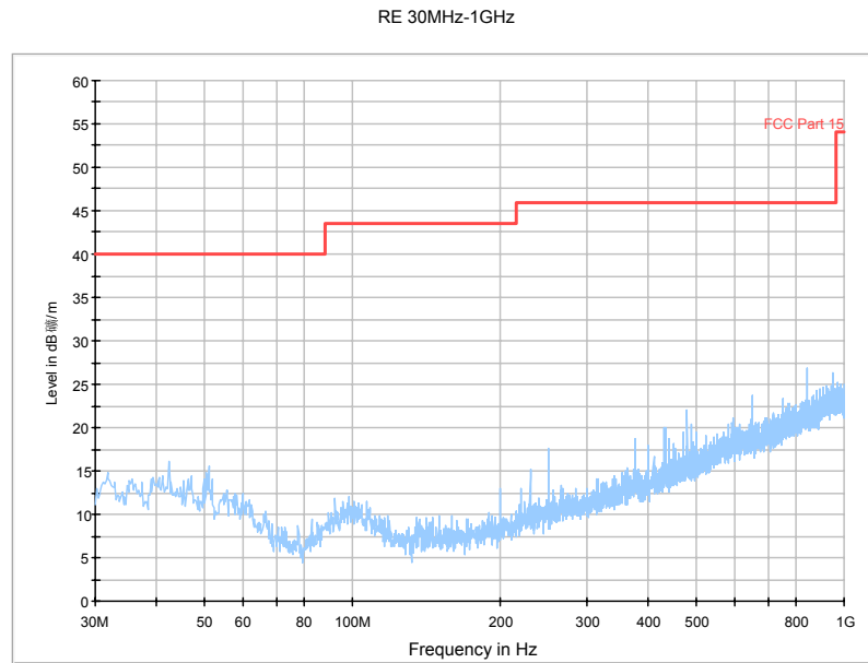
Fig. 59 Radiated Spurious Emission (802.11n-HT20, Ch149, 30 MHz-1 GHz)
