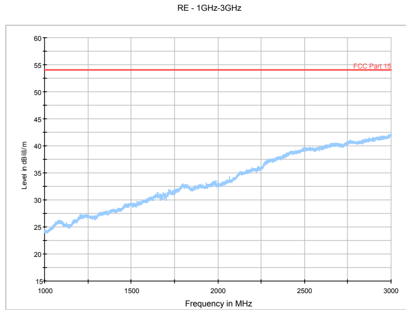
Fig. 66 Radiated Spurious Emission (802.11n-HT20, Ch157, 1 GHz-3 GHz)
