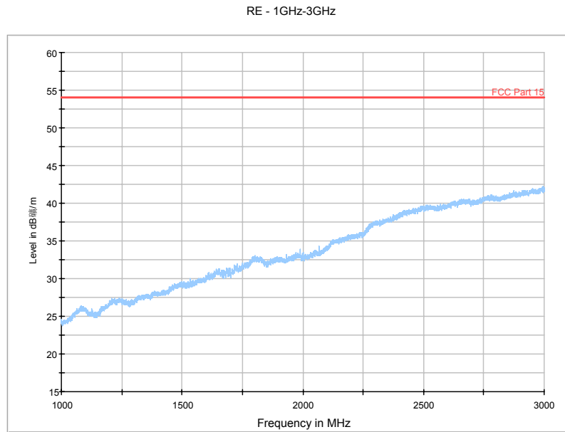
Fig. 78 Radiated Spurious Emission (802.11n-HT40, Ch151, 1 GHz-3 GHz)
