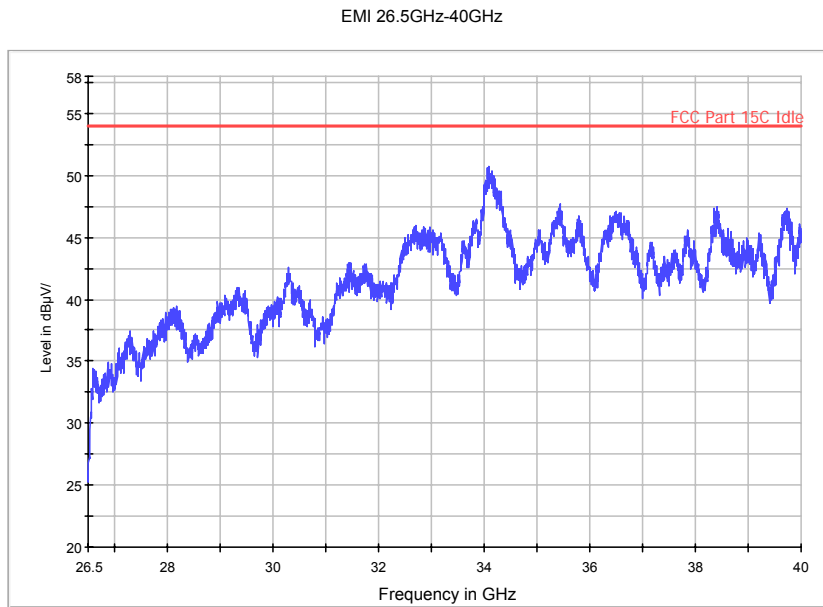
Fig. 76 Radiated Spurious Emission (802.11n-HT20, Ch165, 26.5 GHz-40 GHz)
