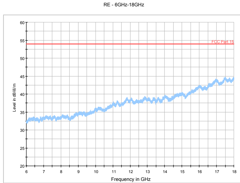
Fig. 74 Radiated Spurious Emission (802.11n-HT20, Ch165, 6 GHz-18 GHz)
