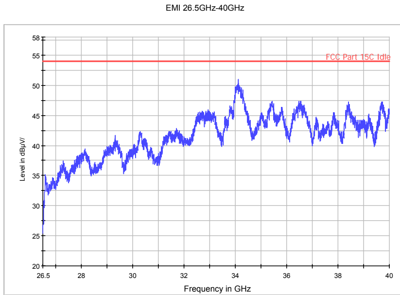
Fig. 70 Radiated Spurious Emission (802.11n-HT20, Ch157, 26.5 GHz-40 GHz)
