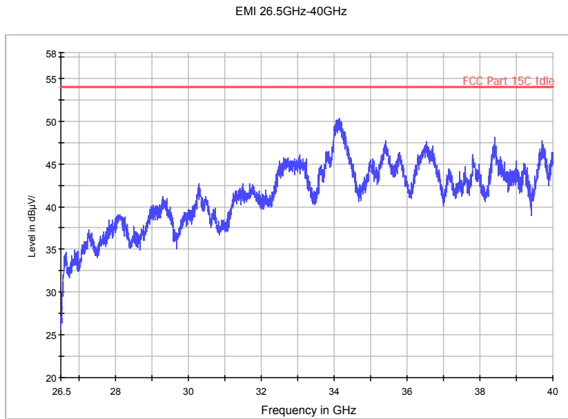
Fig. 46 Radiated Spurious Emission (802.11a, Ch149, 26.5 GHz-40 GHz)
