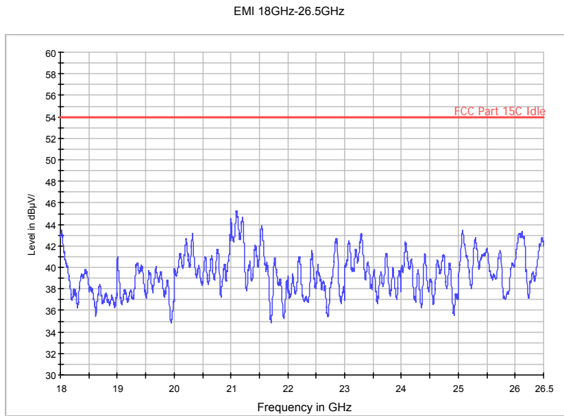
Fig. 86 Radiated Spurious Emission (802.11n-HT40, Ch159, 18 GHz-26.5 GHz)
