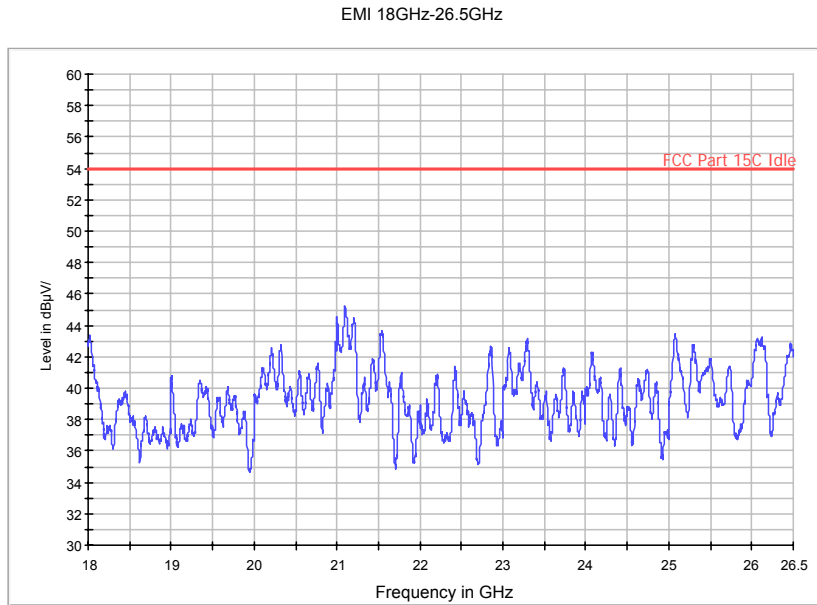
Fig. 81 Radiated Spurious Emission (802.11n-HT40, Ch151, 18 GHz-26.5 GHz)
