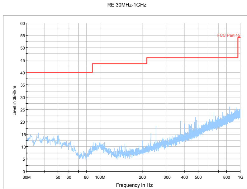
Fig. 71 Radiated Spurious Emission (802.11n-HT20, Ch165, 30 MHz-1 GHz)
