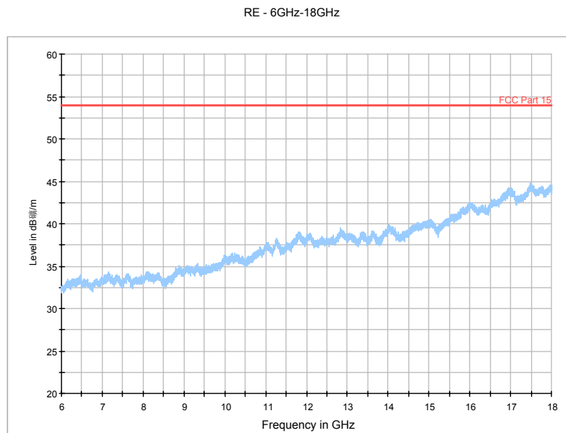
Fig. 85 Radiated Spurious Emission (802.11n-HT40, Ch159, 6 GHz-18 GHz)
