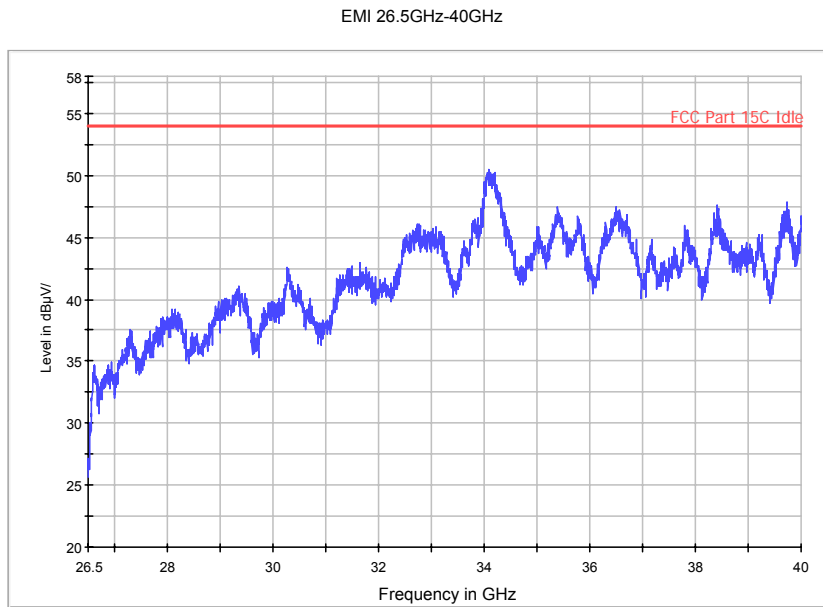
Fig. 52 Radiated Spurious Emission (802.11a, Ch165, 26.5 GHz-40 GHz)
