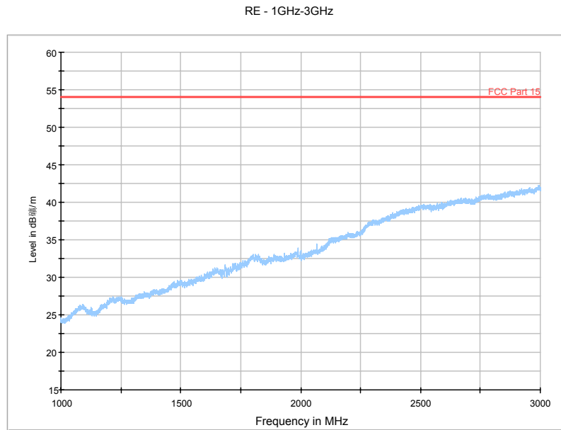
Fig. 72 Radiated Spurious Emission (802.11n-HT20, Ch165, 1 GHz-3 GHz)
