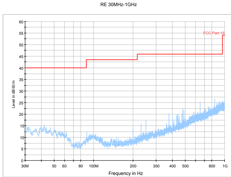
Fig. 47 Radiated Spurious Emission (802.11a, Ch157, 30 MHz-1 GHz)
