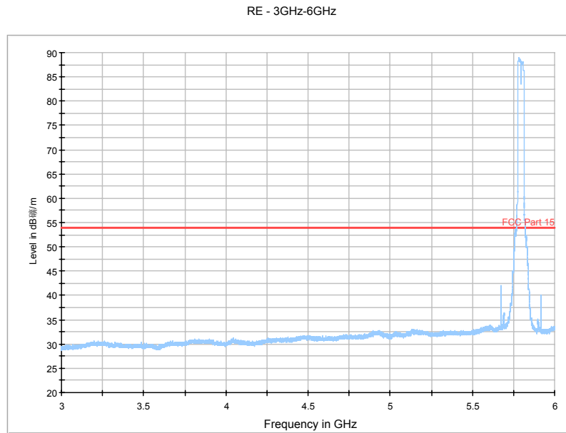
Fig. 84 Radiated Spurious Emission (802.11n-HT40, Ch159, 3 GHz-6 GHz)
