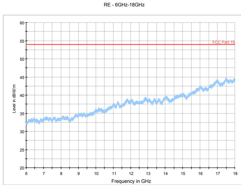
Fig. 50 Radiated Spurious Emission (802.11a, Ch157, 6 GHz-18 GHz)
