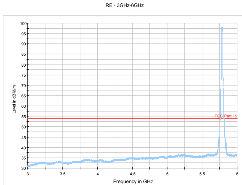
Fig. 49 Radiated Spurious Emission (802.11a, Ch157, 3 GHz-6 GHz)
