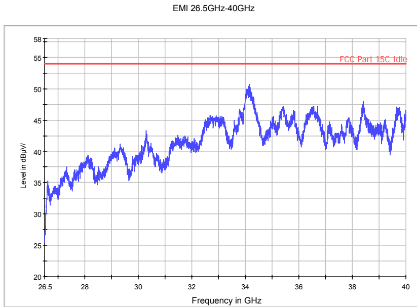
Fig. 64 Radiated Spurious Emission (802.11n-HT20, Ch149, 26.5 GHz-40 GHz)
