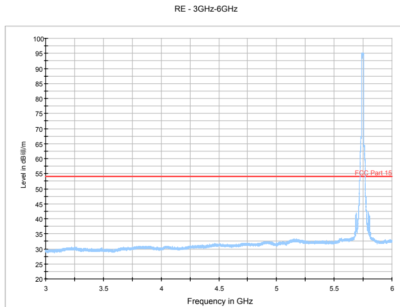
Fig. 61 Radiated Spurious Emission (802.11n-HT20, Ch149, 3 GHz-6 GHz)
