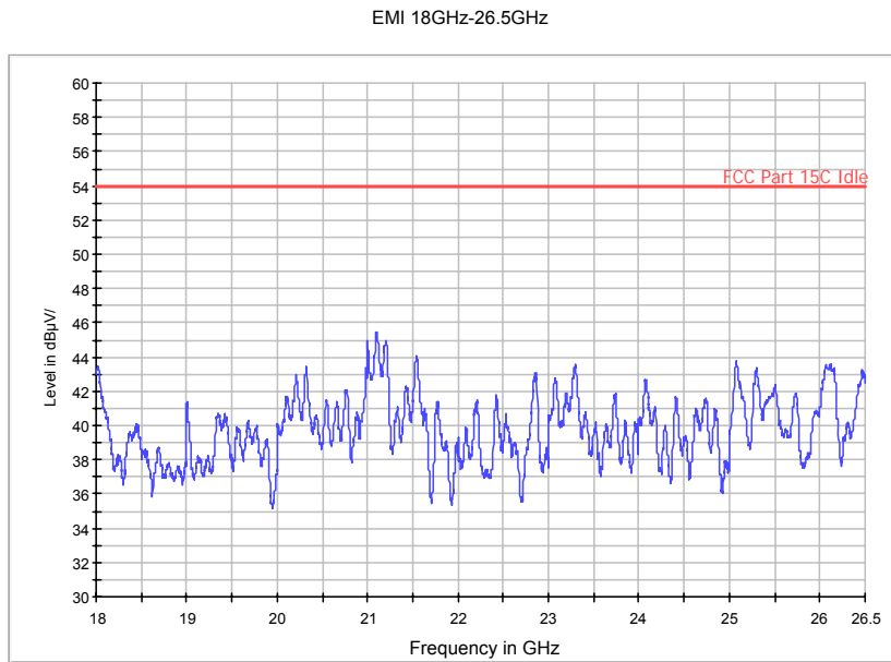
Fig. 63 Radiated Spurious Emission (802.11n-HT20, Ch149, 18 GHz-26.5 GHz)
