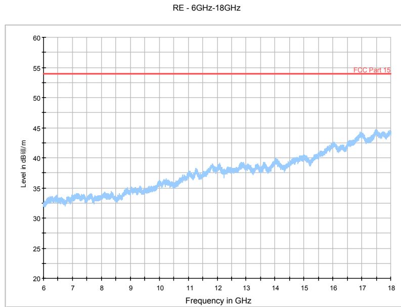
Fig. 80 Radiated Spurious Emission (802.11n-HT40, Ch151, 6 GHz-18 GHz)
