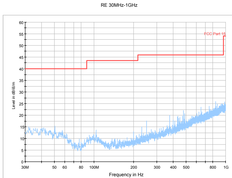
Fig. 53 Radiated Spurious Emission (802.11a, Ch165, 30 MHz-1 GHz)
