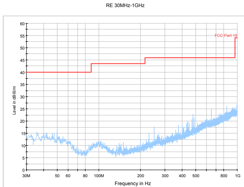
Fig. 77 Radiated Spurious Emission (802.11n-HT40, Ch151, 30 MHz-1 GHz)
