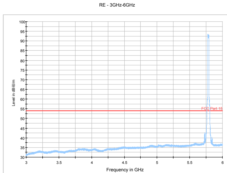
Fig. 67 Radiated Spurious Emission (802.11n-HT20, Ch157, 3 GHz-6 GHz)
