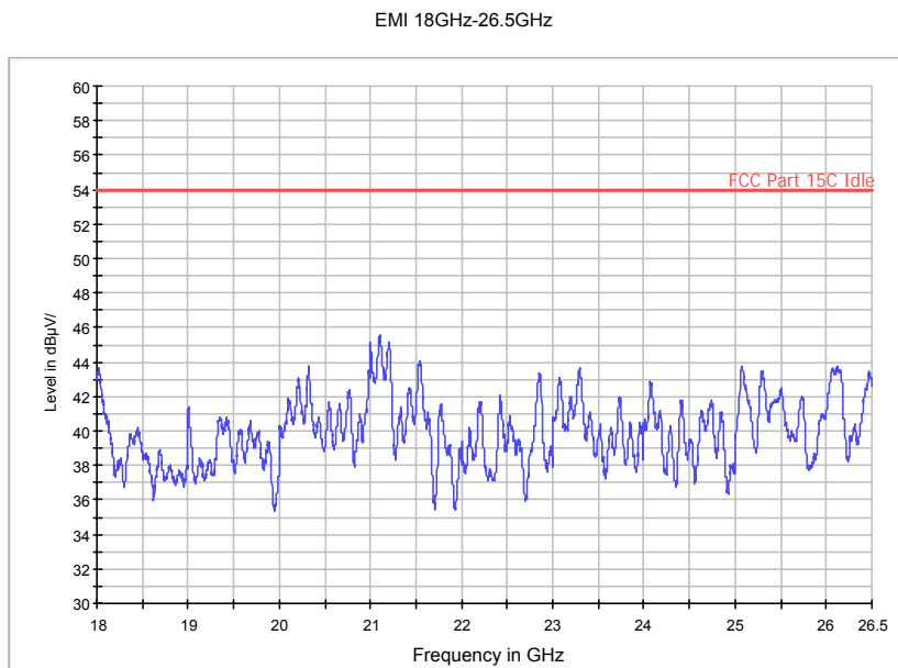
Fig. 51 Radiated Spurious Emission (802.11a, Ch157, 18 GHz-26.5 GHz)
