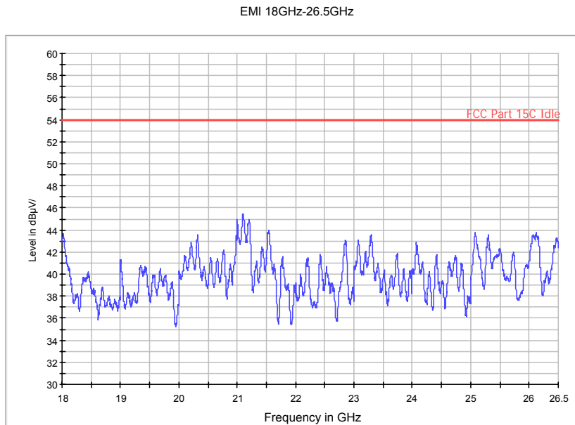
Fig. 57 Radiated Spurious Emission (802.11a, Ch165, 18 GHz-26.5 GHz)
