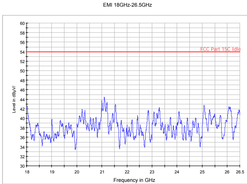
Fig. 75 Radiated Spurious Emission (802.11n-HT20, Ch165, 18 GHz-26.5 GHz)
