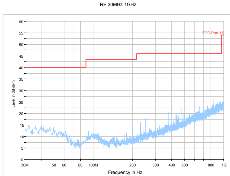
Fig. 82 Radiated Spurious Emission (802.11n-HT40, Ch159, 30 MHz-1 GHz)
