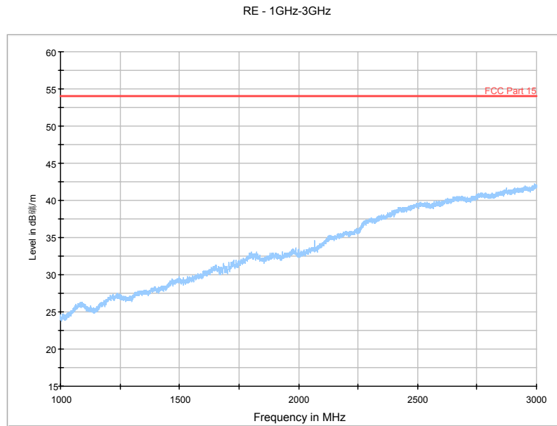
Fig. 54 Radiated Spurious Emission (802.11a, Ch165, 1 GHz-3 GHz)
