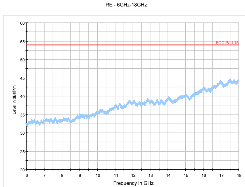
Fig. 62 Radiated Spurious Emission (802.11n-HT20, Ch149, 6 GHz-18 GHz)
