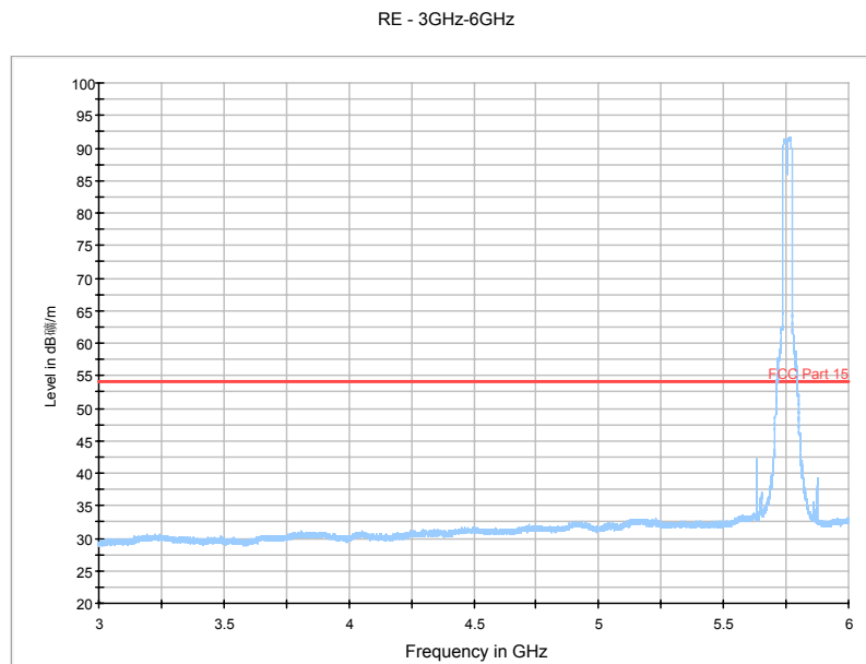
Fig. 79 Radiated Spurious Emission (802.11n-HT40, Ch151, 3 GHz-6 GHz)
