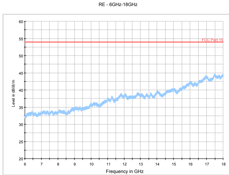
Fig. 68 Radiated Spurious Emission (802.11n-HT20, Ch157, 6 GHz-18 GHz)
