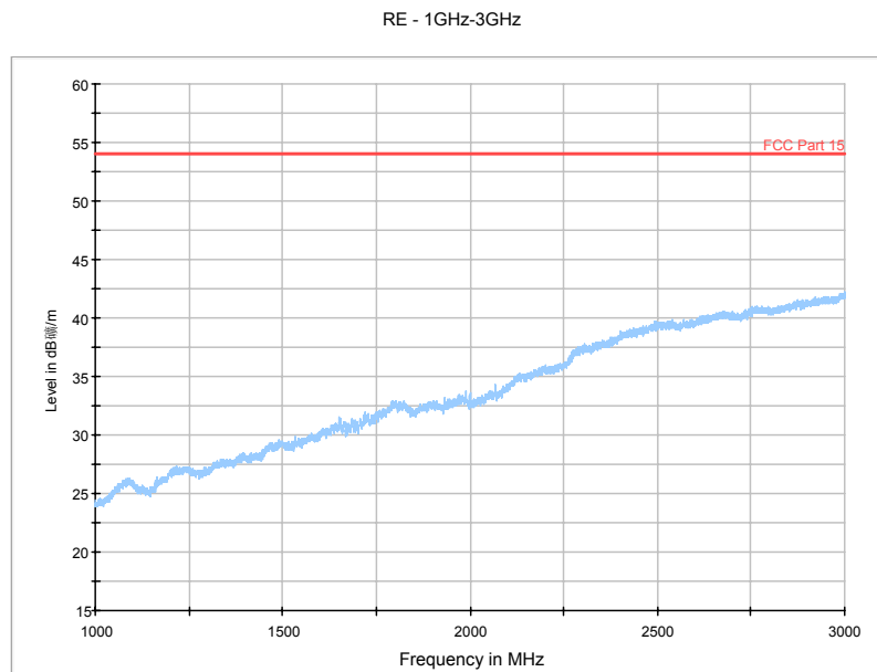
Fig. 83 Radiated Spurious Emission (802.11n-HT40, Ch159, 1 GHz-3 GHz)
