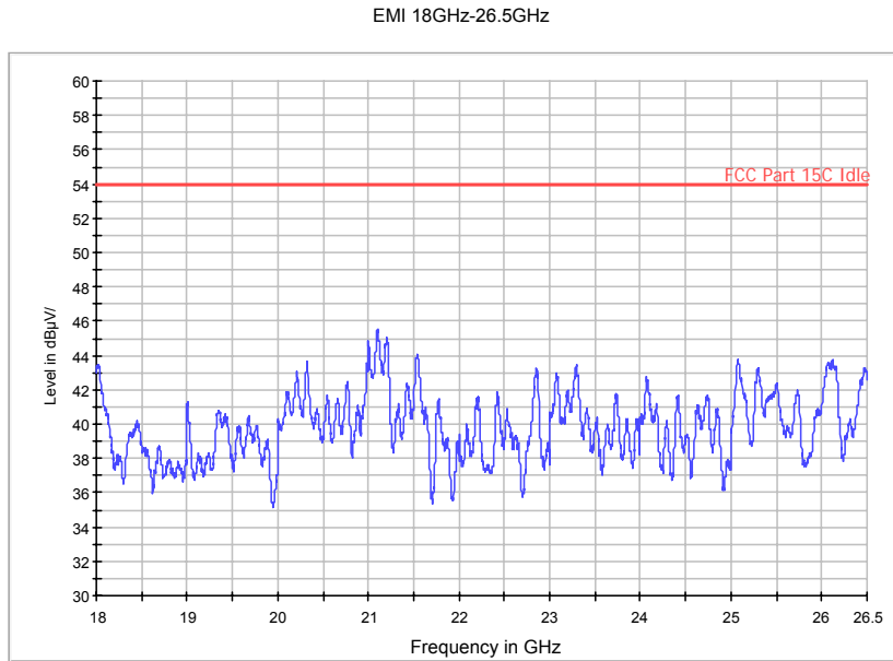
Fig. 69 Radiated Spurious Emission (802.11n-HT20, Ch157, 18 GHz-26.5 GHz)
