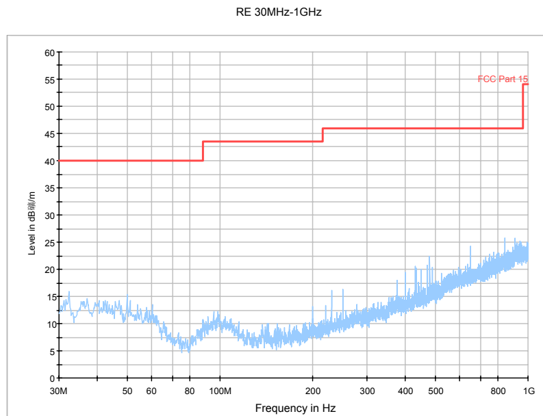
Fig. 65 Radiated Spurious Emission (802.11n-HT20, Ch157, 30 MHz-1 GHz)
