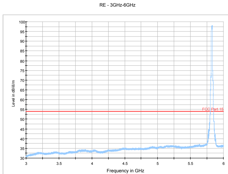
Fig. 55 Radiated Spurious Emission (802.11a, Ch165, 3 GHz-6 GHz)
