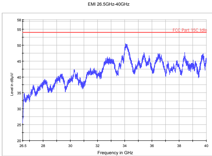
Fig. 58 Radiated Spurious Emission (802.11a, Ch165, 26.5 GHz-40 GHz)
