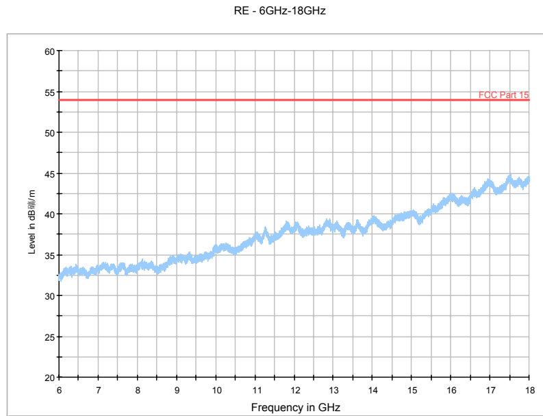
Fig. 56 Radiated Spurious Emission (802.11a, Ch165, 6 GHz-18 GHz)
