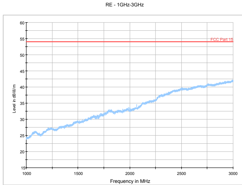
Fig. 60 Radiated Spurious Emission (802.11n-HT20, Ch149, 1 GHz-3 GHz)
