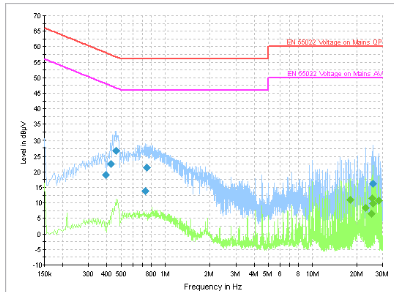
Fig. 89 AC Powerline Conducted Emission-Idle
