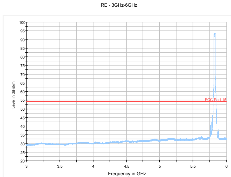
Fig. 73 Radiated Spurious Emission (802.11n-HT20, Ch165, 3 GHz-6 GHz)
