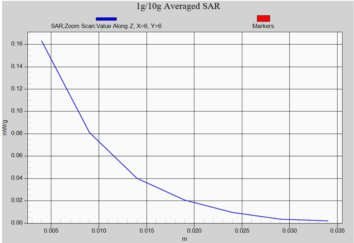
Fig. 21-1 Z-Scan at power reference point (2450 MHz CH11)
