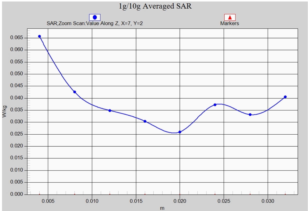
Fig. 24-1 Z-Scan at power reference point (5GHz CH116)
