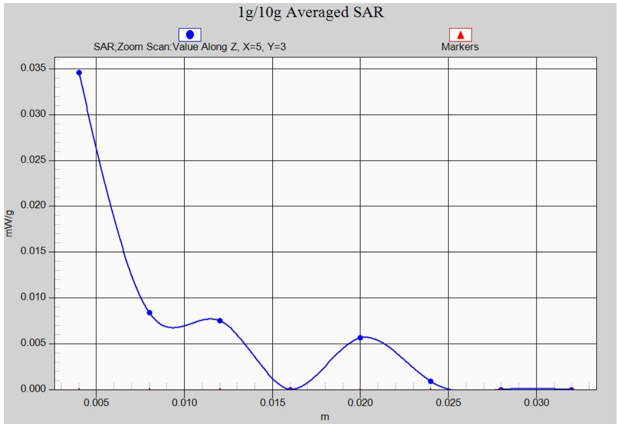
Fig. 22-1 Z-Scan at power reference point (5GHz CH153)
