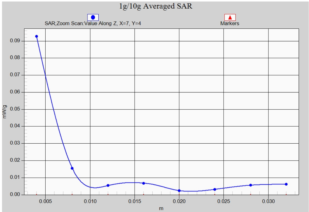
Fig. 23-1 Z-Scan at power reference point (5GHz CH153)
