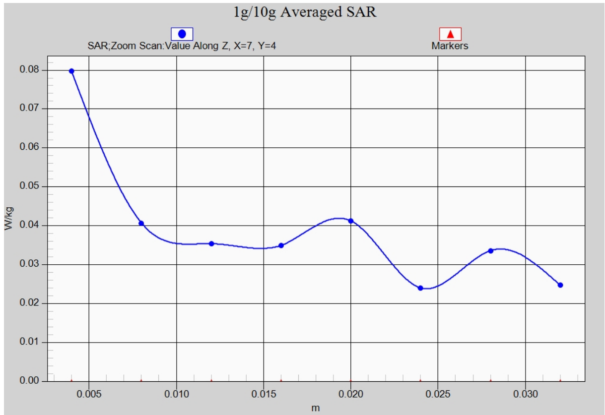
Fig. 25-1 Z-Scan at power reference point (5GHz CH116)
