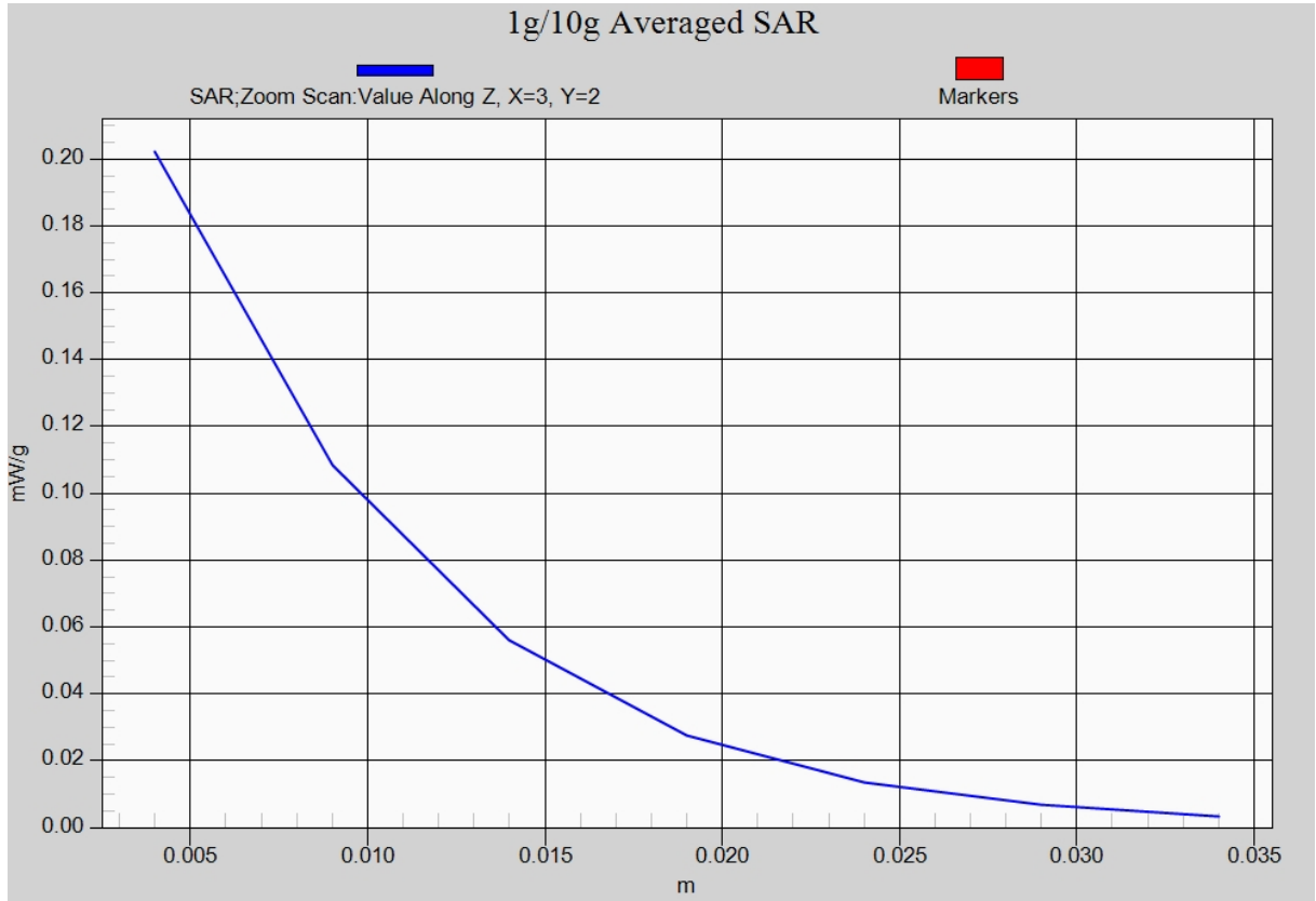
Fig. 20-1 Z-Scan at power reference point (2450 MHz CH6)
