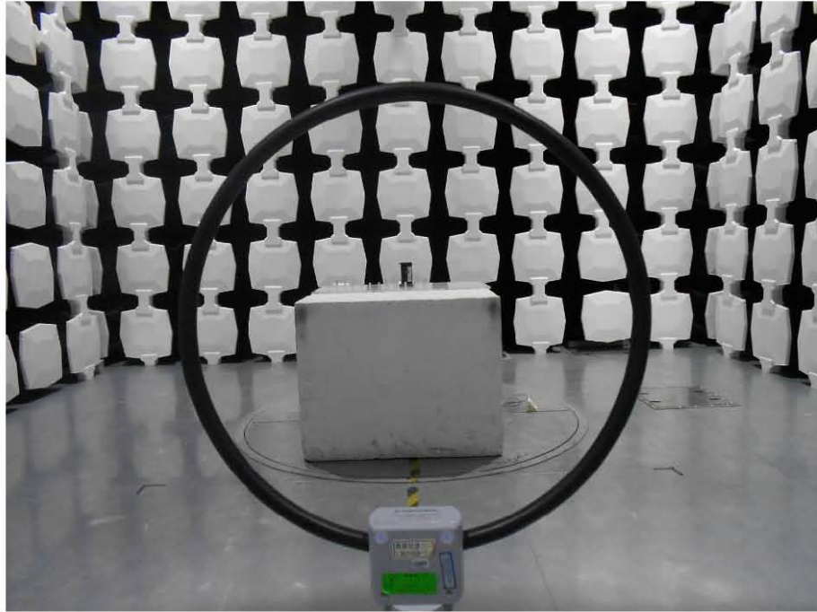
Picture C-1: Field Strength Measurements (Below 30MHz)
