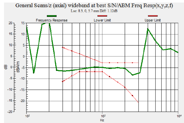
Fig 7.2 GSM850 Ch661
