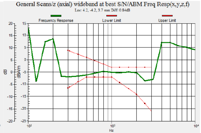
Fig 7.2 GSM1900 Ch661
