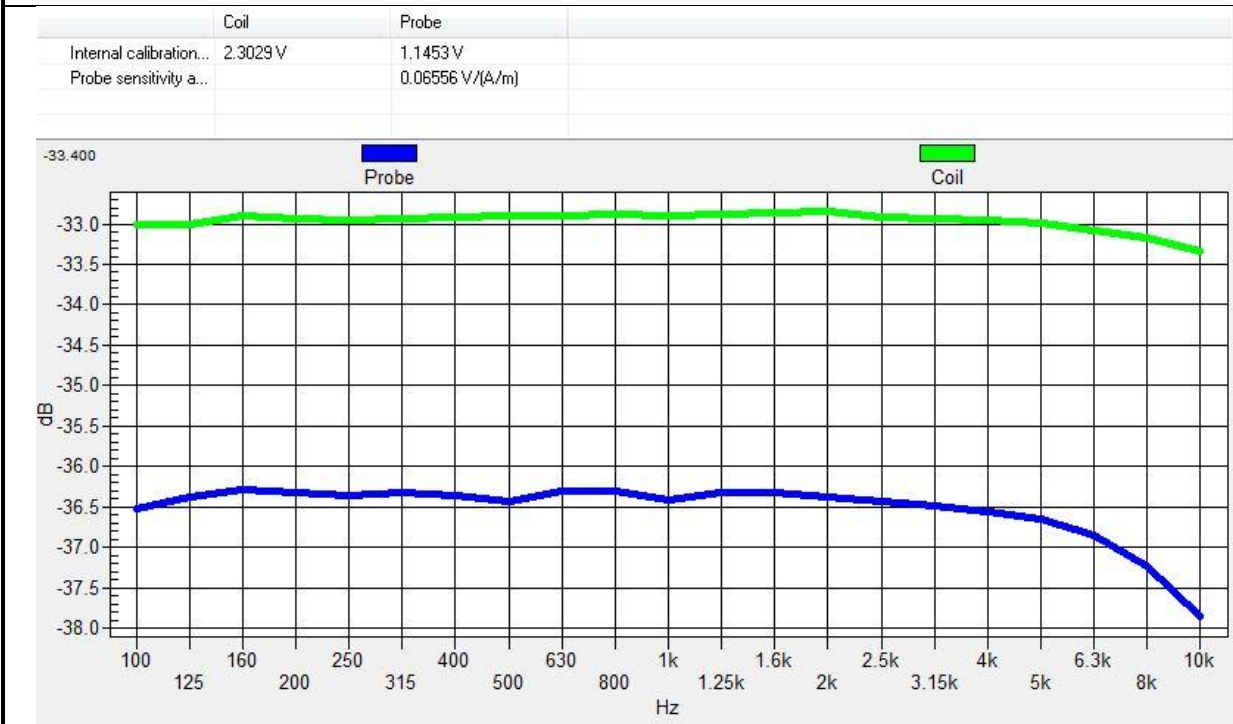
Fig. 5.5 The frequency response and sensitivity of AM1D probe
