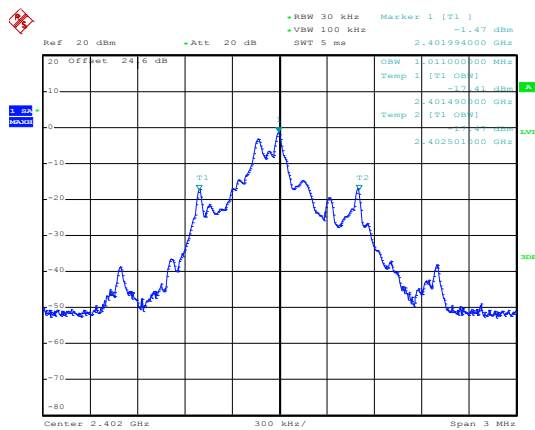
99% Bandwidth Plot on 2402MHz
