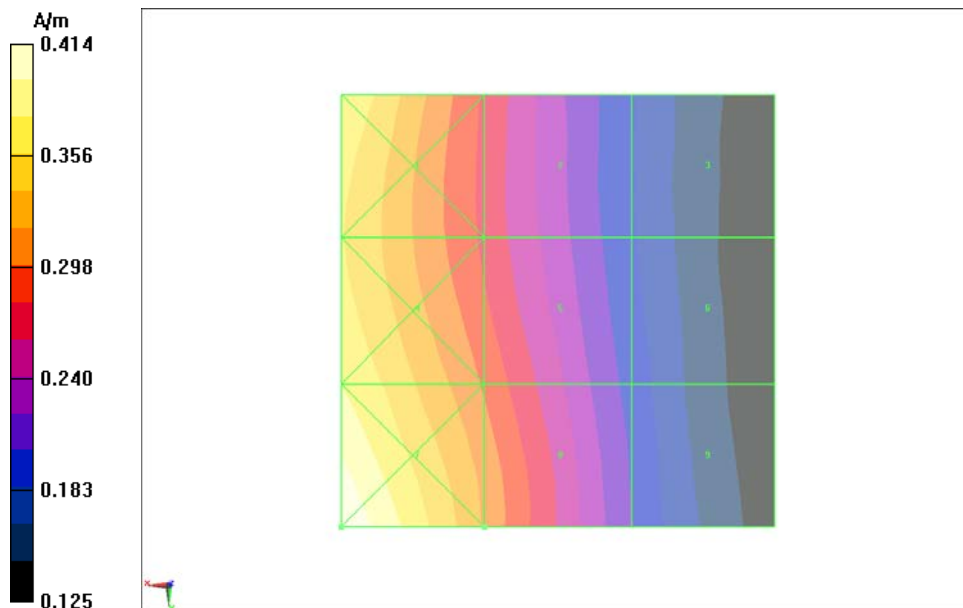
Fig B.17 HAC RF H-Field GSM 850 Middle
