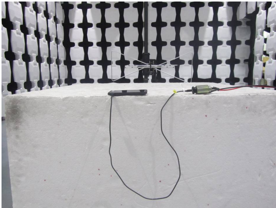
Radiated emission GPS
