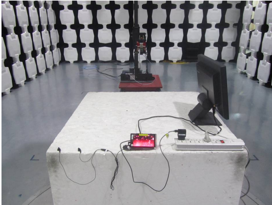
Radiated emission MHL
