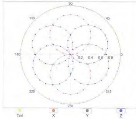
f=600 MHz,TEM
