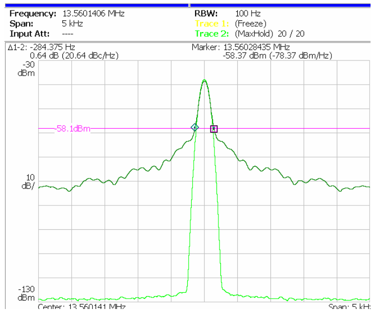
Figure A-5: Test result of EUT1 at test set. NFC03
