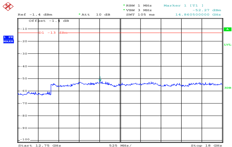
Plot 3: Channel 661 (12.75 GHz - 18 GHz)
