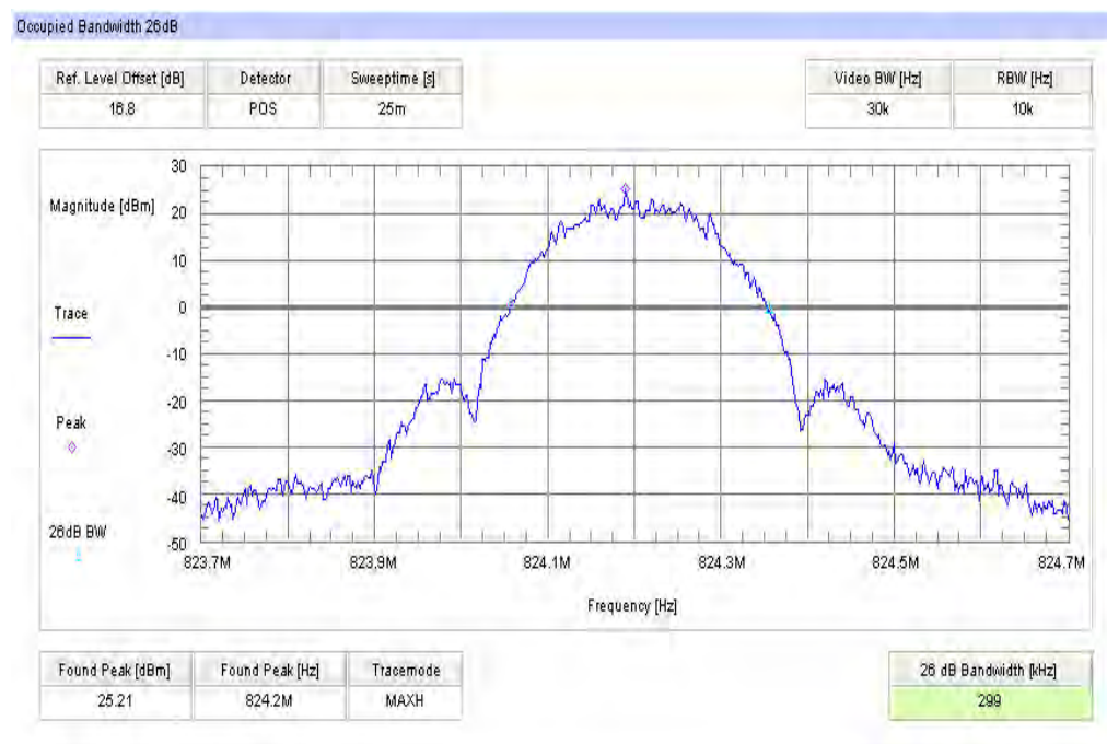
Plot 8: Channel 128 (-26 dBc BW) - 8-PSK
