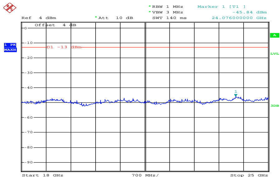
Plot 4: Channel 661 (18 GHz - 25 GHz)
