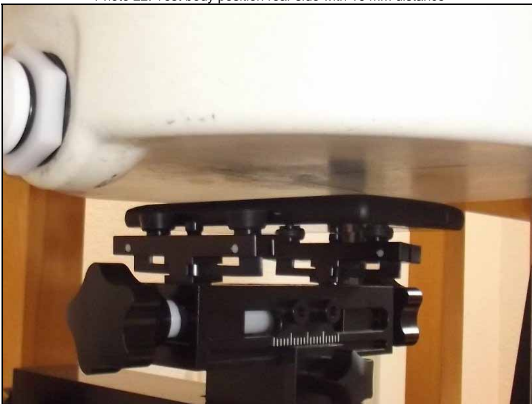
Photo 22: Test body position rear side with 10 mm distance
