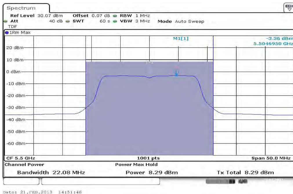
Plot 5: 5500 MHz
