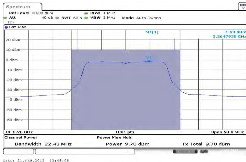
Plot 3: 5260 MHz
