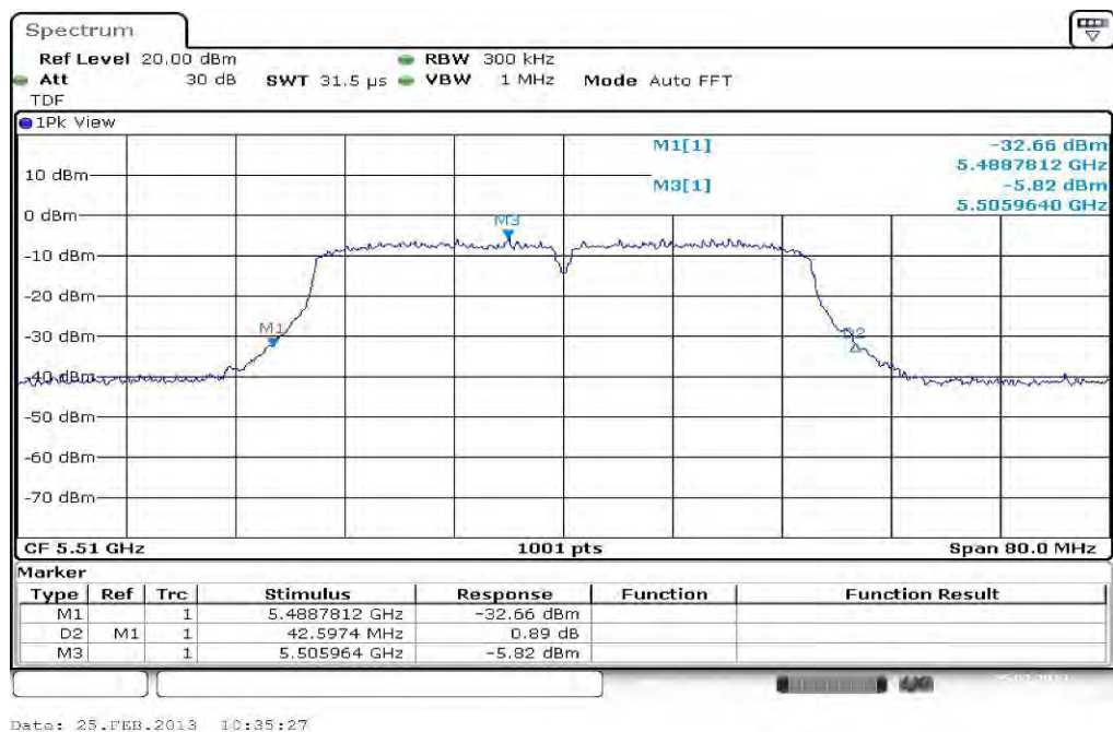
Plot 5: 5510 MHz
