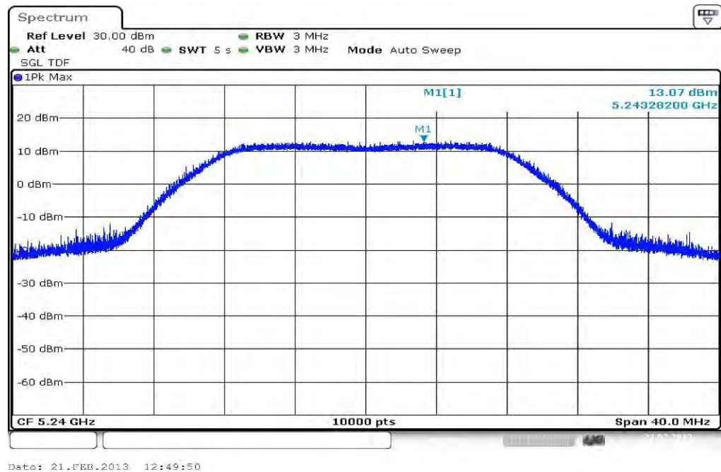
Plot 2: OFDM / a – mode, 5240 MHz
