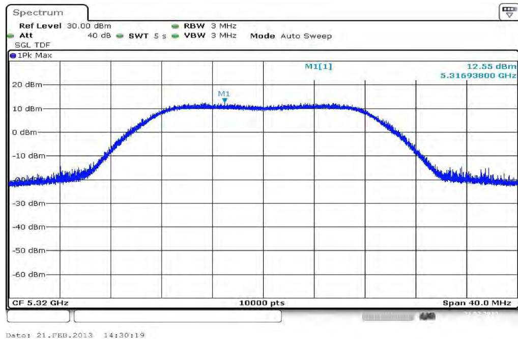
Plot 4: OFDM / a – mode, 5320 MHz
