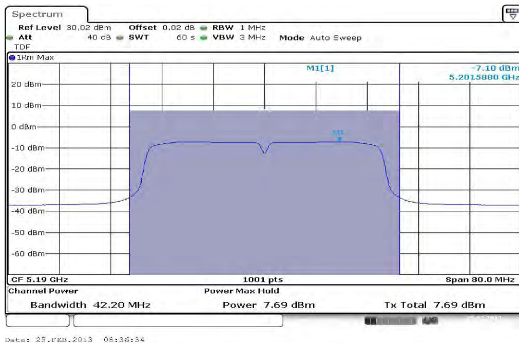
Plot 1: 5190 MHz
