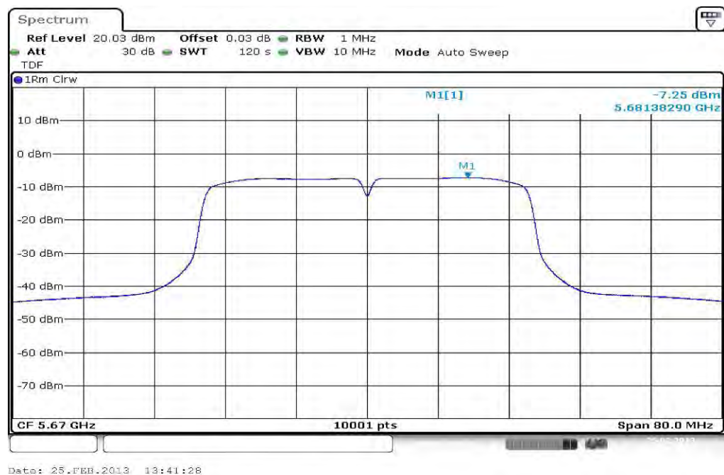
Plot 7: 5670 MHz
