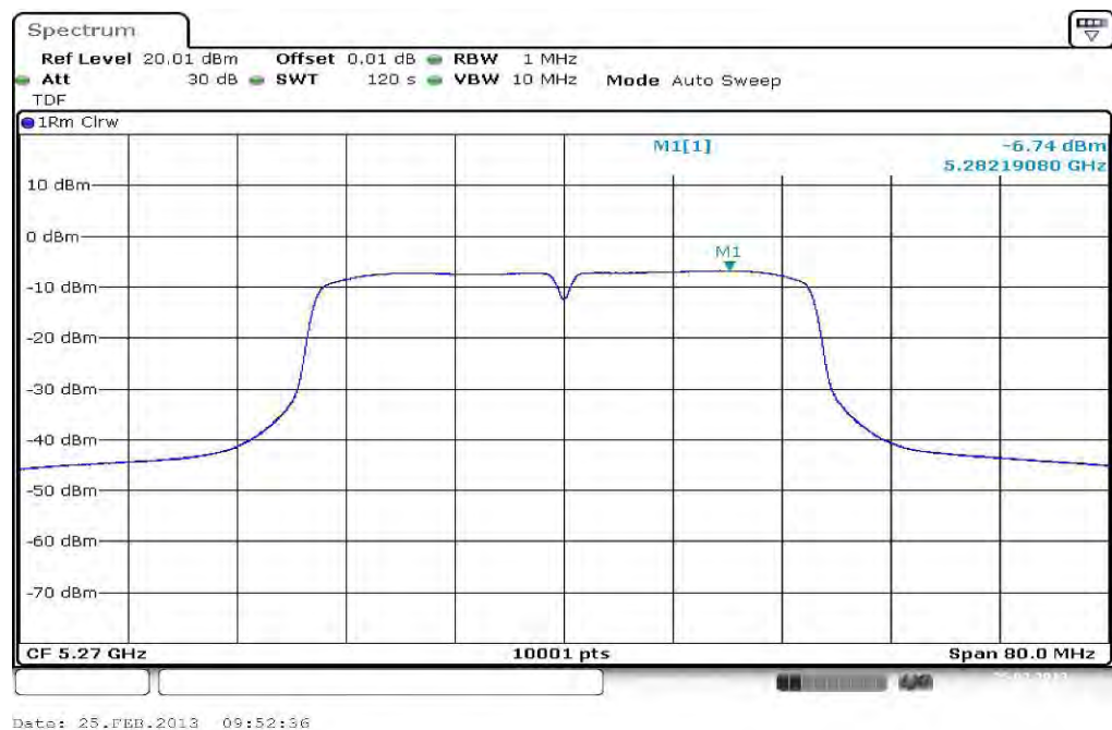
Plot 3: 5270 MHz
