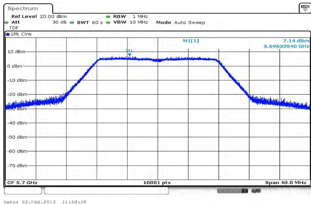
Plot 7: 5700 MHz
