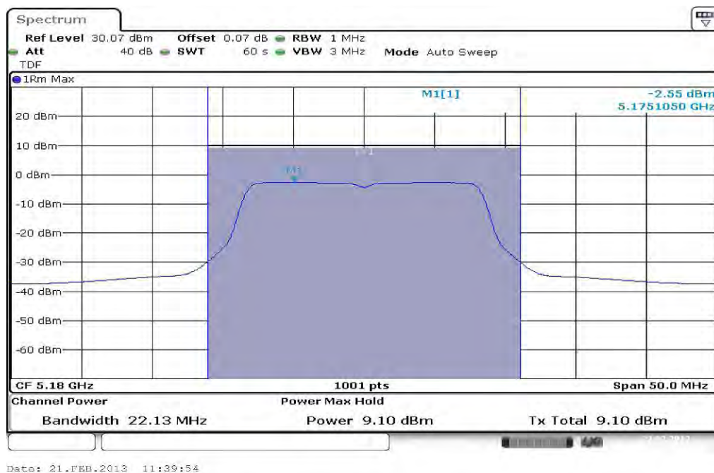
Plot 1: 5180 MHz
