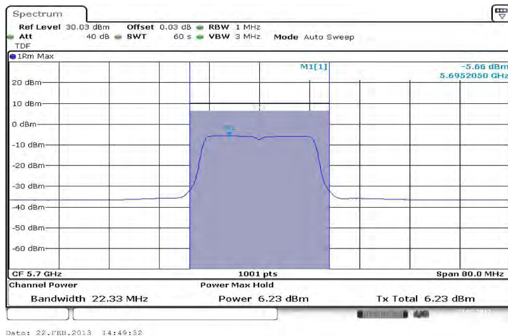
Plot 7: 5700 MHz
