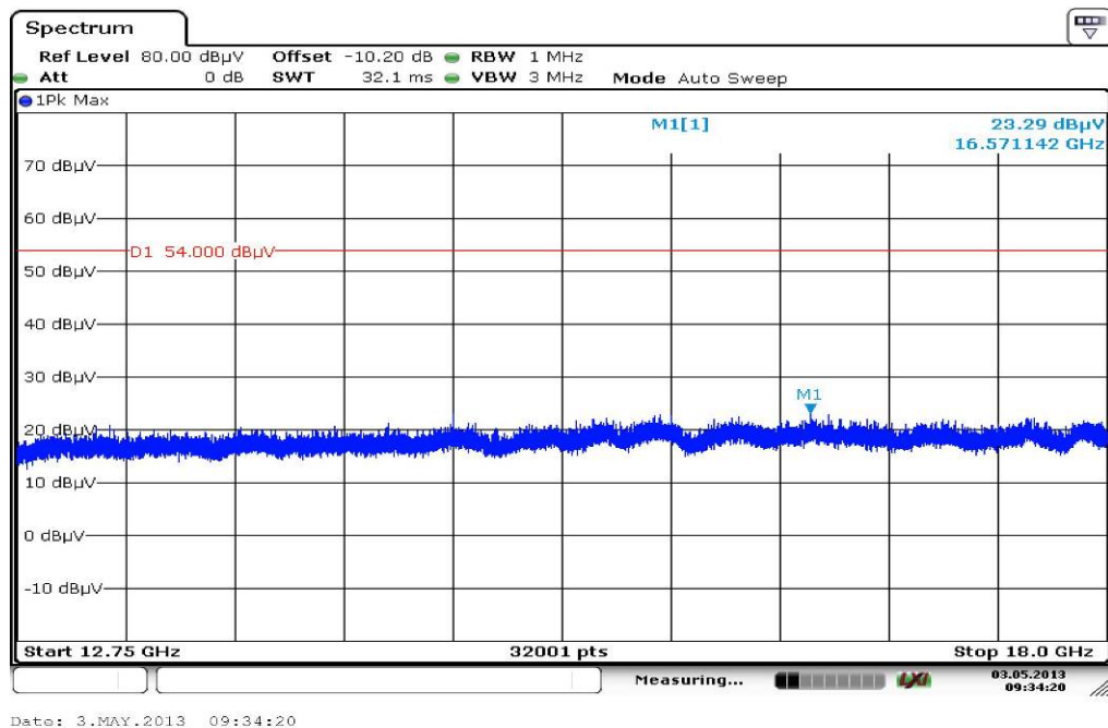
Plot 4: Receiver mode 12.75 GHz to 18 GHz
