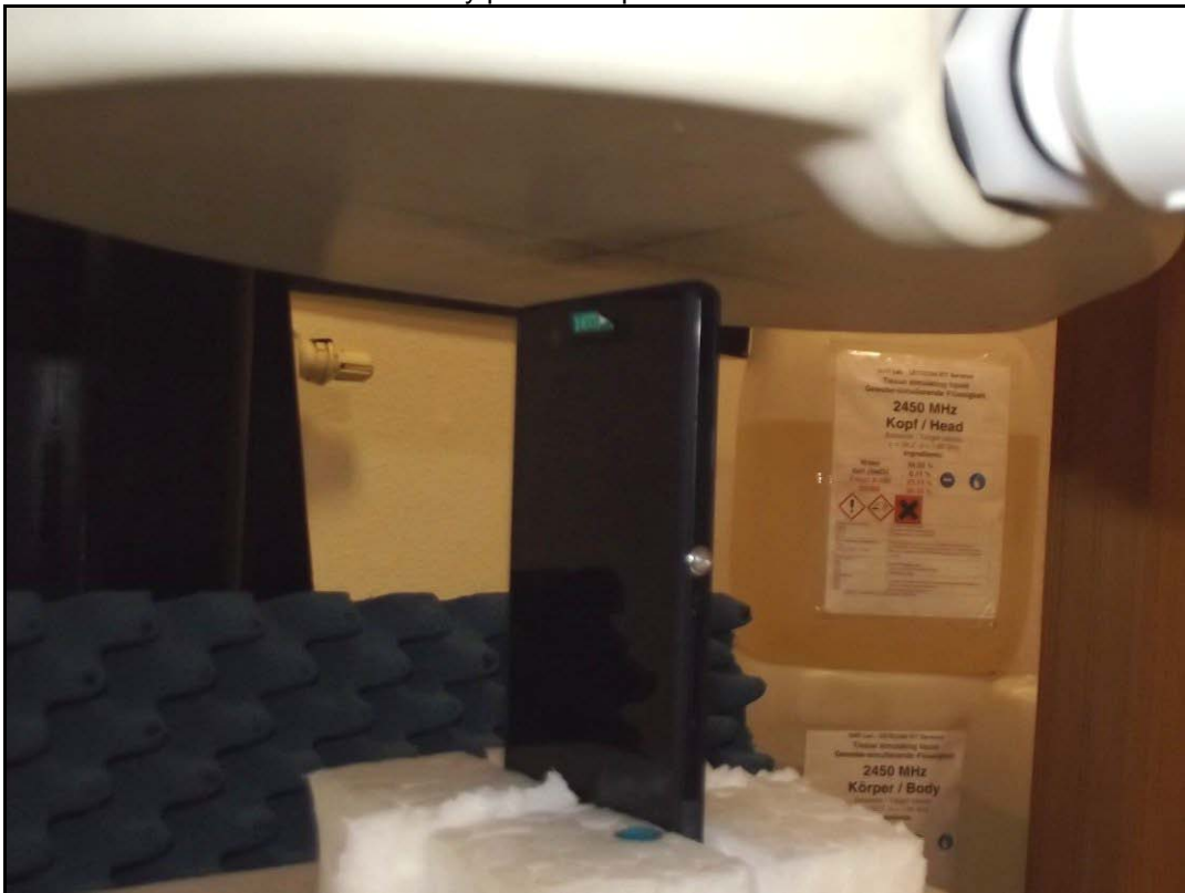
Photo 22: Test body position top side with 10 mm distance
