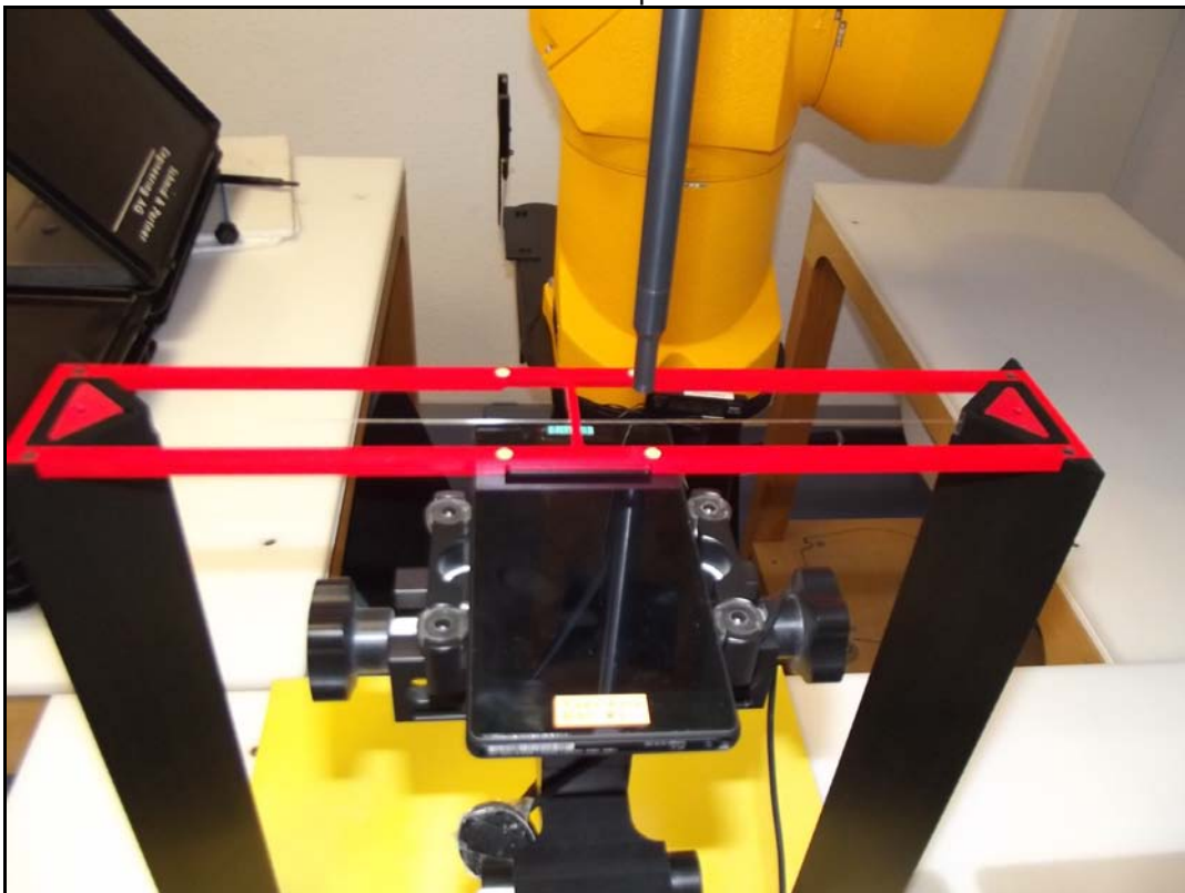
Photo 6: Test position
