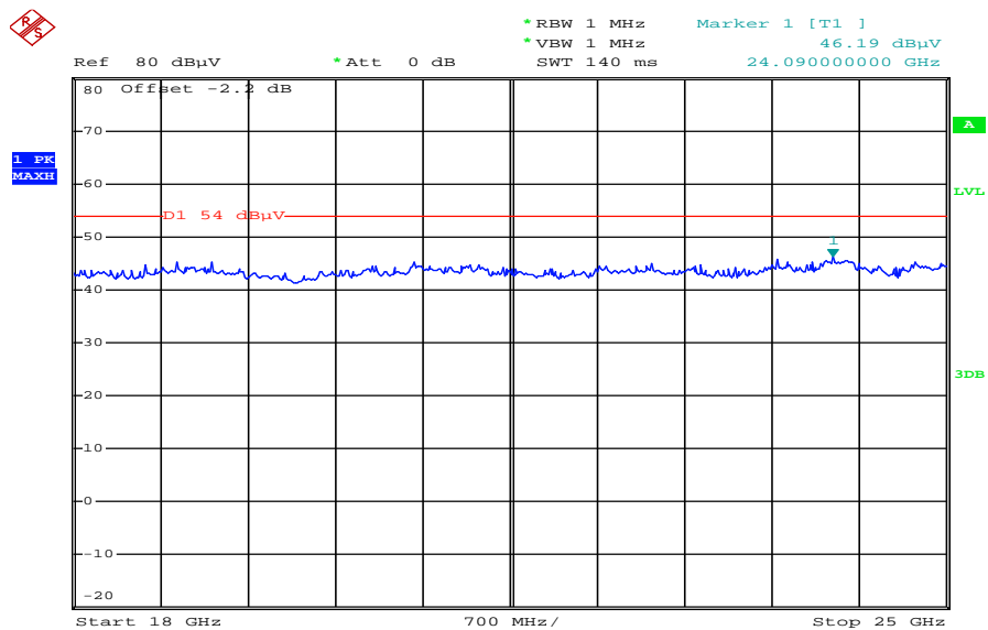
Plot 4: 18 GHz to 25 GHz, RX mode, vertical & horizontal polarization
