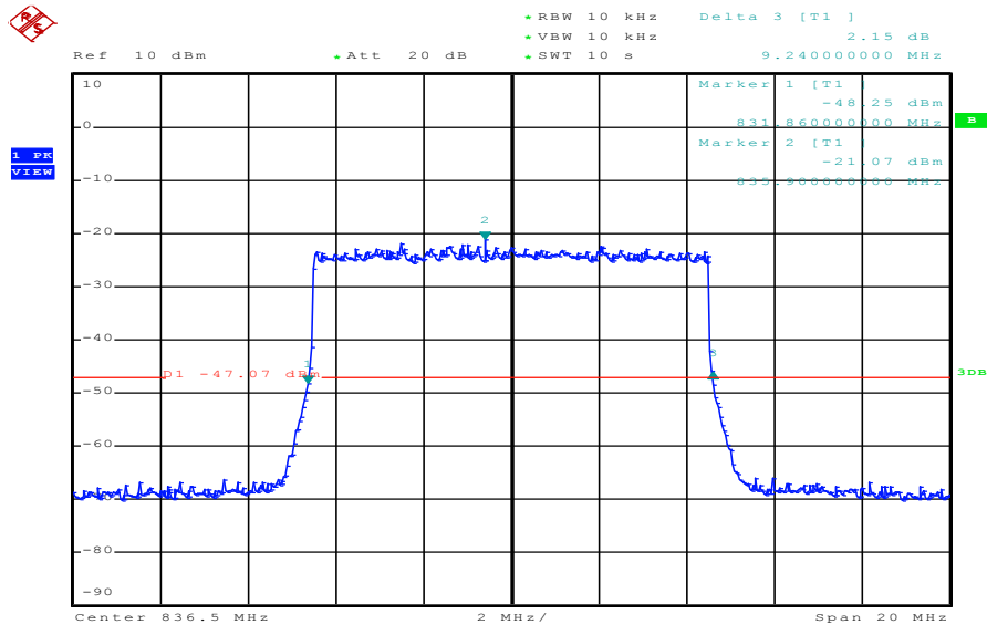
Plot 8: 10 MHz (-26 dBc BW)
