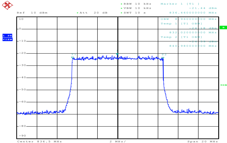
Plot 7: 10 MHz (99% - OBW)
