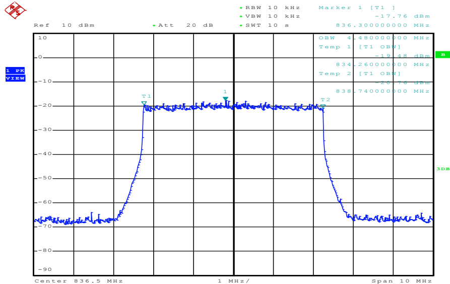
Plot 5: 5 MHz (99% - OBW)
