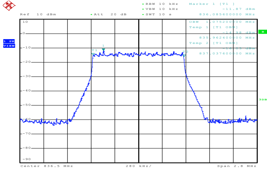
Plot 1: 1.4 MHz (99% - OBW)
