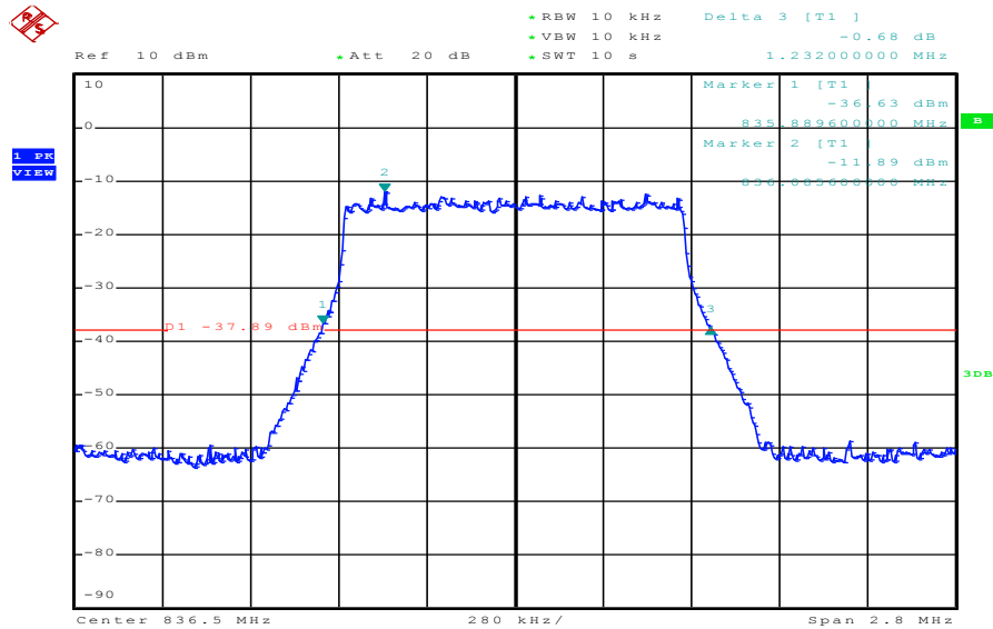
Plot 2: 1.4 MHz (-26 dBc BW)
