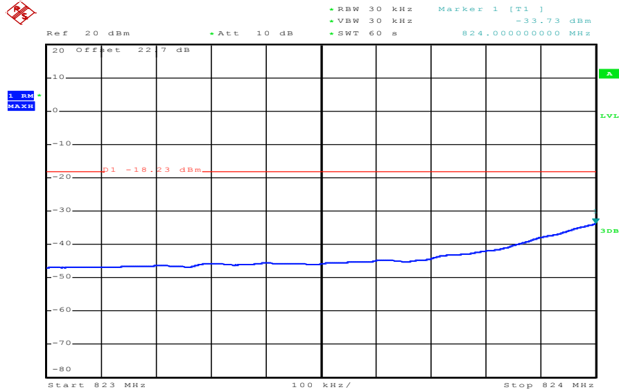
Plot 3: Lowest channel – 16-QAM
