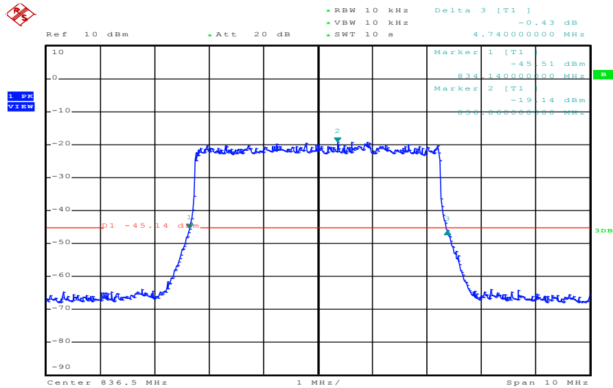
Plot 6: 5 MHz (-26 dBc BW)
