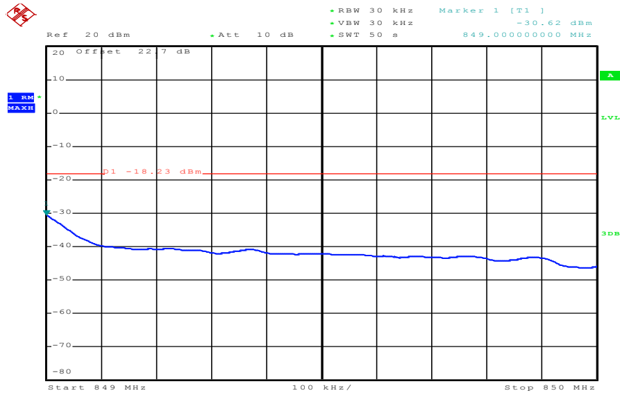
Plot 4: Highest channel – 16-QAM
