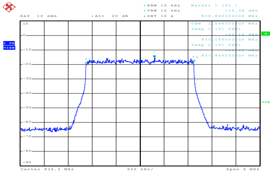
Plot 3: 3 MHz (99% - OBW)
