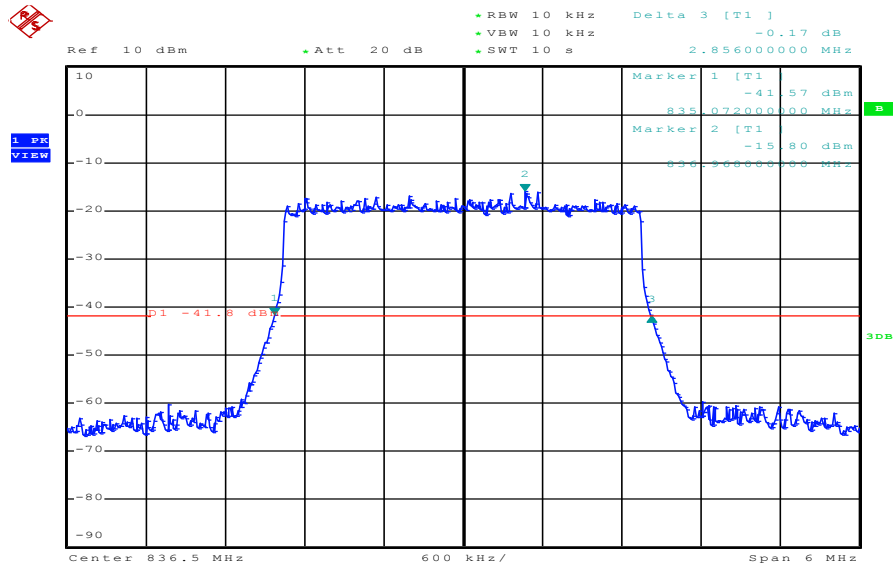
Plot 4: 3 MHz (-26 dBc BW)
