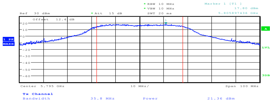
Plot 2: TX mode, highest channel
