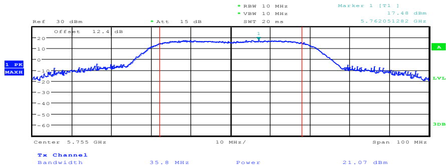
Plot 1: TX mode, lowest channel
