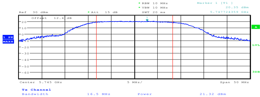
Plot 2: TX mode, middle channel
