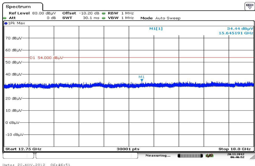
Plot 3: 12.75 GHz to 18 GHz, RX / idle – mode, vertical & horizontal polarization
