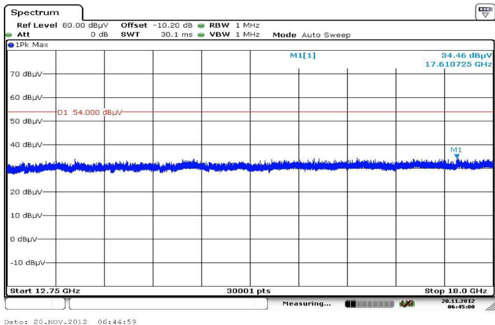
Plot 3: 12.75 GHz to 18 GHz, lowest channel, vertical & horizontal polarization
