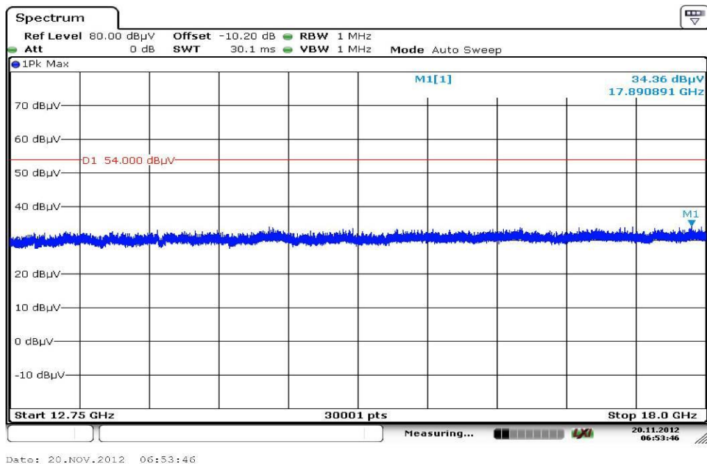
Plot 7: 12.75 GHz to 18 GHz, mid channel, vertical & horizontal polarization
