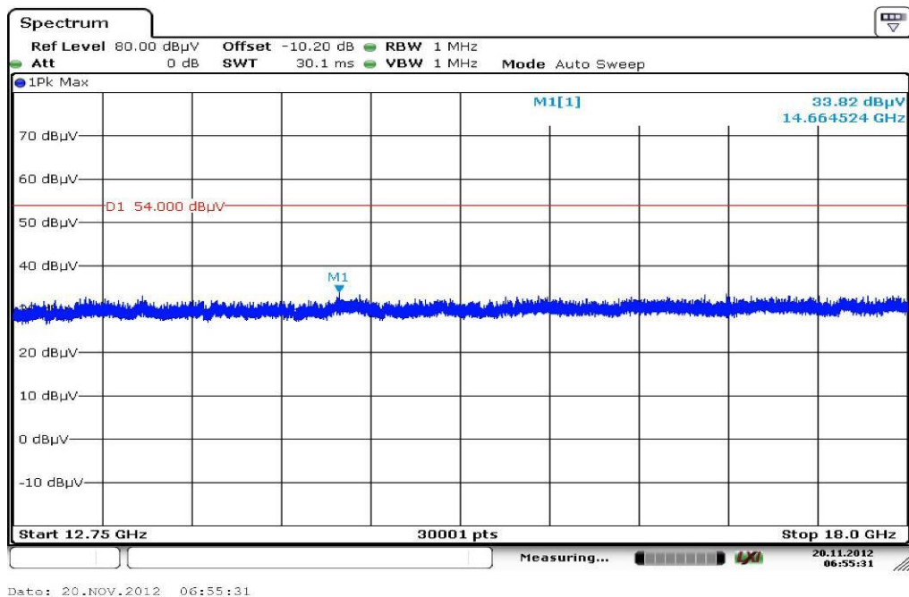
Plot 11: 12.75 GHz to 18 GHz, highest channel, vertical & horizontal polarization
