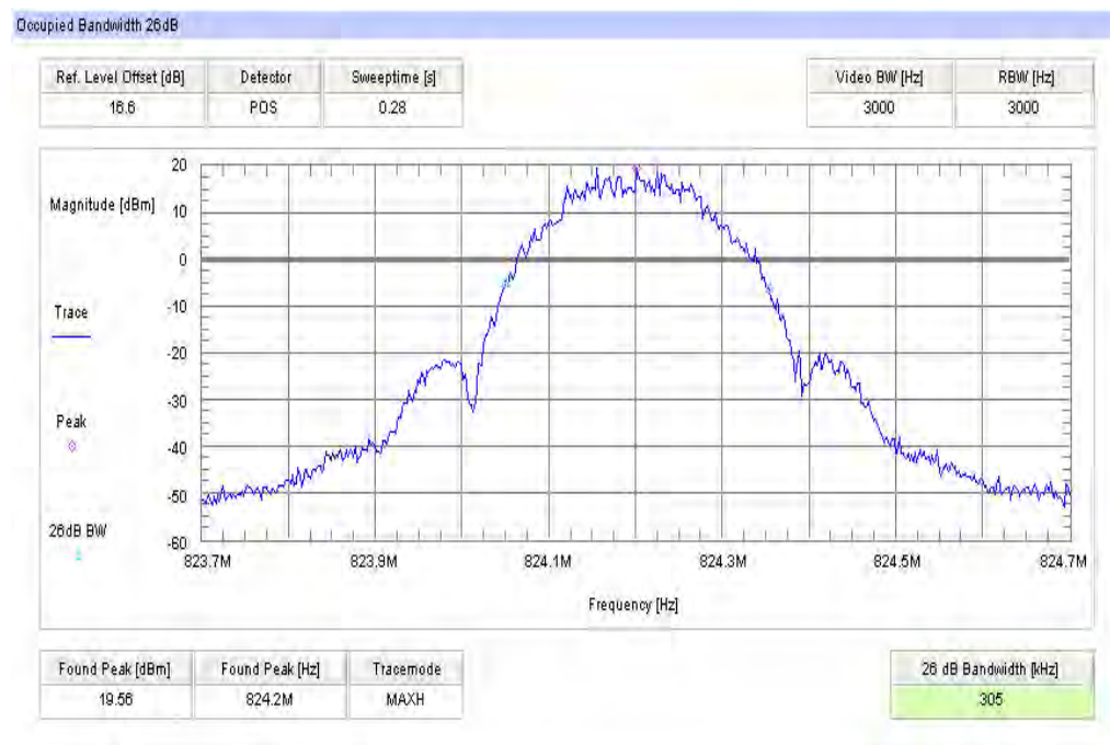
Plot 8: Channel 128 (-26 dBc BW) - EDGE
