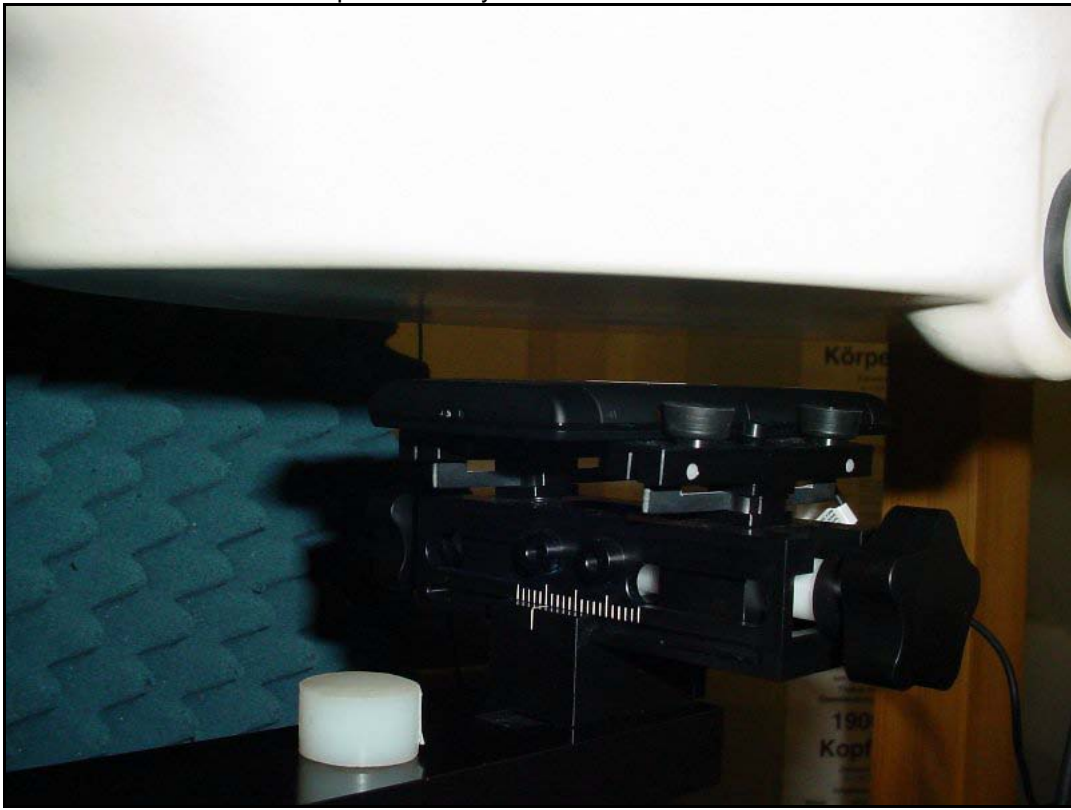
Photo 18: Test position body (hotspot) front side with 10 mm distance
