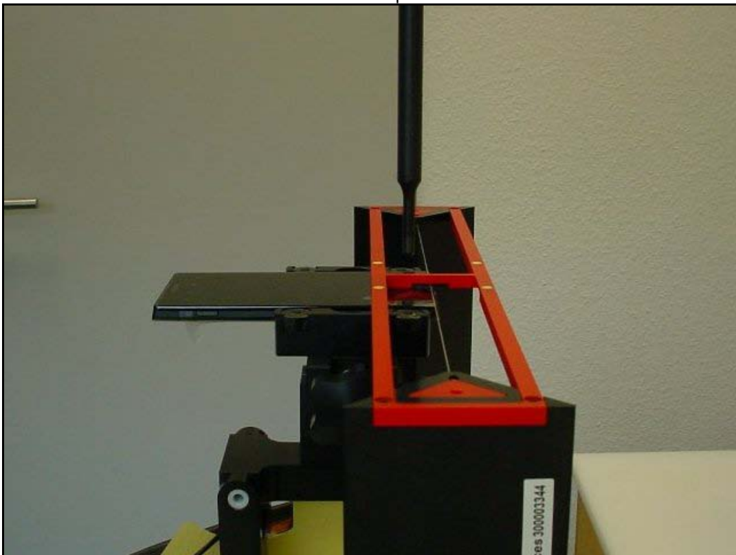
Photo 2: Test position
