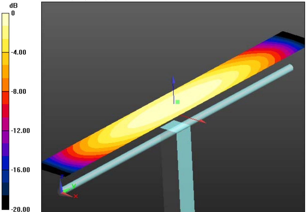
0 dB = 0.4523 A/m = -6.89 dB A/m
