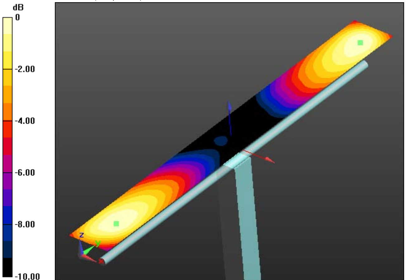
0 dB = 164.0 V/m = 44.30 dB V/m
