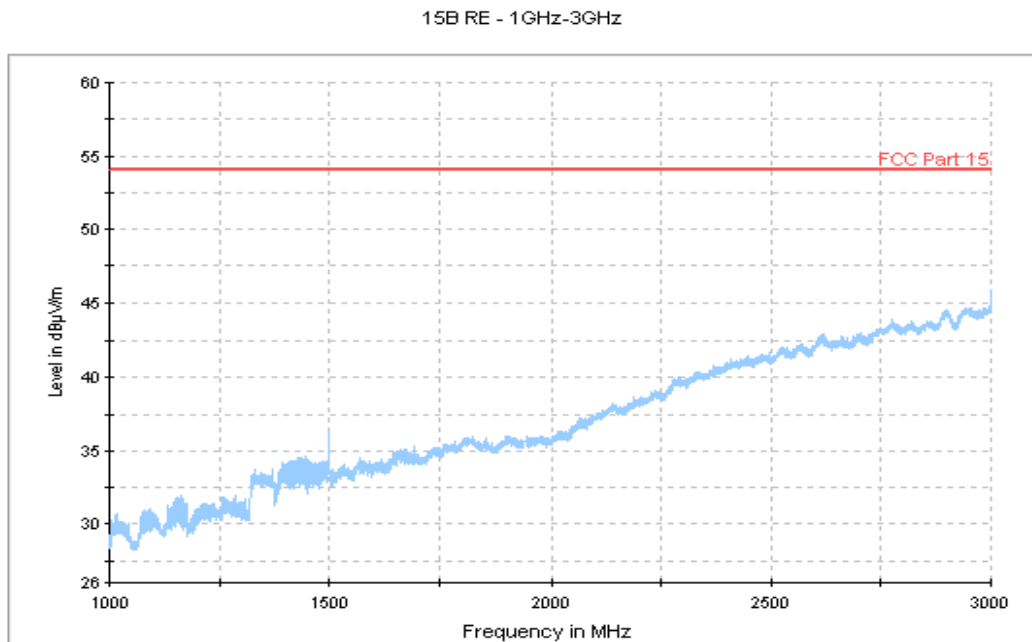
Figure B.2 Radiated Emission from 1GHz to 3GHz
